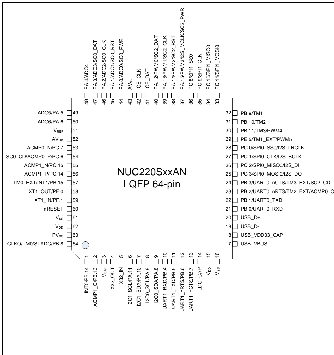
Figure 4-6 NuMicro™ NUC220SxxAN LQFP 64-pin Diagram
