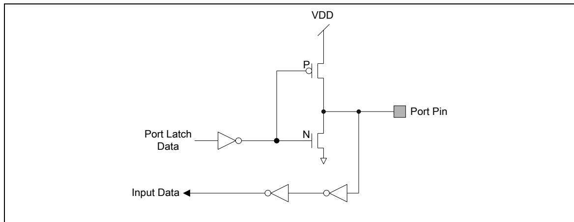
Figure 6-16 Push-Pull Output
