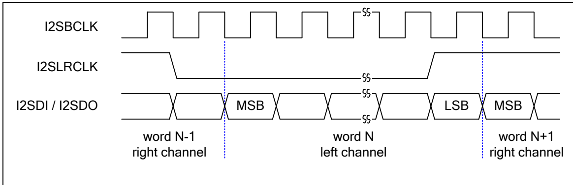
Figure 6-114 I 2 S Data Format Timing Diagram
