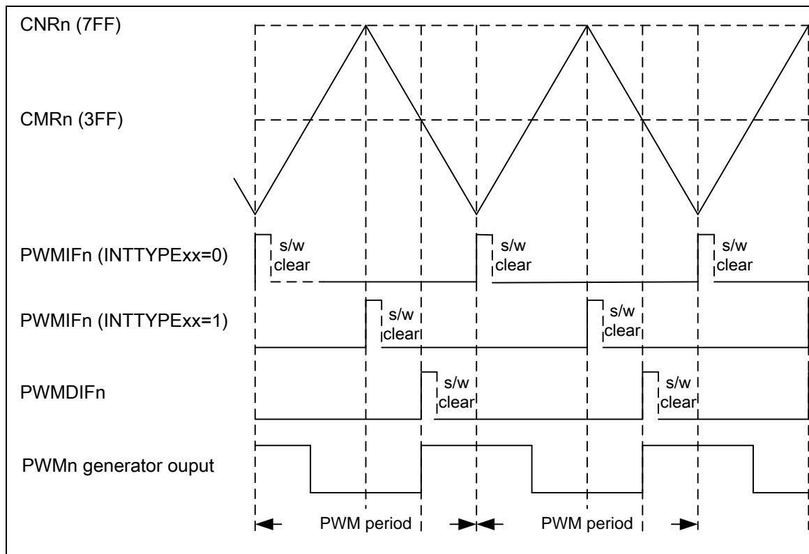
Figure 6-36 PWM Center-aligned Interrupt Generate Timing Waveform
