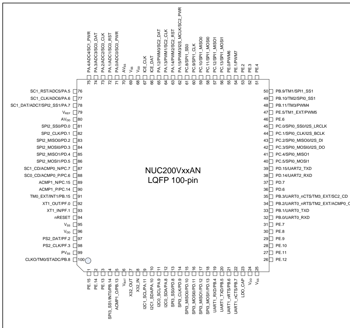
Figure 4-2 NuMicro™ NUC200VxxAN LQFP 100-pin Diagram
