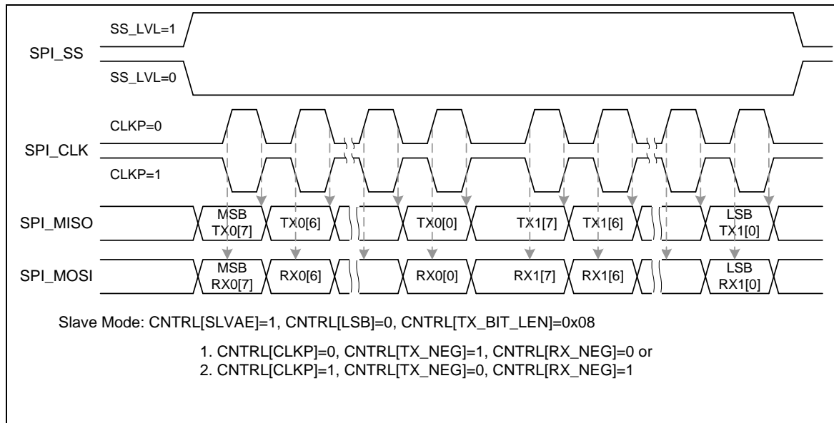
Figure 6-110 SPI Timing in Slave Mode
