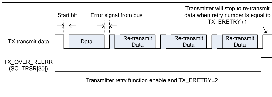
Figure 6-71 SC Transmitter Retry Number and Retry Over Flag
