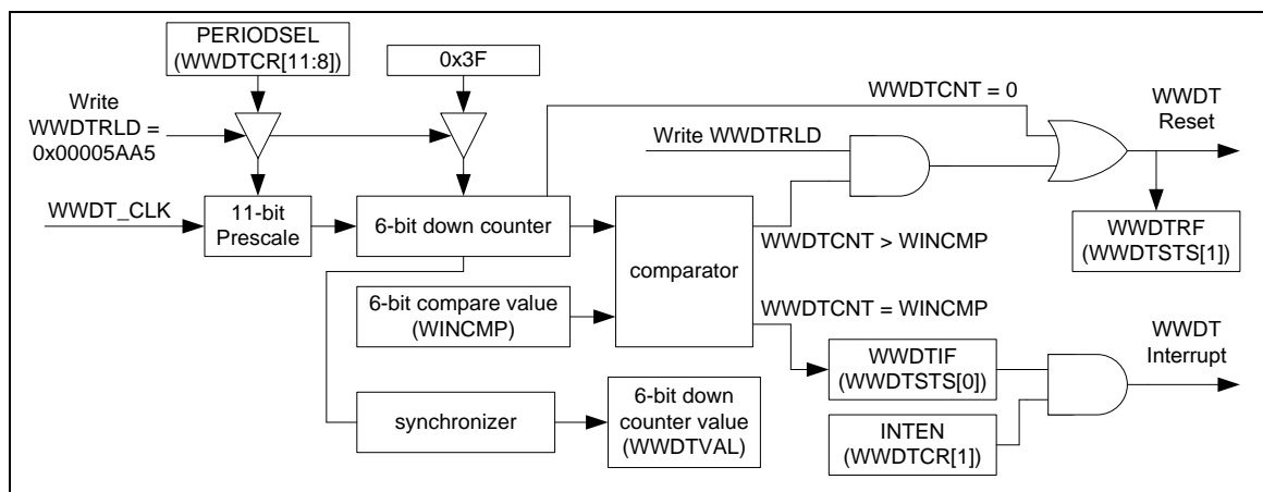
Figure 6-48 Window Watchdog Timer Block Diagram
