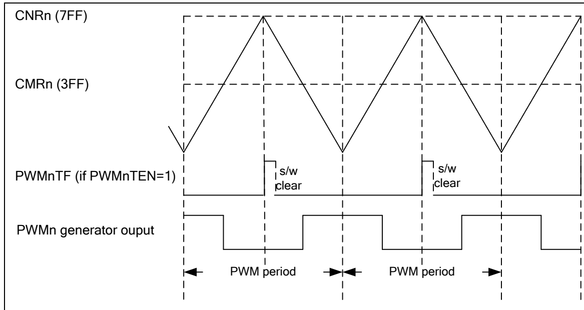
Figure 6-40 PWM trigger ADC to conversion in Center-aligned type Timing Waveform
