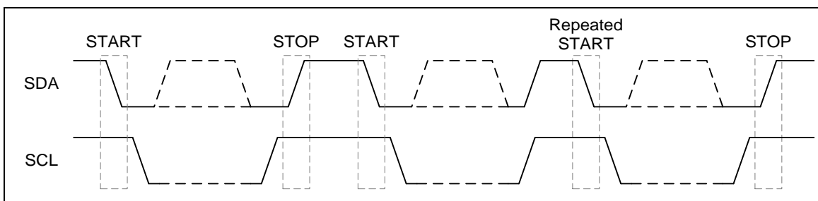
Figure 6-83 START and STOP Conditions
