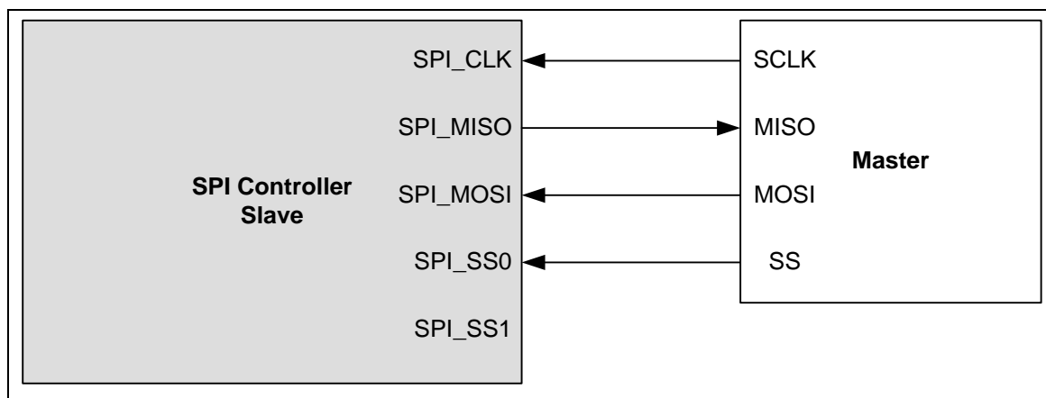
Figure 6-99 SPI Slave Mode Application Block Diagram
