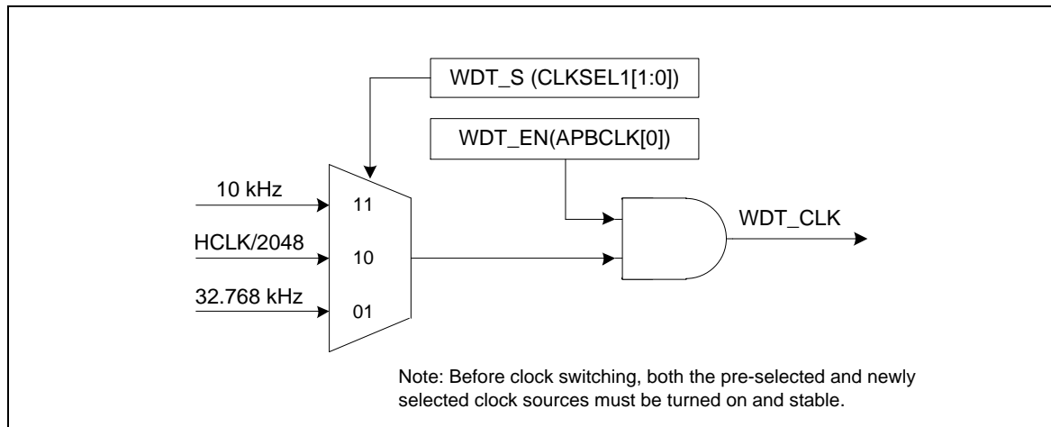
Figure 6-44 Watchdog Timer Clock Control
