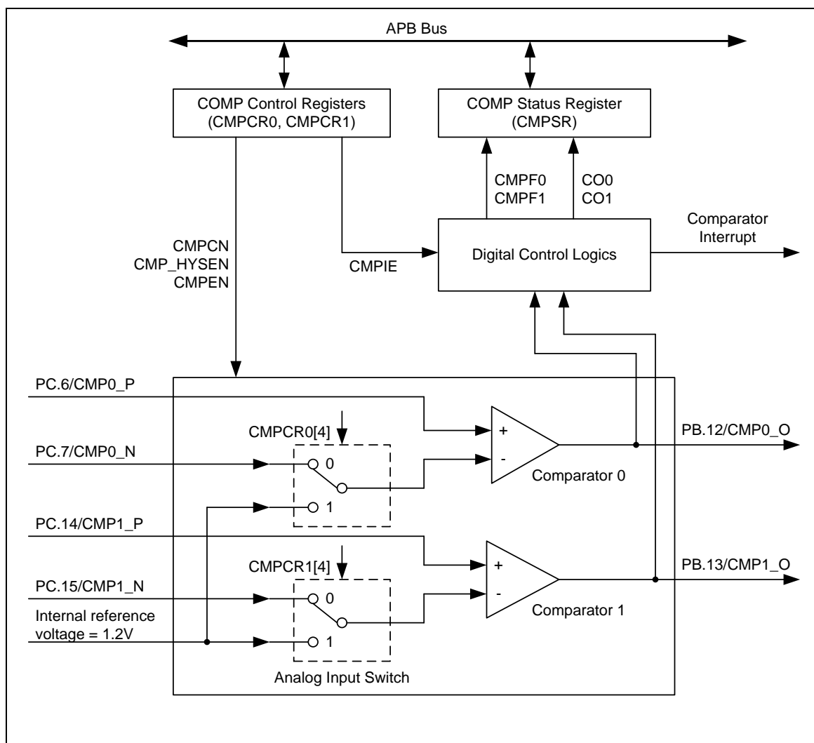
Figure 6-133 Analog Comparator Block Diagram
