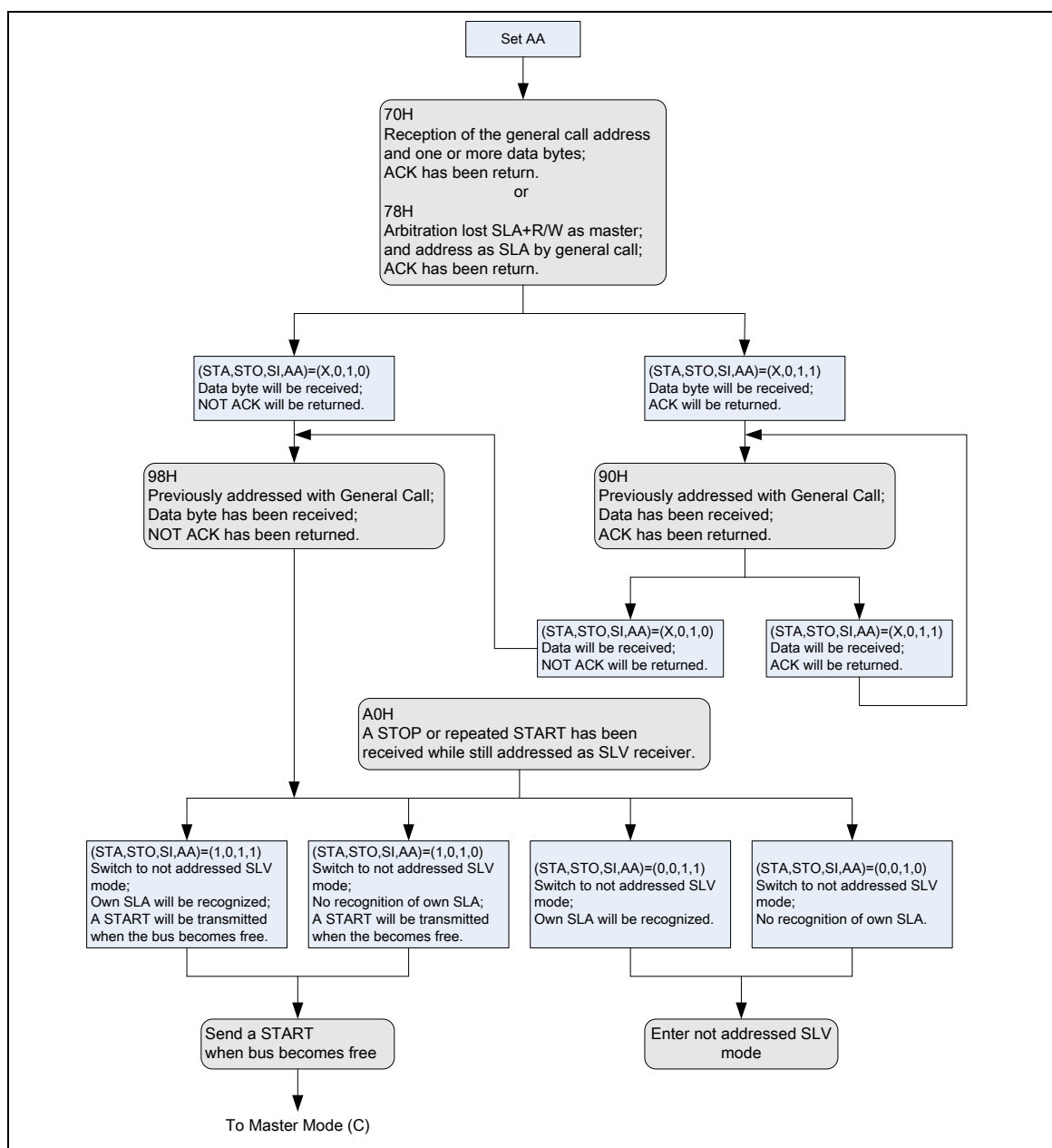
Figure 6-93 GC Mode
