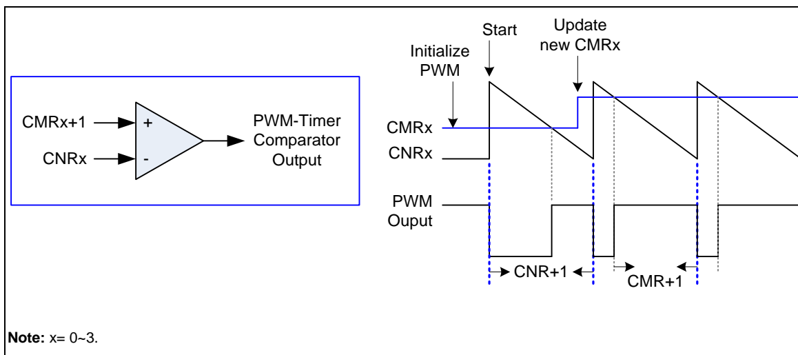
Figure 6-32 Legend of Internal Comparator Output of PWM-Timer
