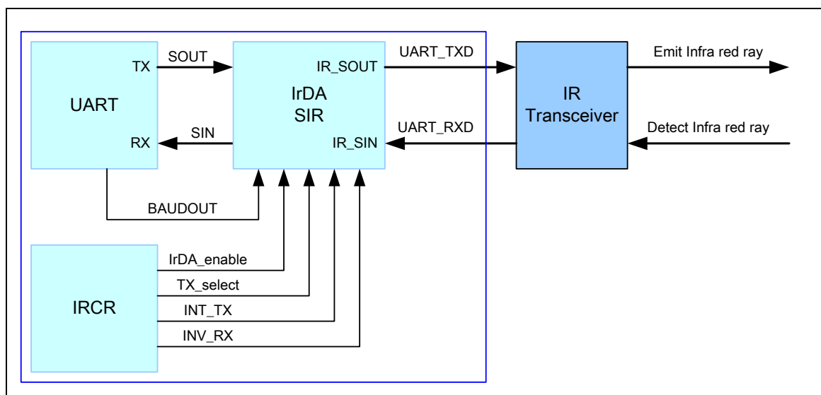
Figure 6-54 IrDA Block Diagram
