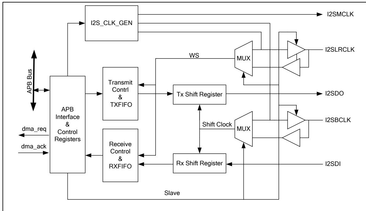
Figure 6-112 I²S Controller Block Diagram
