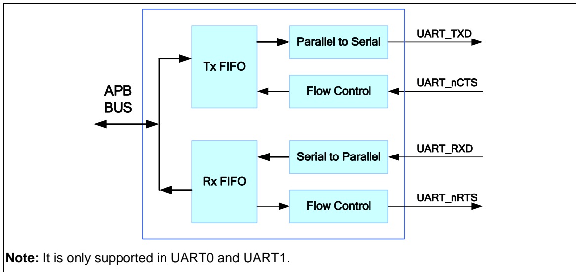
Figure 6-53 Auto Flow Control Block Diagram
