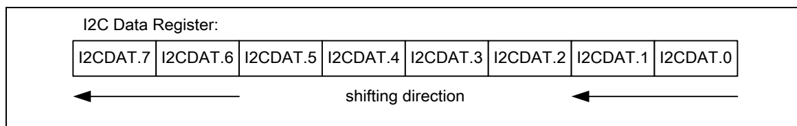
Figure 6-86 I 2 C Data Shifting Direction
