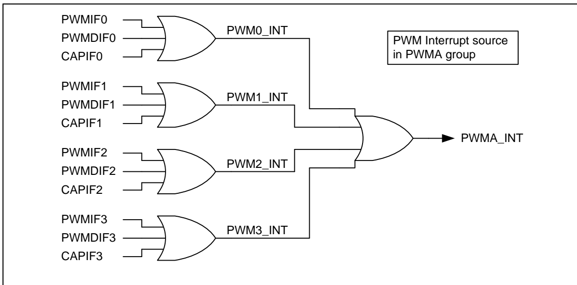
Figure 6-42 PWM Group A PWM-Timer Interrupt Architecture Diagram
