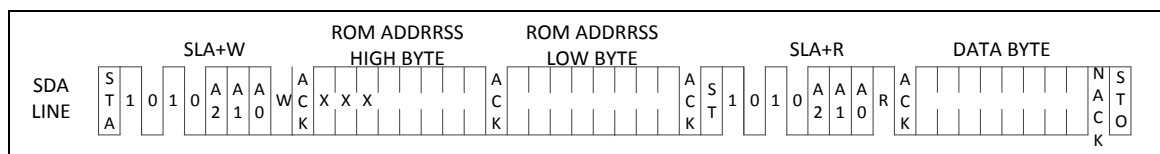
Figure 6-94 Random Read of EEPROM
