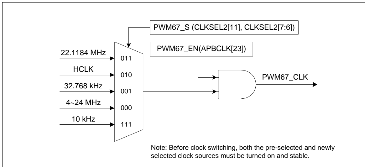
Figure 6-30 PWM Generator 6 Clock Source Control
