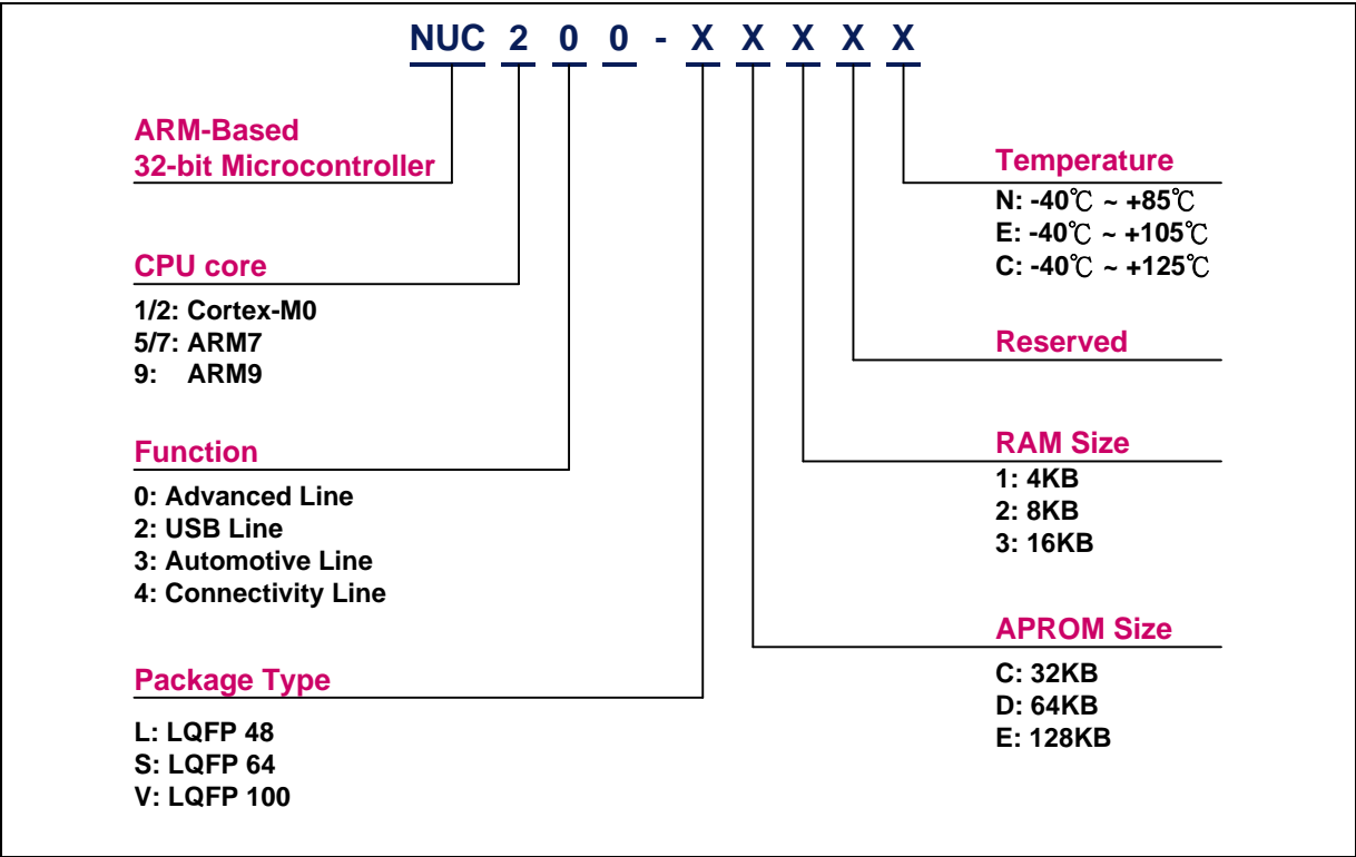
Figure 4-1 NuMicro™ NUC200 Series Selection Code
