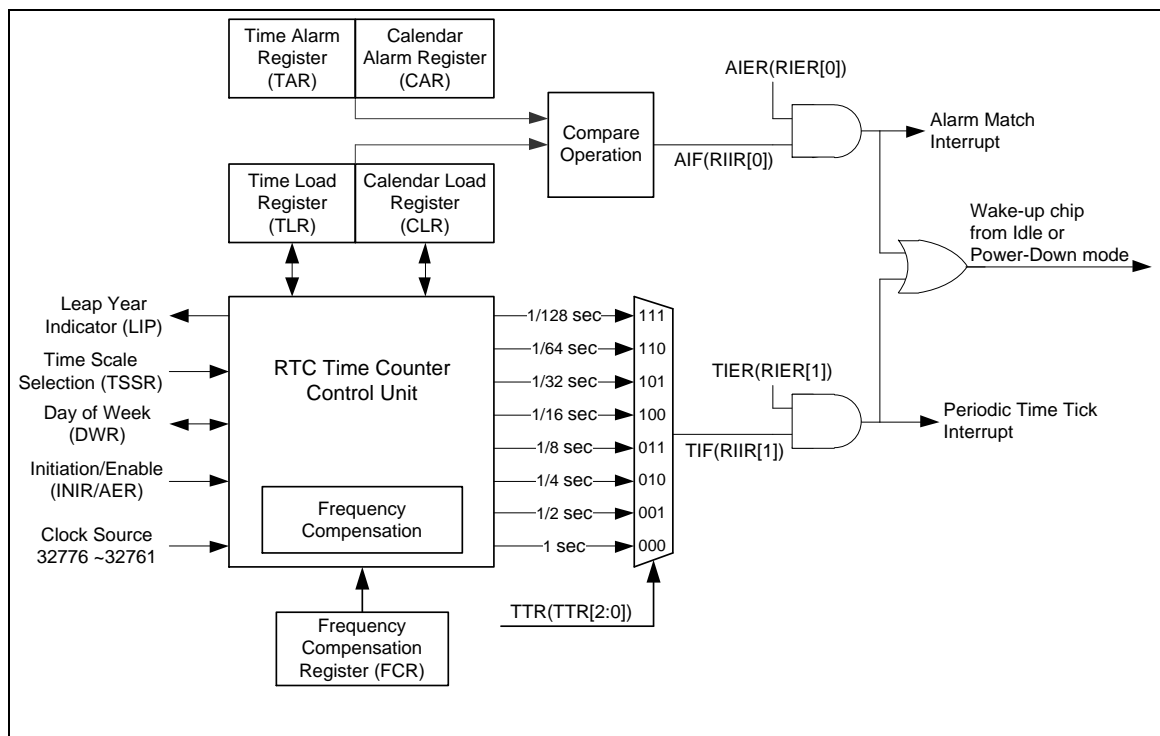
Figure 6-50 RTC Block Diagram
