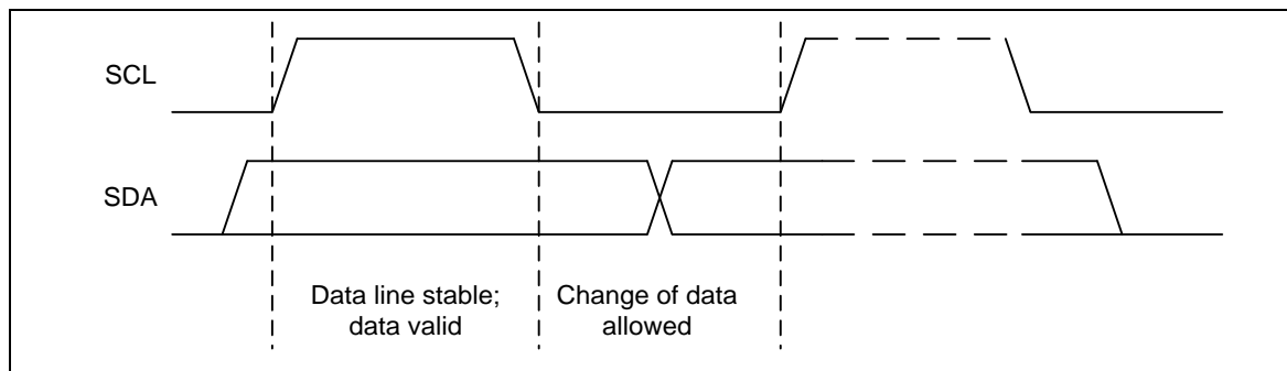
Figure 6-84 Bit Transfer on I 2 C Bus
