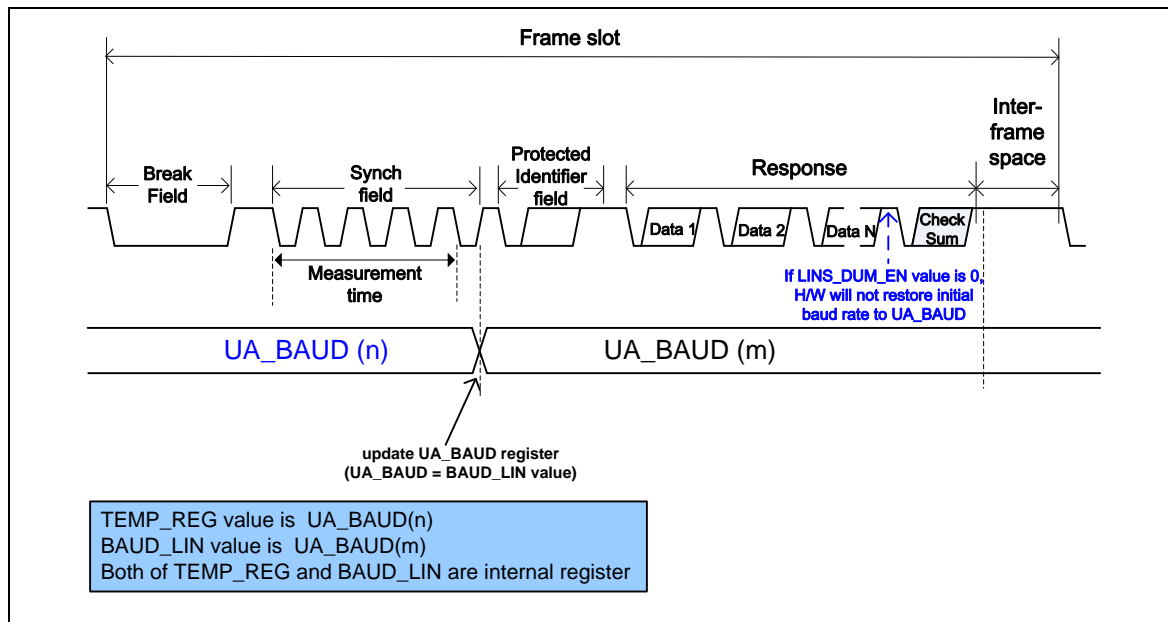
Figure 6-61 UA_BAUD Update Sequence in Automatic Resynchronization Mode when LINS_DUM_EN = 0
