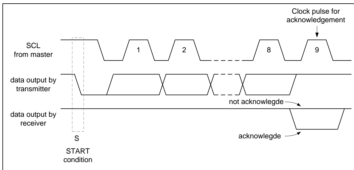
Figure 6-85 Acknowledge on I 2 C Bus
