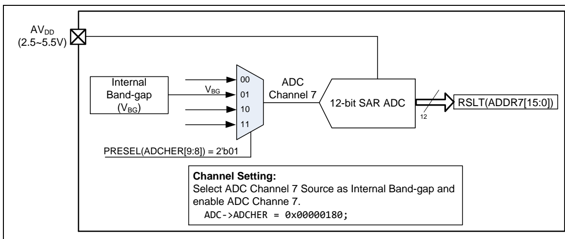
Figure 6-128 V_{BG} for Measuring AV_{DD} Application Block Diagram
