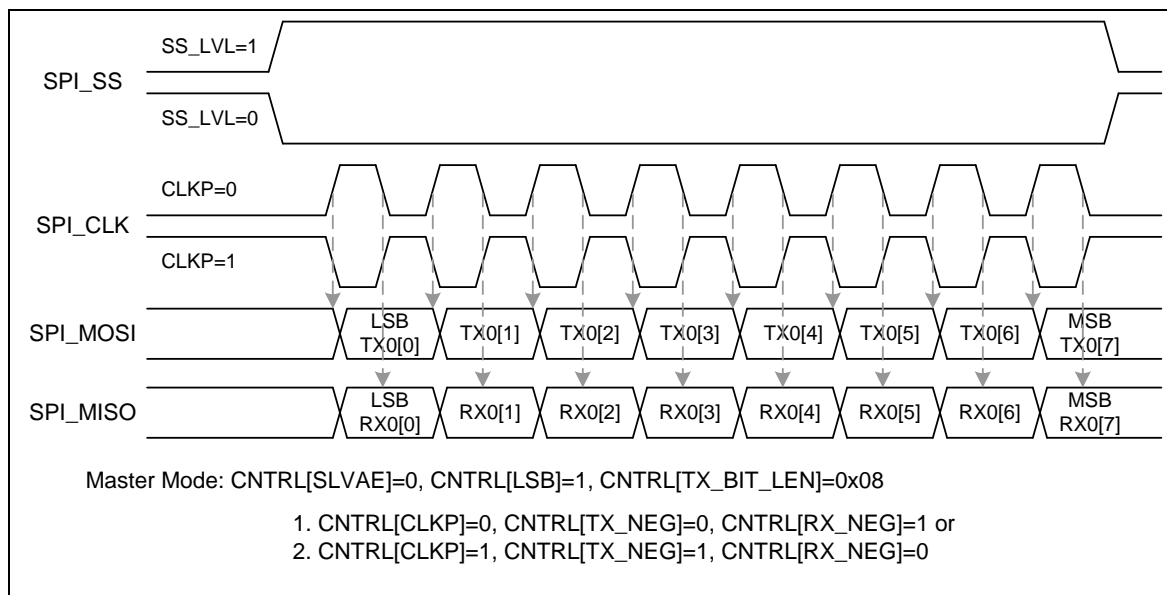
Figure 6-109 SPI Timing in Master Mode (Alternate Phase of SPICLK)
