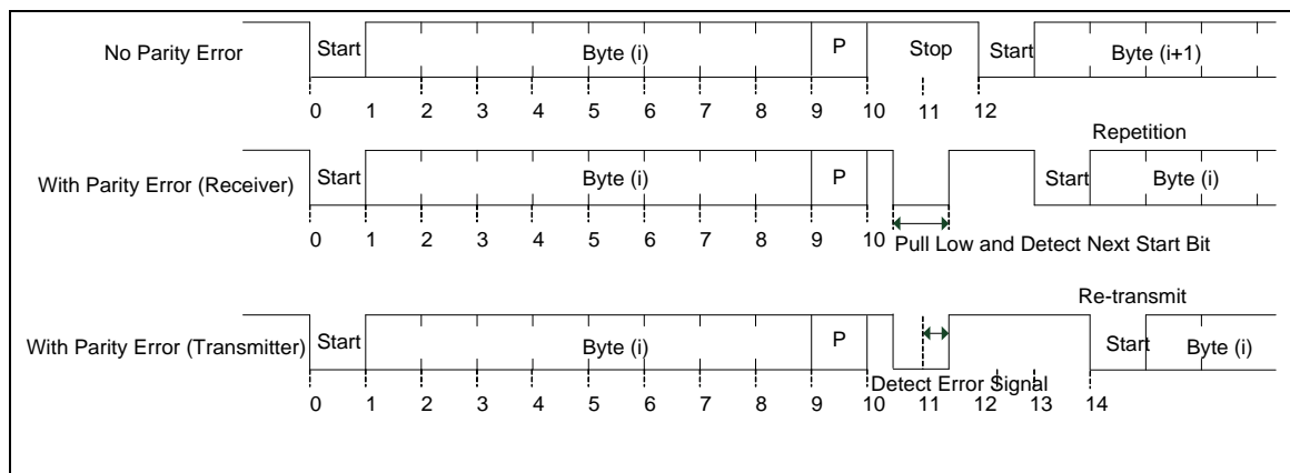
Figure 6-70 SC Error Signal
