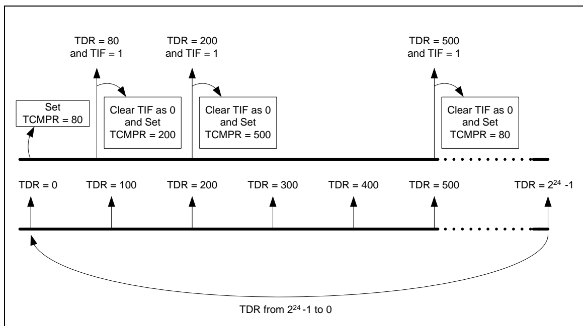
Figure 6-23 Continuous Counting Mode
