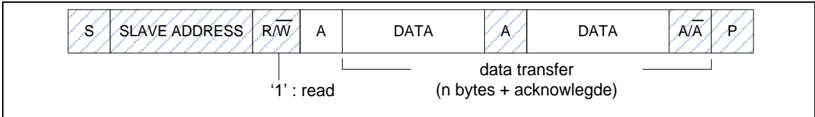
Figure 6-82 Master Reads Data from Slave
