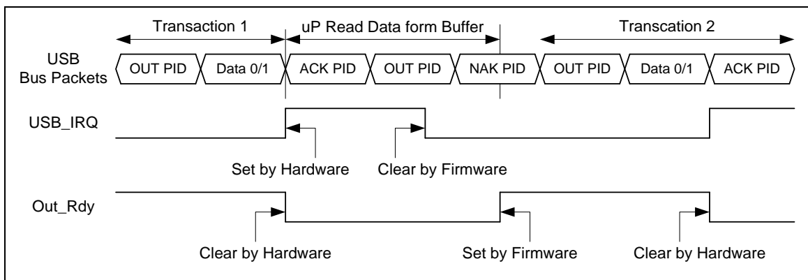
Figure 6-122 Data Out Transfer
