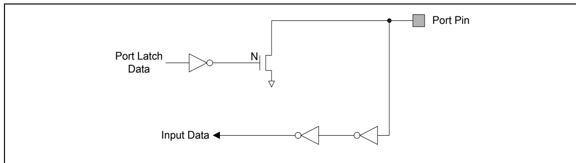
Figure 6-17 Open-Drain Output
