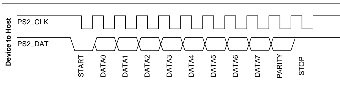
Figure 6-74 Data Format of Device-to-Host
