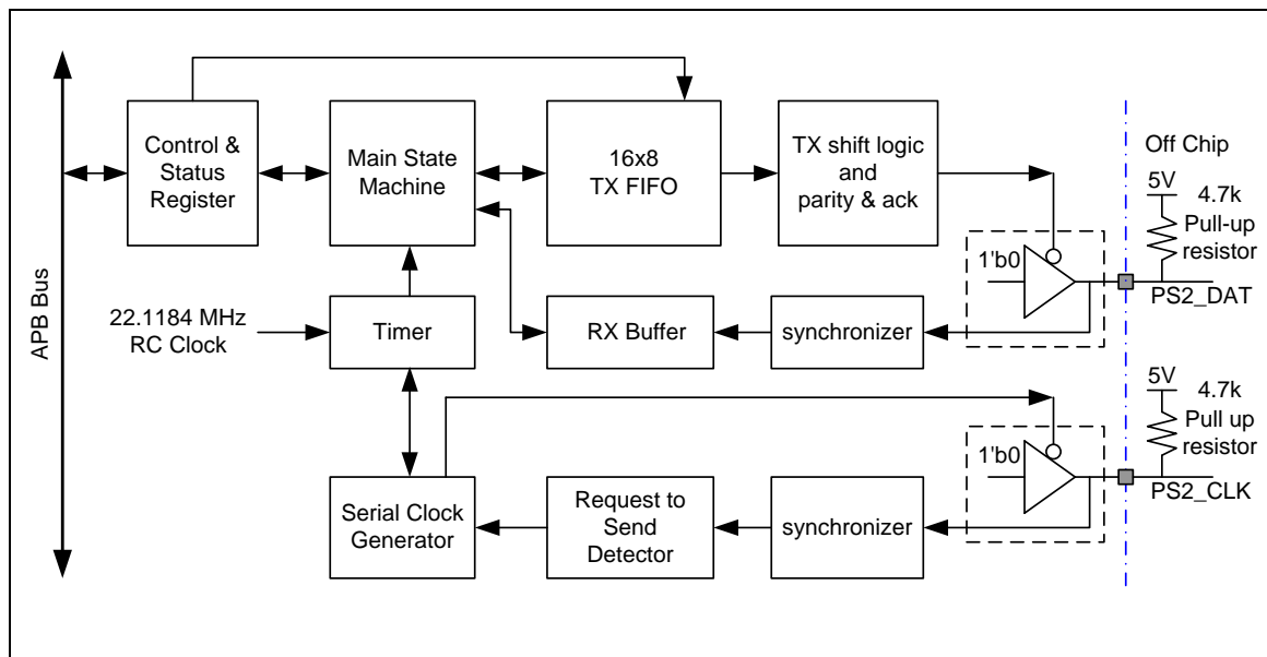
Figure 6-73 PS/2 Device Block Diagram
