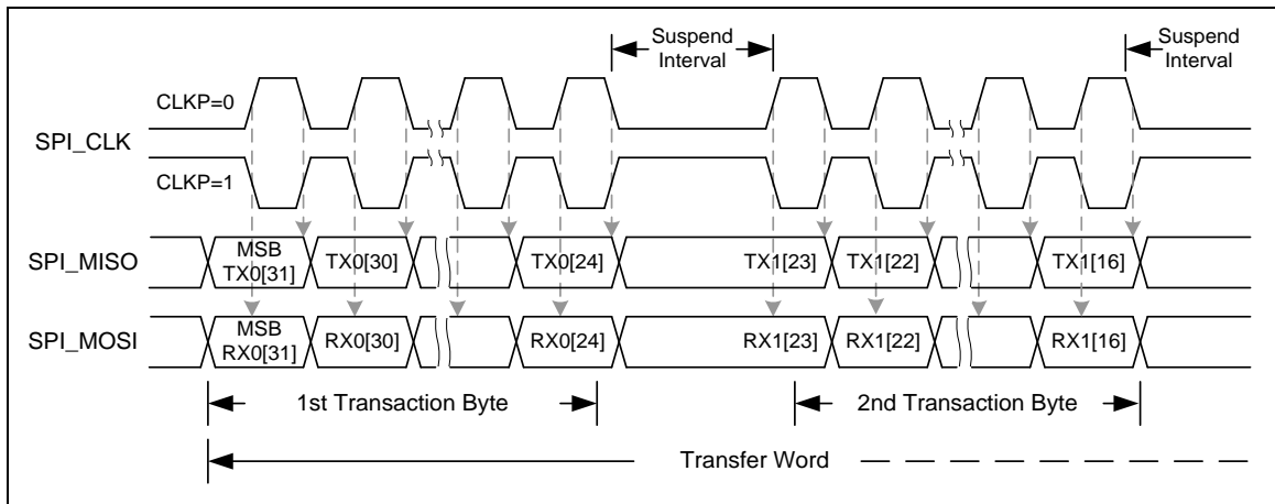
Figure 6-103 Timing Waveform for Byte Suspend
