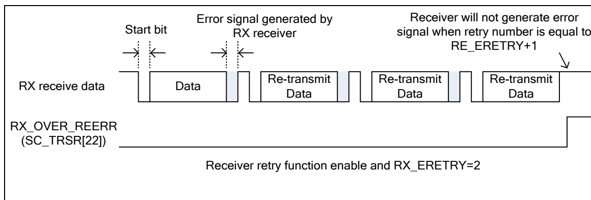
Figure 6-72 SC Receiver Retry Number and Retry Over Flag
