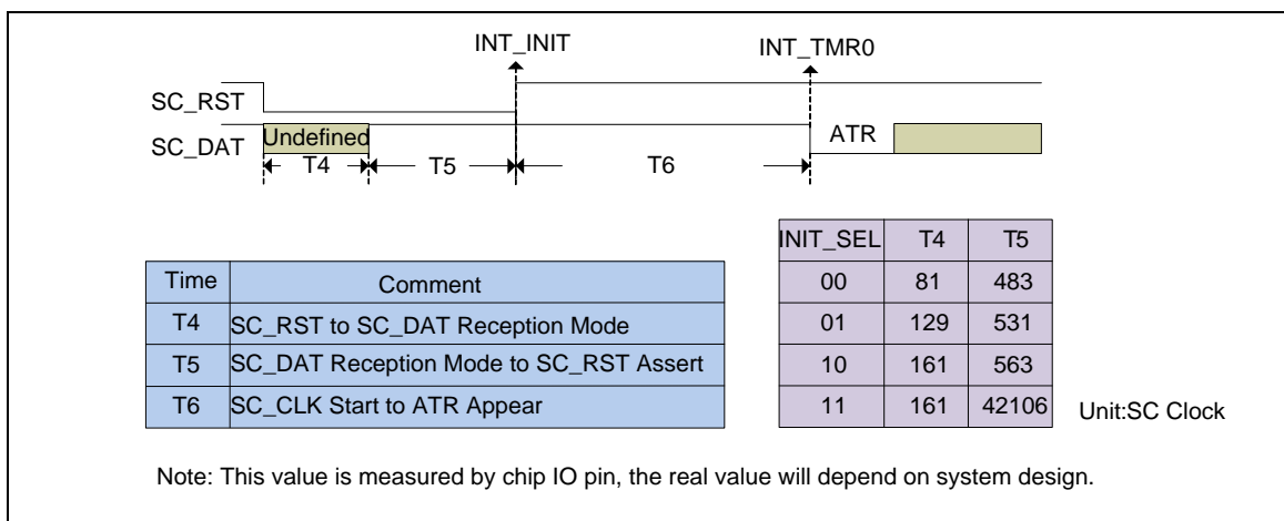
Figure 6-67 SC Warm Reset Sequence
