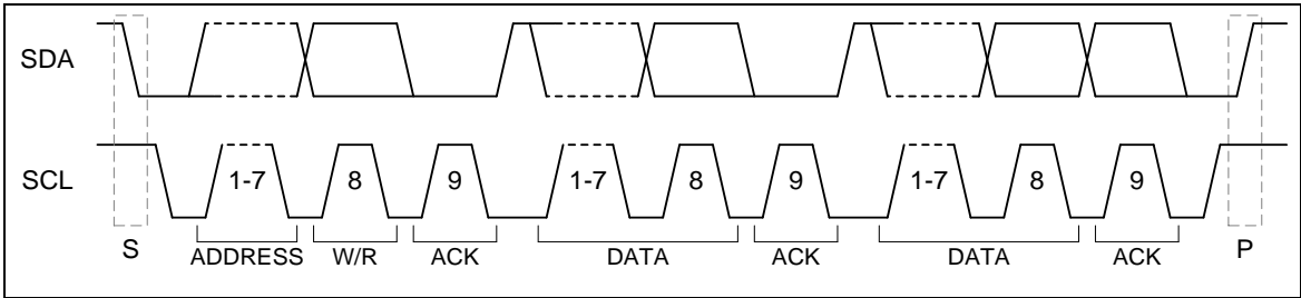
Figure 6-80 I 2 C Protocol
