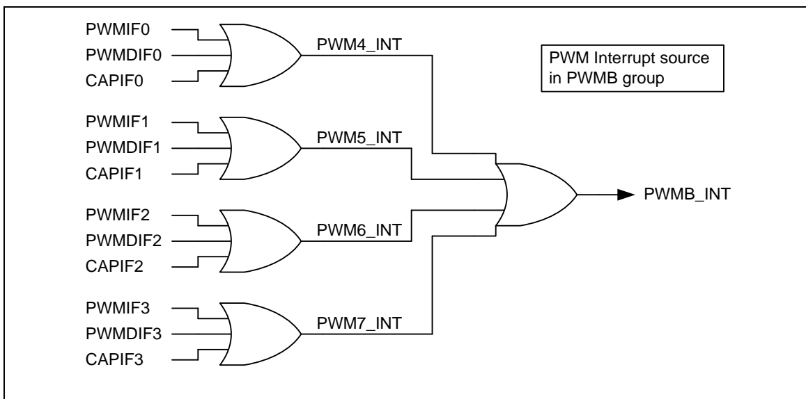
Figure 6-43 PWM Group B PWM-Timer Interrupt Architecture Diagram
