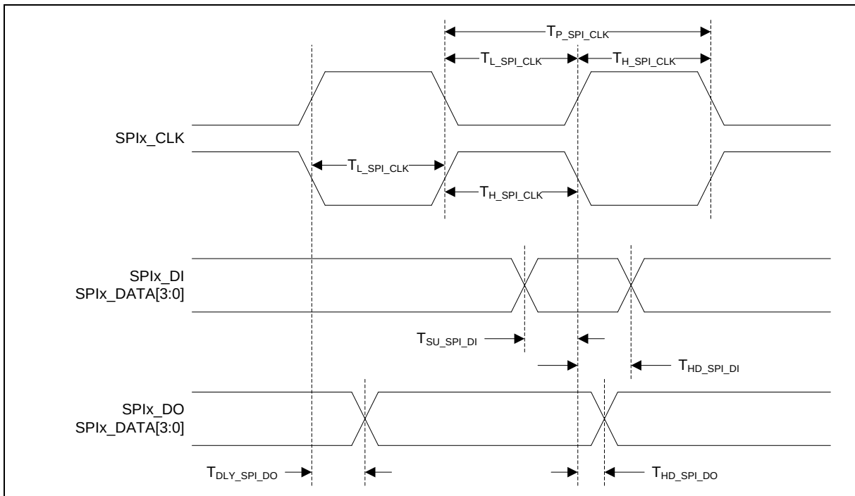
Figure 6.4-6 SPI Interface Timing Diagram
