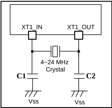
Figure 6.4-2 Typical HXT Crystal Application Circuit
