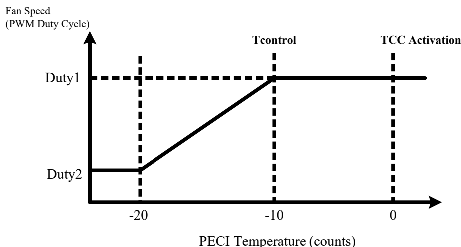
Figure 6-3 PECI Temperature
