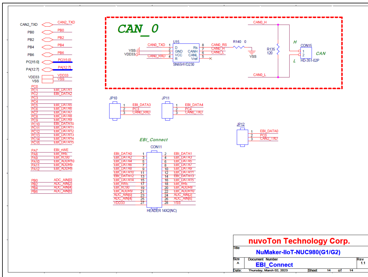
Figure 5-14 Expand EBI Interface and CAN_0
