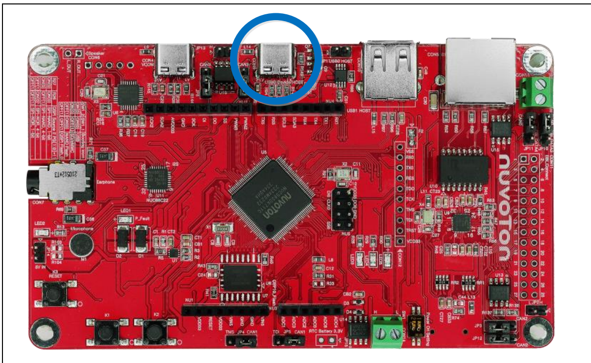
Figure 4-10 USB Port
