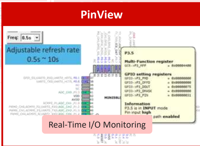
Graphical I/O setting
