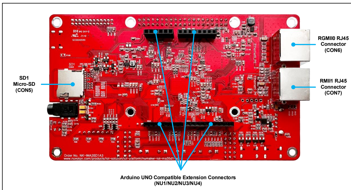
Figure 3-2 Rear View of NuMaker-IoT-MA35D1-A3
