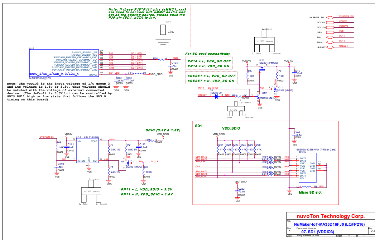
Figure 6-7 SD1 Schematic
