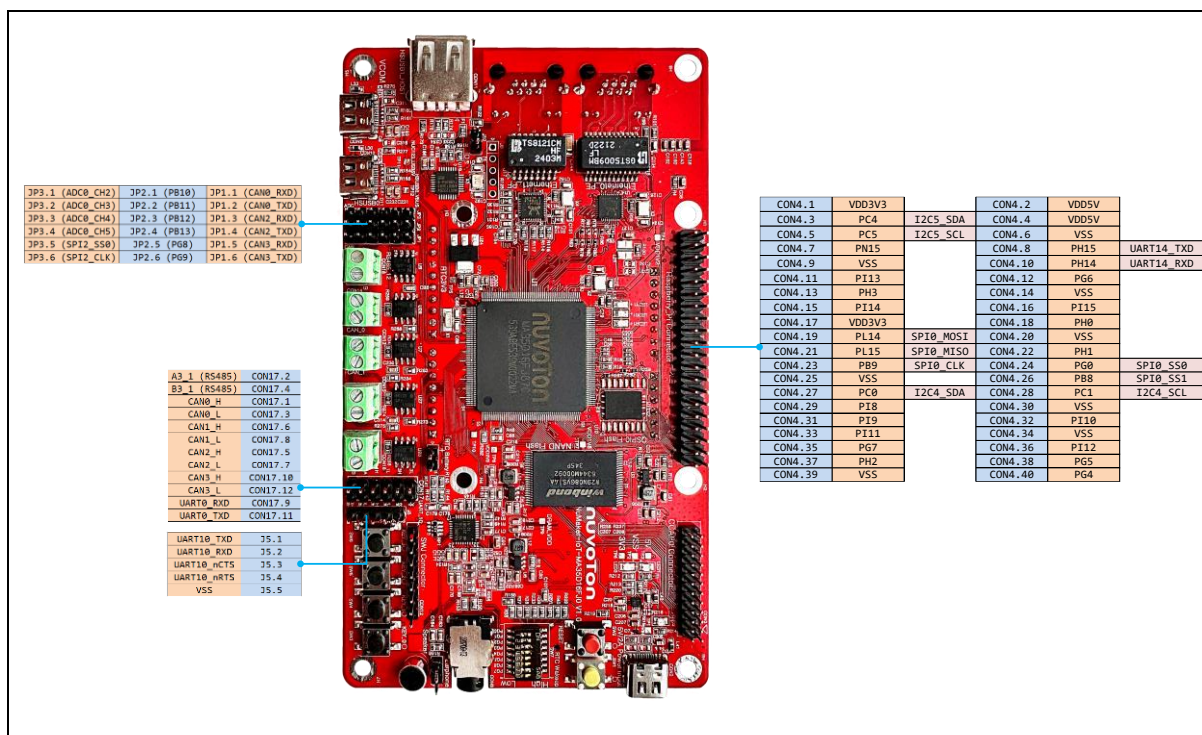
Figure 3-3 JP1~JP3, UART, RS485, CAN Headers and Raspberry Pi Connector
