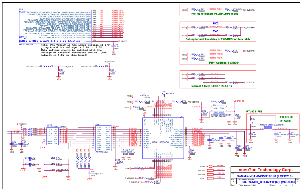
Figure 6-8 RGMII0_PE Schematic
