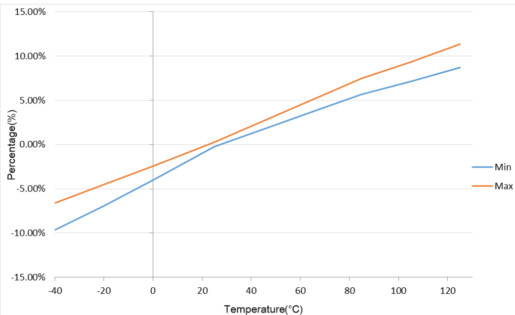
(a) Test condition: V_{DD}=3.6 V, Temp = -40~125°C
