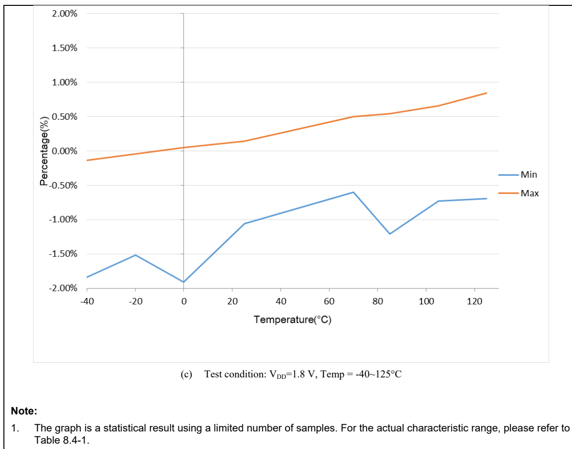
Figure 8.4-1 HIRC vs. Temperature
