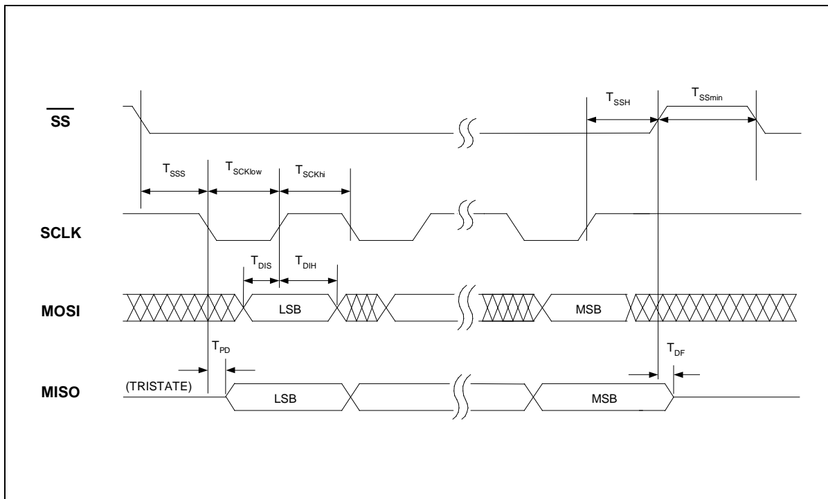
Figure 12.15: SPI Operation
