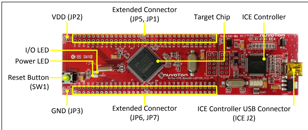
Figure 2-1 NuTiny-SDK-NANO100 (PCB Board)
