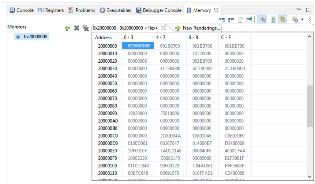
Figure 4-10 Memory View
