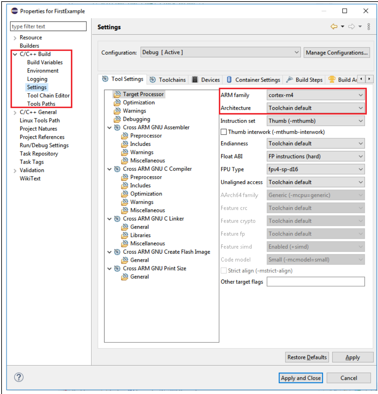
Figure 4-5 Build Settings
