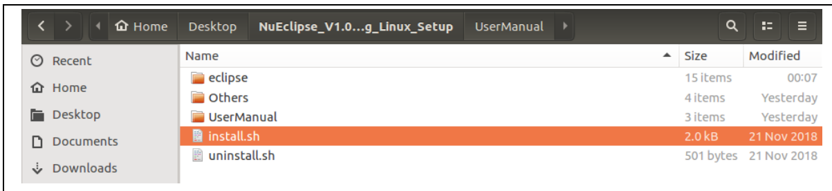
Figure 3-2 Install.sh Script
