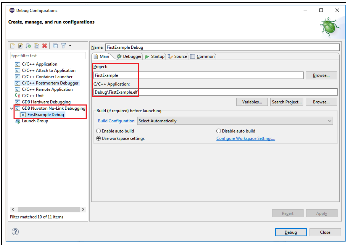
Figure 4-6 Debug Configuration
