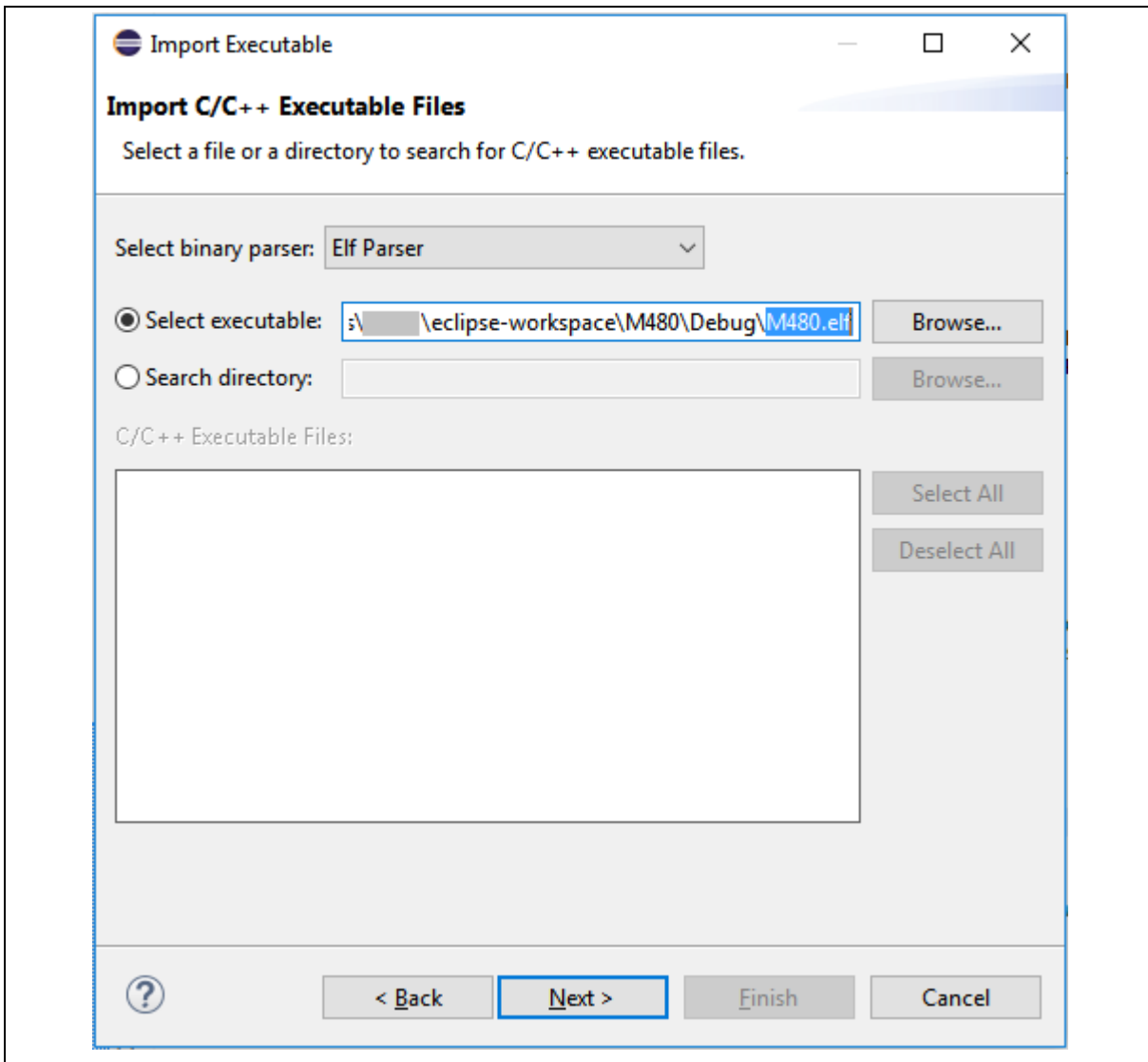
Figure 4-27 Selecting Executable
