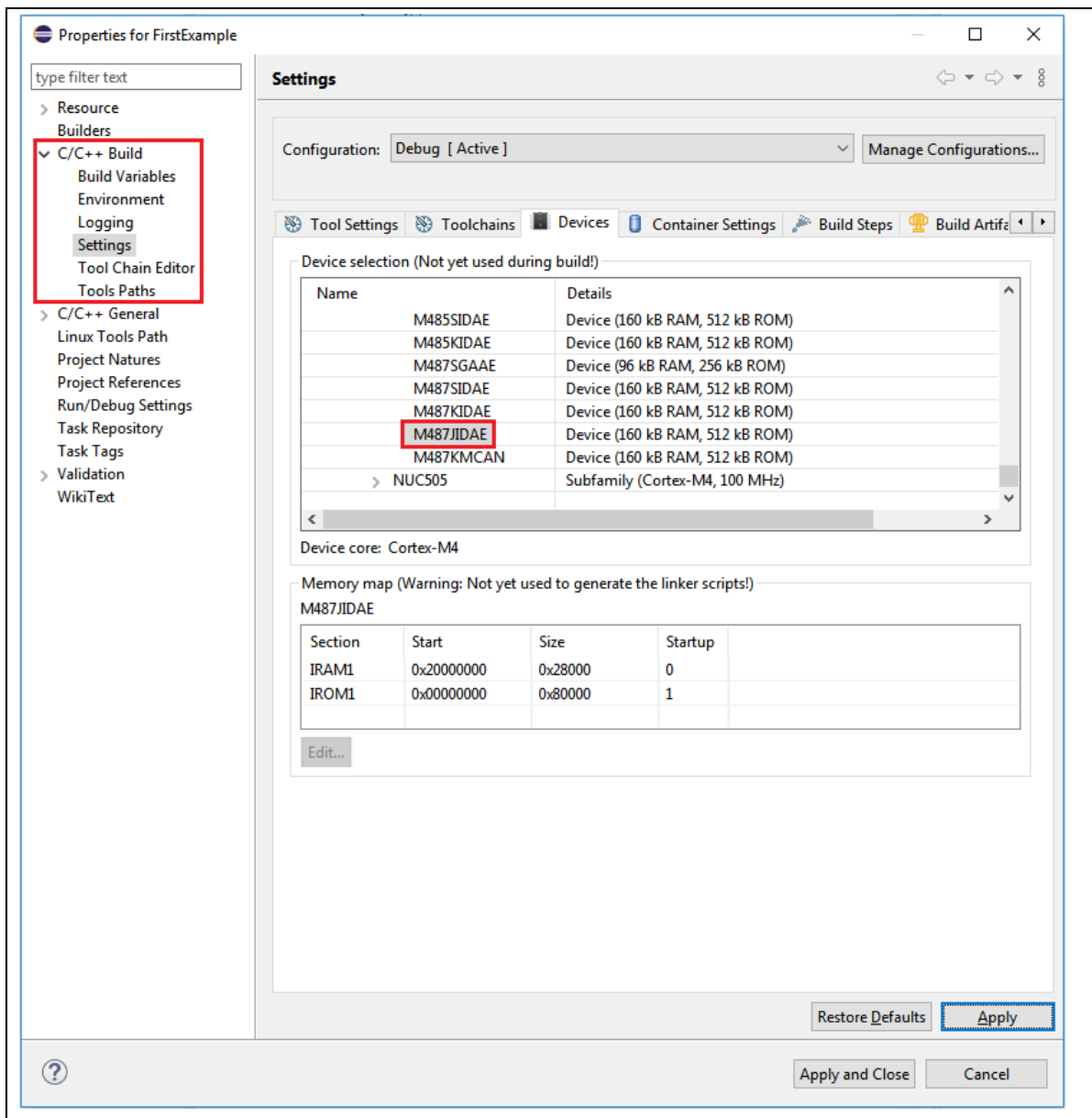
Figure 4-17 Device Selection
