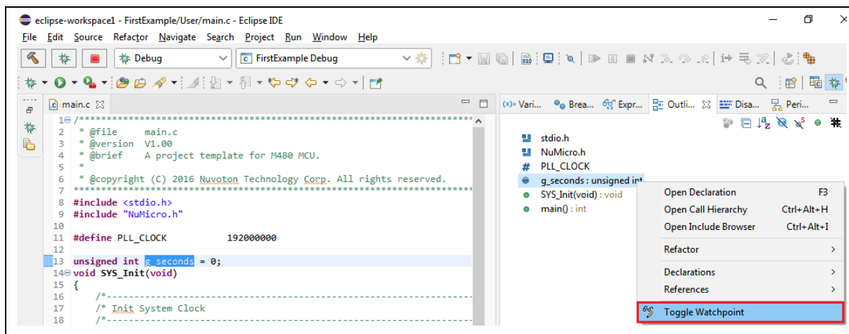
Figure 4-19 Toggle Watchpoint
