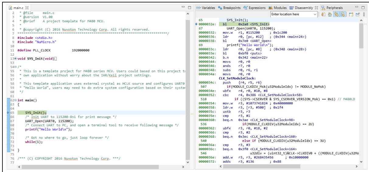
Figure 4-12 Disassembly View
