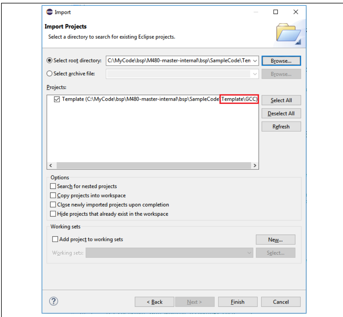
Figure 4-4 Importing Projects
