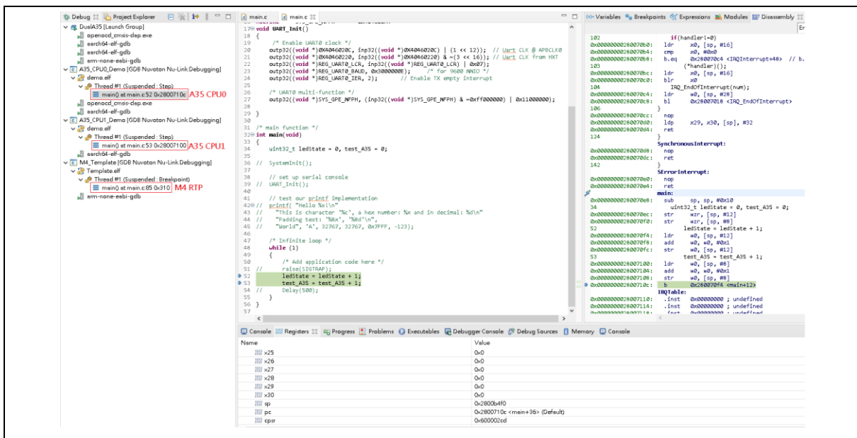
Figure 4-39 Multi-core Debugging
