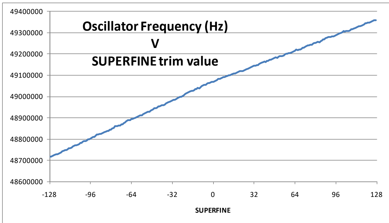
Figure 7-17 Example SUPERFINE Trim Frequency Adjustment.
