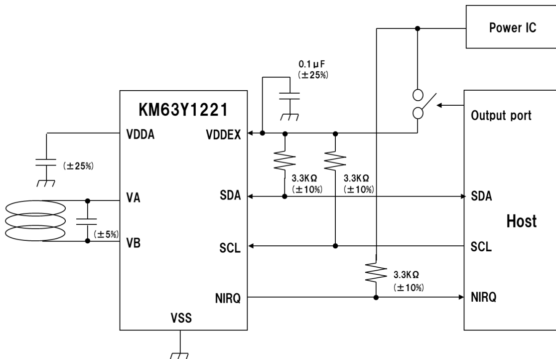
Figure 2-3 Connection Example
