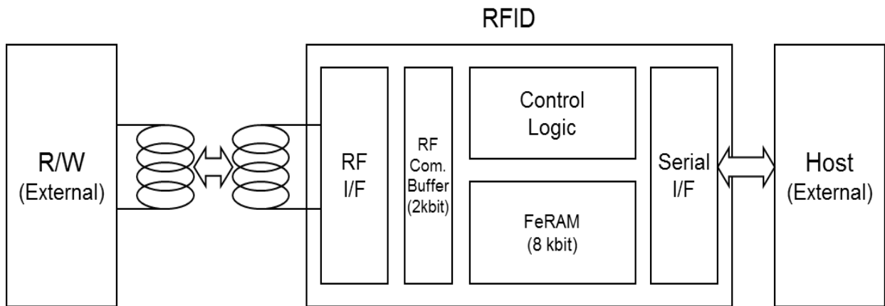
Figure 1-1 Block Diagram
