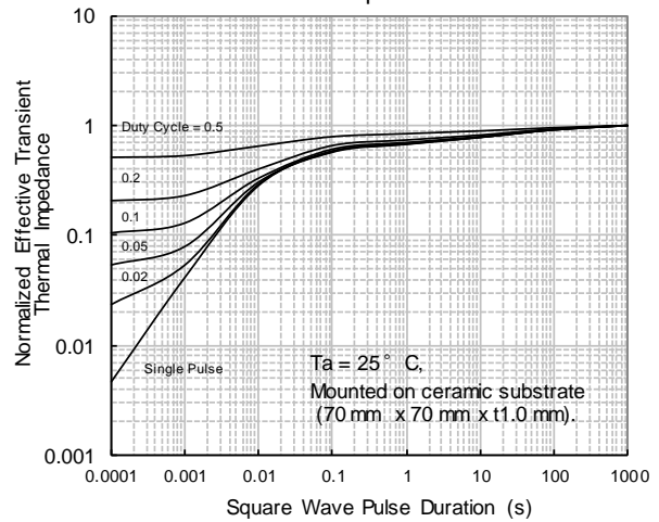
Thermal Response
