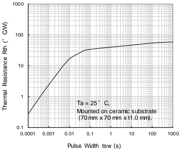
Rth - tsw
