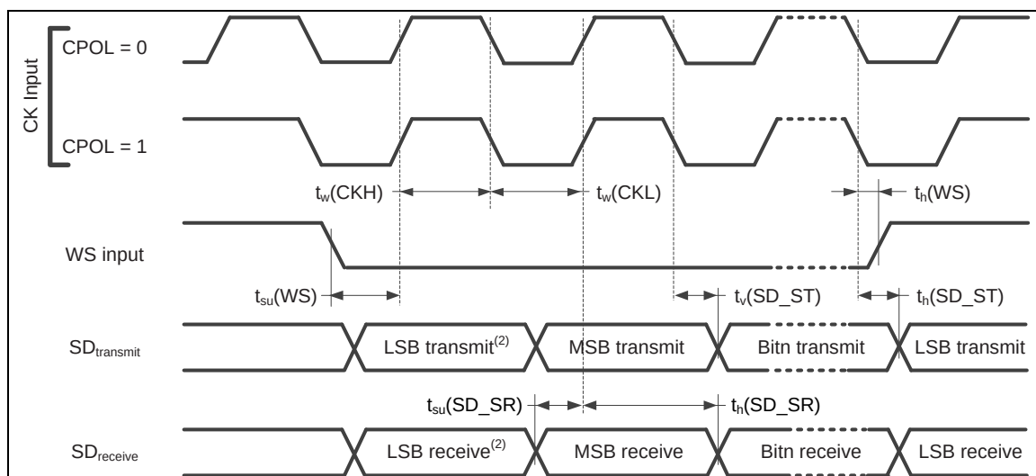
Figure 7.8-2 I²S Slave Mode Timing Diagram
