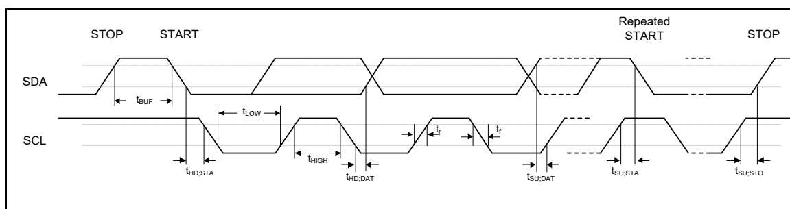
Figure 7.6-1 I 2 C Timing Diagram
