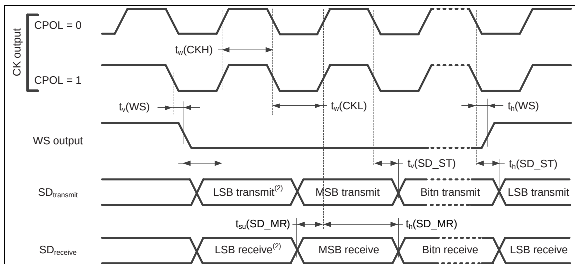
Figure 7.8-1 I²S Master Mode Timing Diagram
