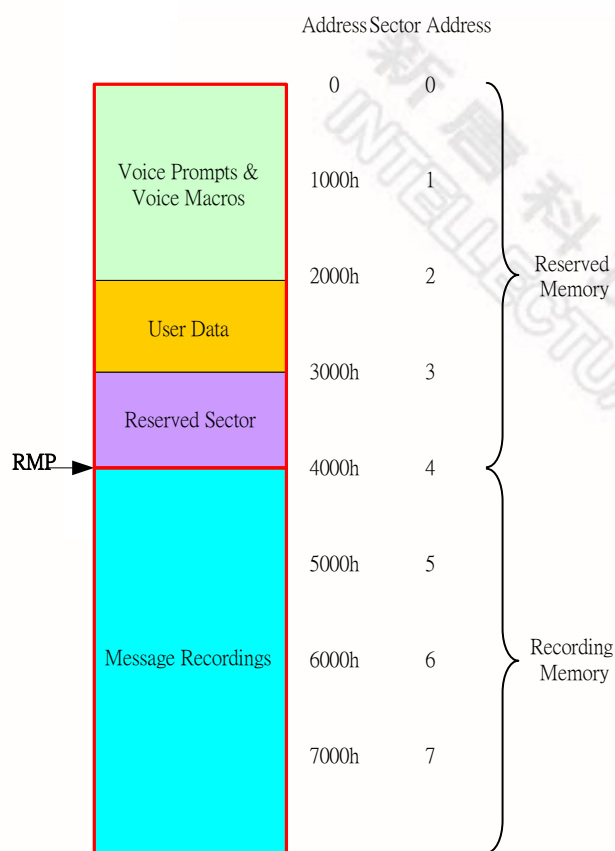
Figure 8-1 ISD3900 Memory Format
