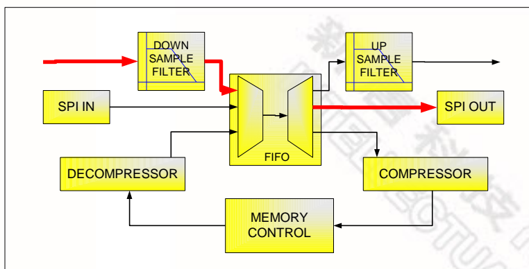
Figure 13-4 Feed-through SPI
