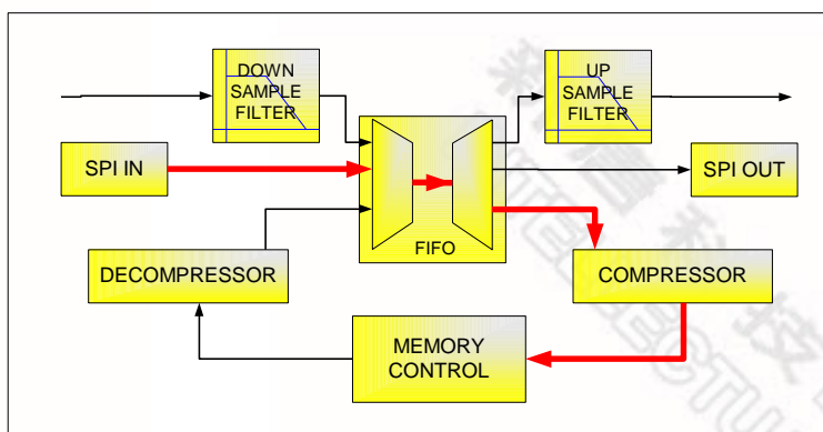
Figure 13-1 SPI Record
