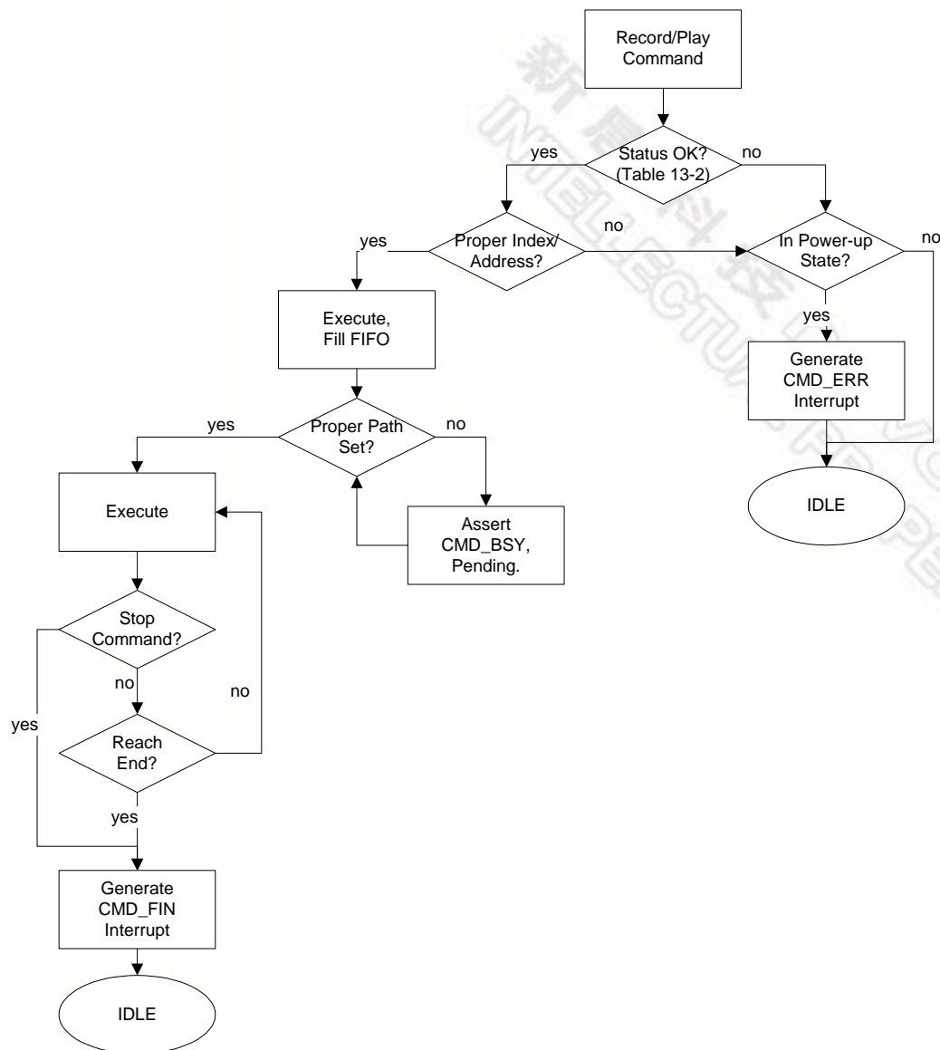
Figure 11-2 Record/Playback Flowchart
