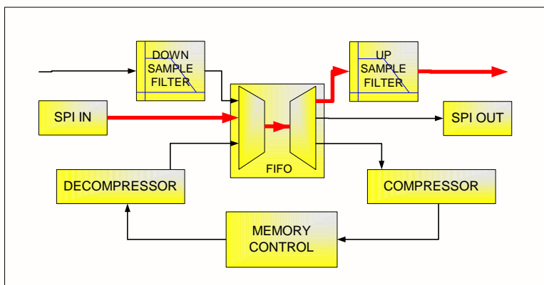
Figure 13-2 SPI Feed-through
