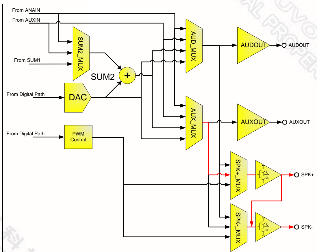
Figure 12-1 BTL from the AUX_MUX (the red line)
