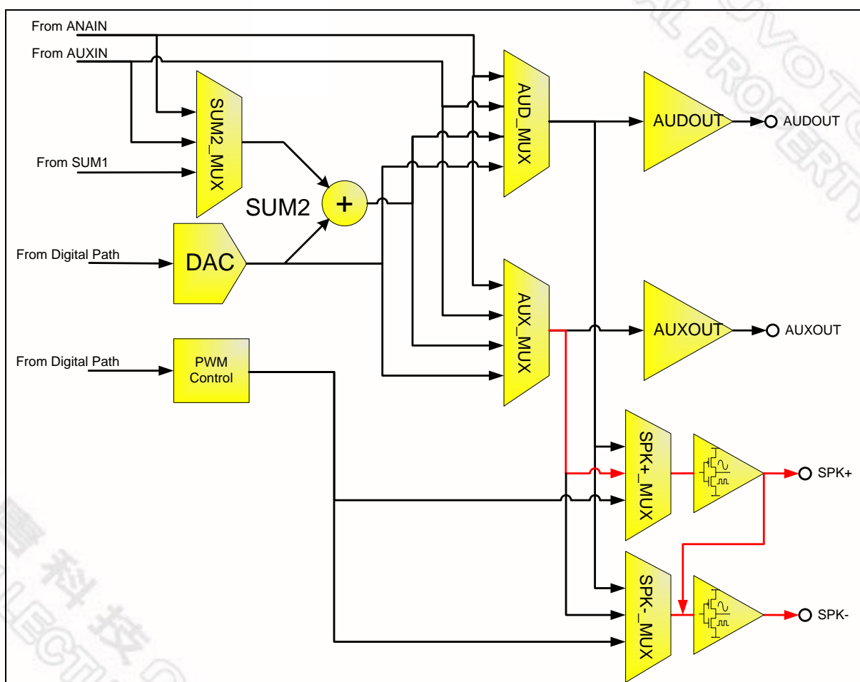
Figure 7-6 Analog Outputs
