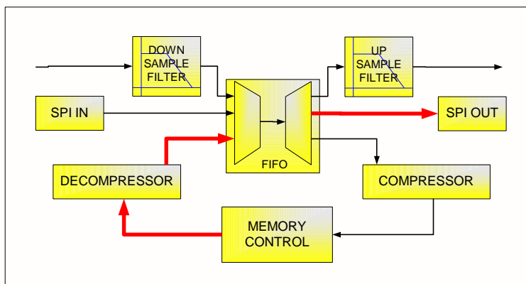
Figure 13-3 SPI Playback
