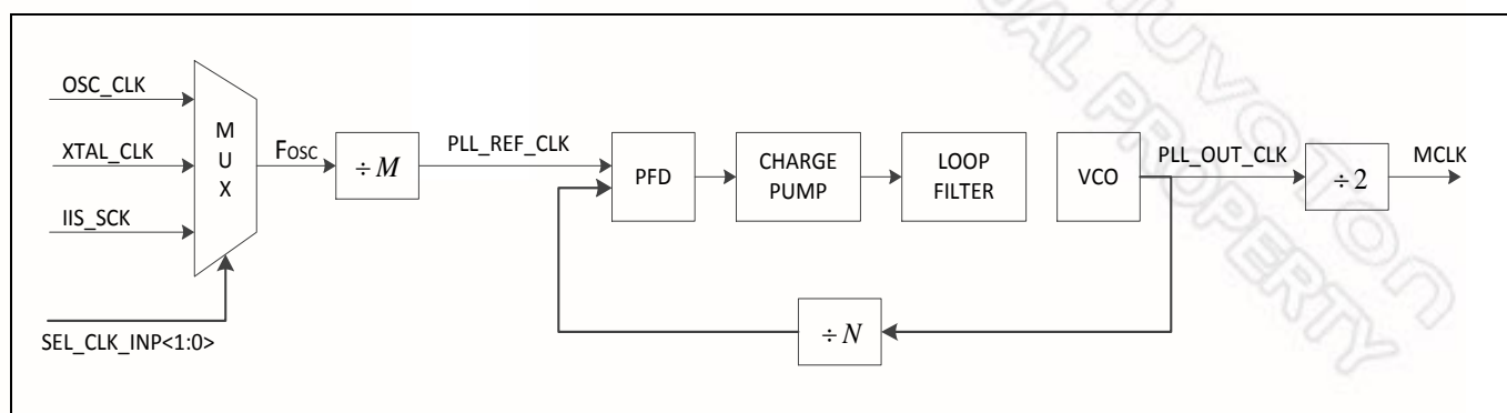
Figure 10-1 PLL Clock Generation on ISD3900
