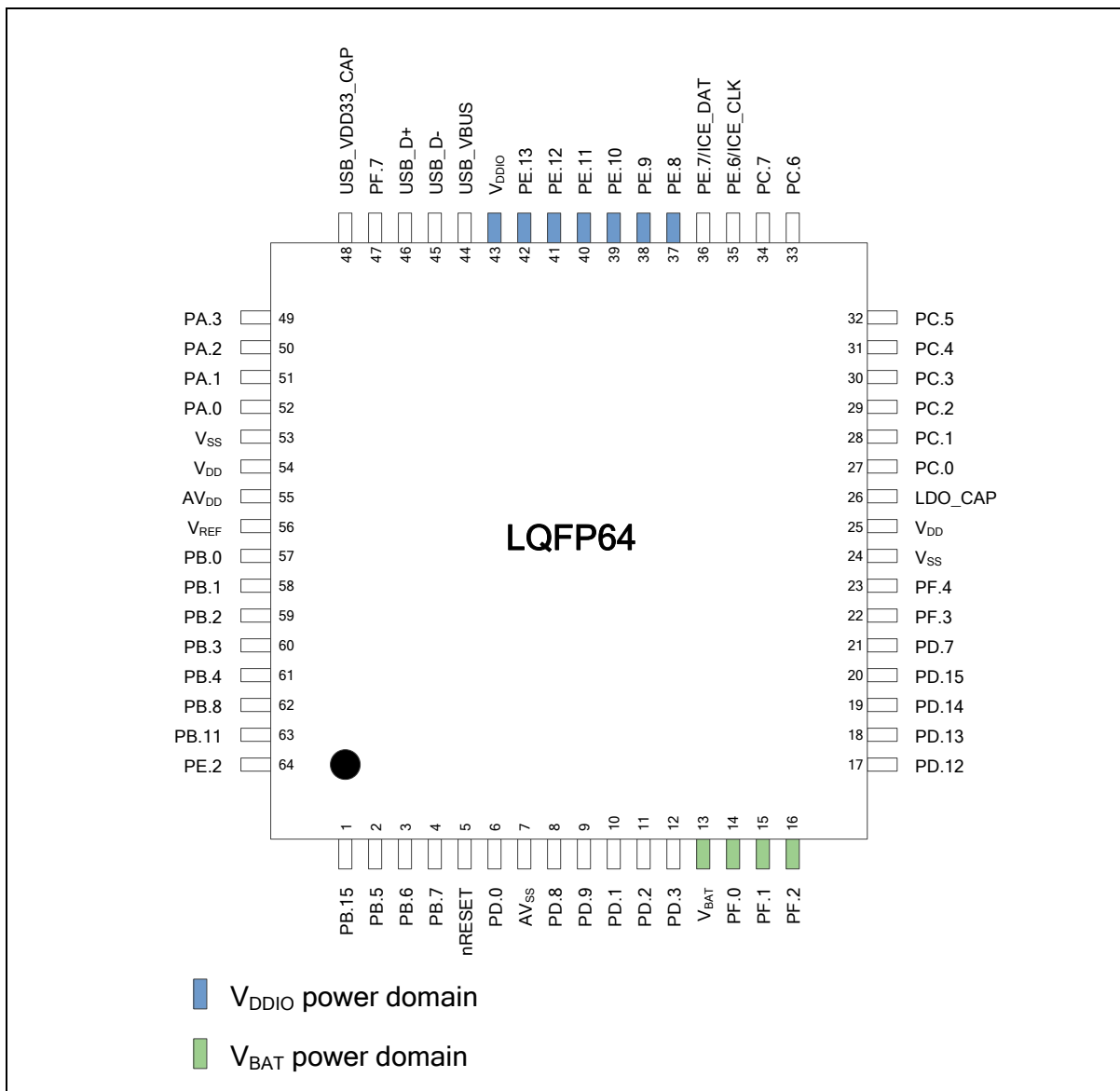
Figure 4.1-2 NuMicro® NUC029SGE LQFP 64-pin Diagram
