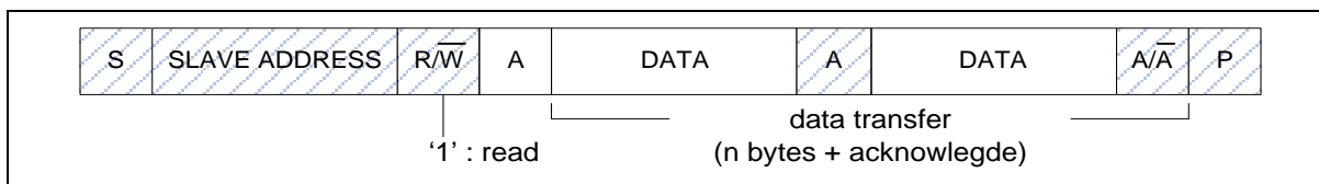
Figure 6.22-10 Master Reads Data from Slave with a 7-bit address
