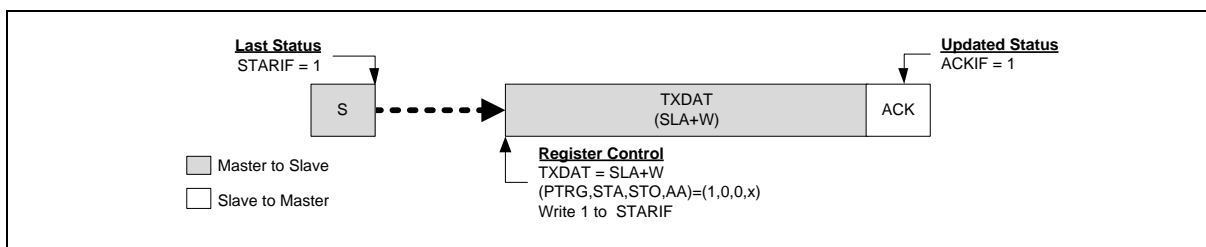
Figure 6.22-8 Control I 2 C Bus according to Current I 2 C Status
