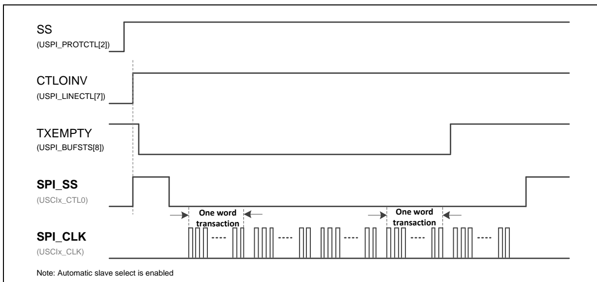
Figure 6.21-13 Auto Slave Select ( SUSPITV < 0x3 )
