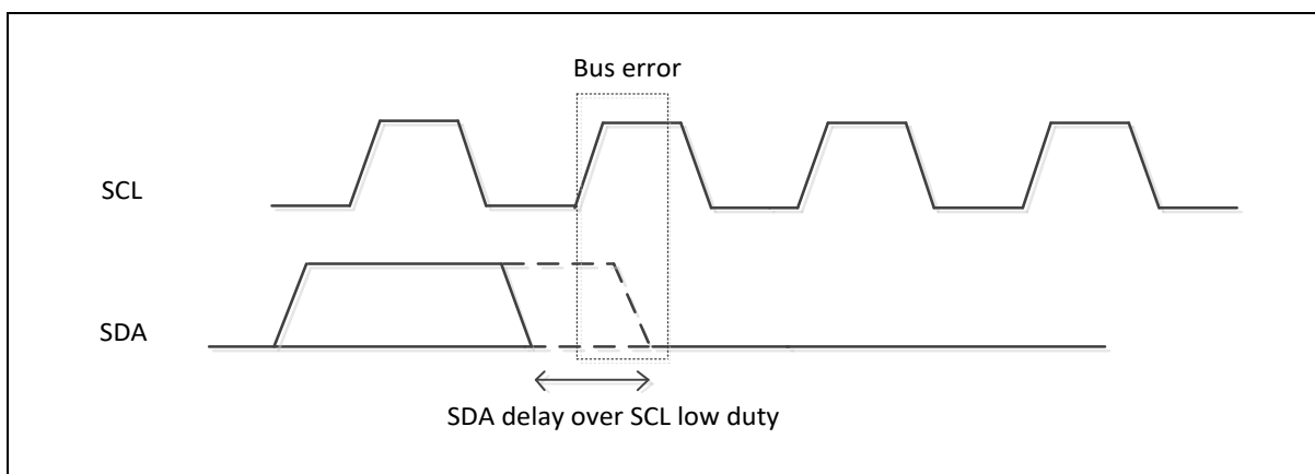
Figure 6.11-18 Hold Time Wrong Adjustment
