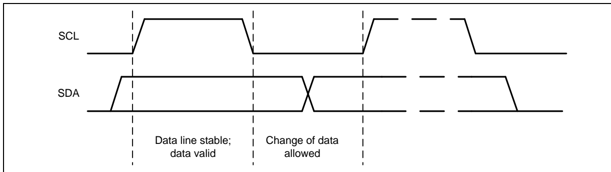
Figure 6.22-5 Bit Transfer on the I²C Bus
