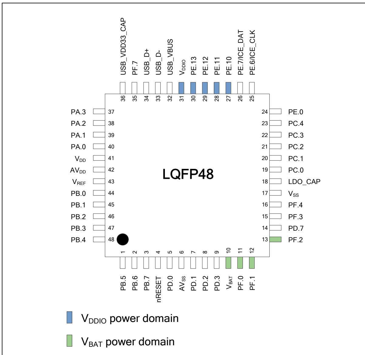
Figure 4.1-1 NuMicro® NUC029LGE LQFP 48-pin Diagram
