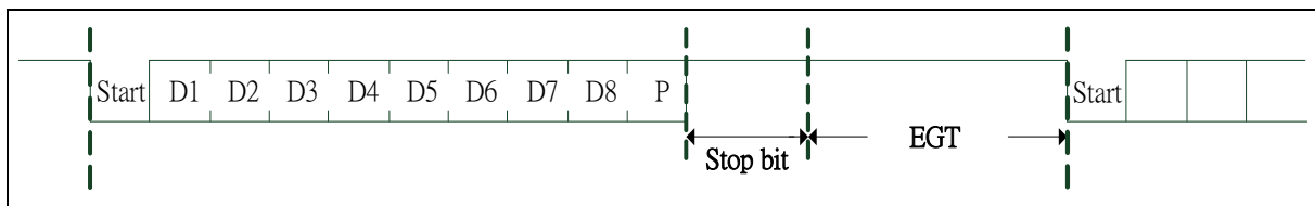
Figure 6.15-12 Extra Guard Time Operation
