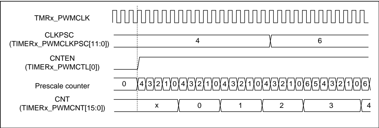
Figure 6.17-13 PWM Prescale Waveform in Up Count Type
