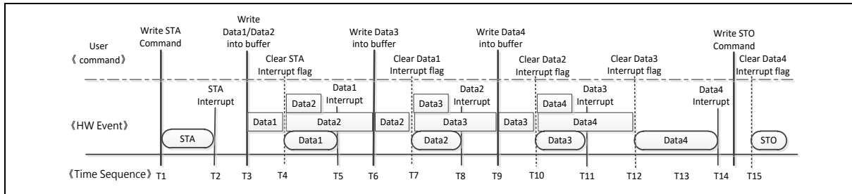
Figure 6.11-15 Timing of Two-level Buffer Transmit in Master Write
