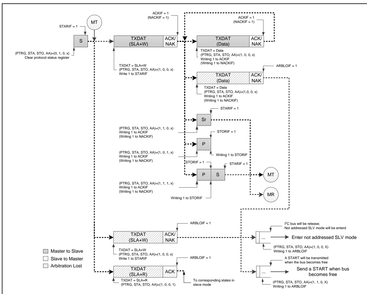
Figure 6.22-13 Master Transmitter Mode Control Flow with 7-bit Address
