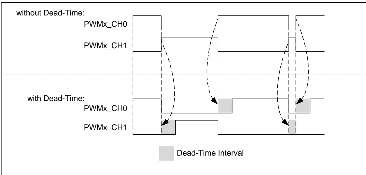
Figure 6.17-26 Dead-Time Insertion
