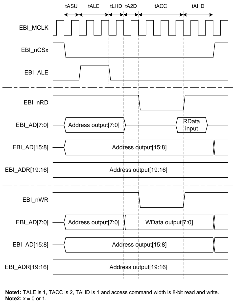
Figure 6.8-5 Timing Control Waveform for 8-bit Data Width
