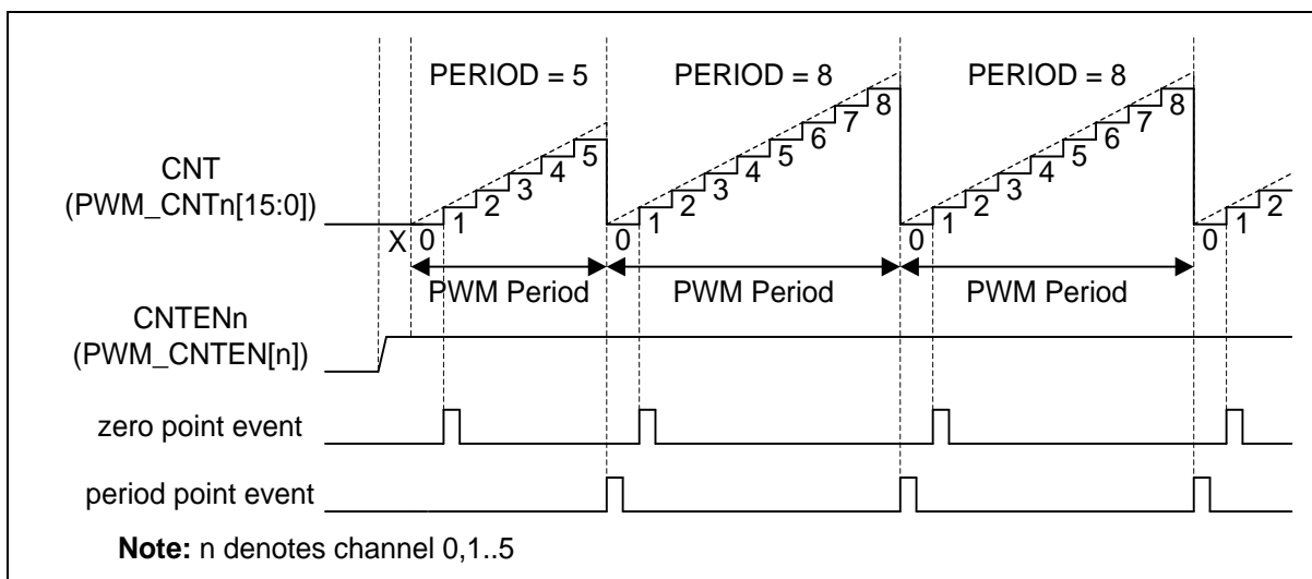
Figure 6.13-7 PWM Up Counter Type
