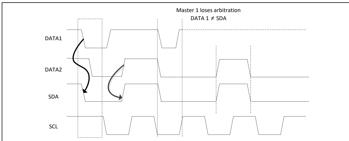
Figure 6.22-7 Arbitration Lost
