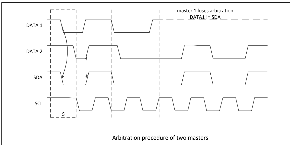
Figure 6.11-14 Arbitration Lost
