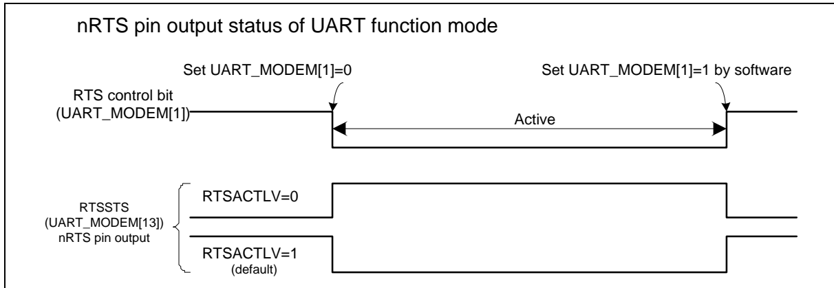
Figure 6.23-14 UART nRTS Auto-Flow with Software Control
