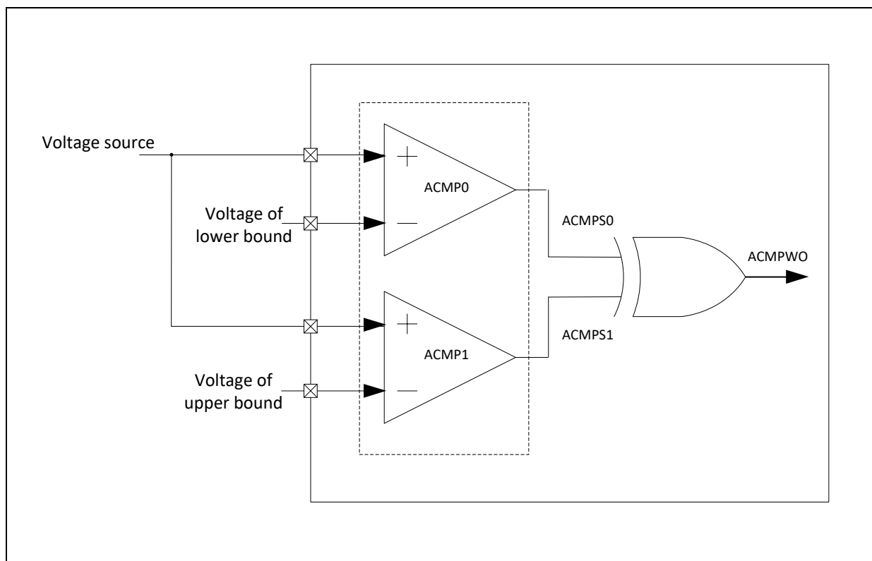
Figure 6.5-7 Example Connection of Window Compare Mode
