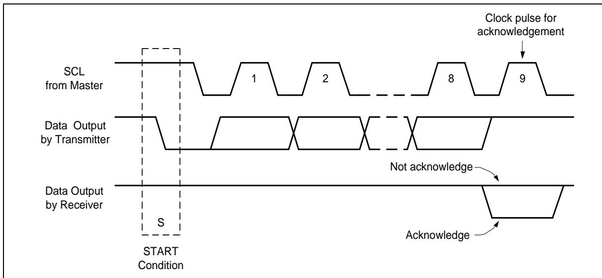
Figure 6.22-6 Acknowledge on the I²C Bus
