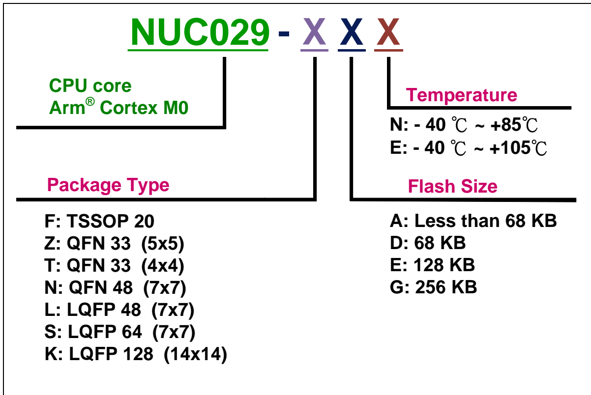
Figure 3.1-1 NuMicro® NUC029 Series Selection Code
