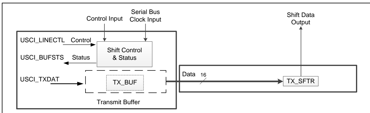
Figure 6.19-6 Transmit Data Path
