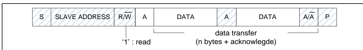
Figure 6.11-8 Master Reads Data from Slave by 7-bit
