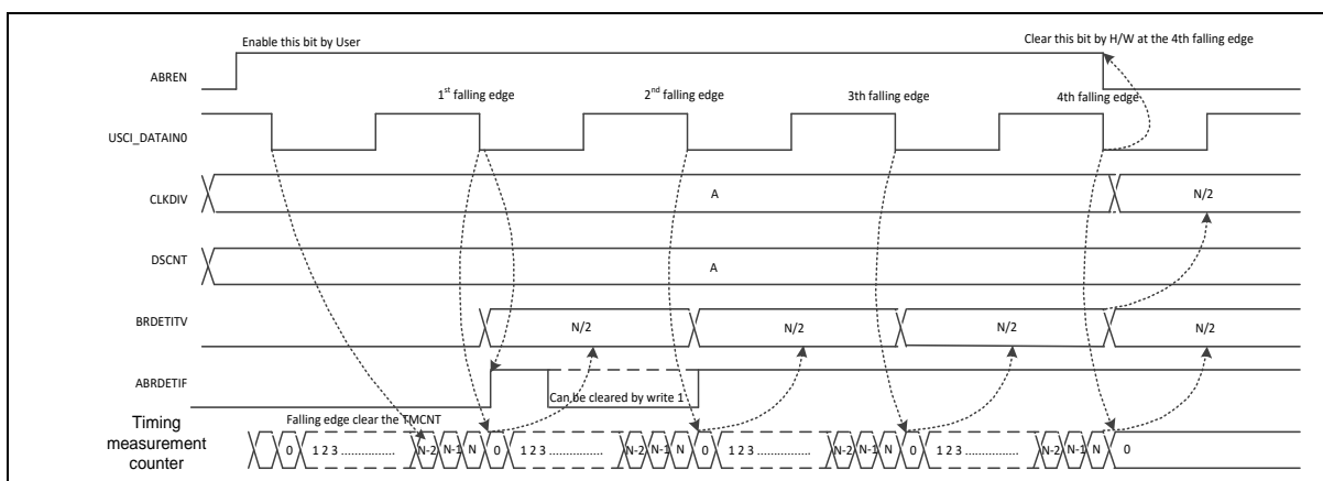
Figure 6.20-5 UART Auto Baud Rate Control
