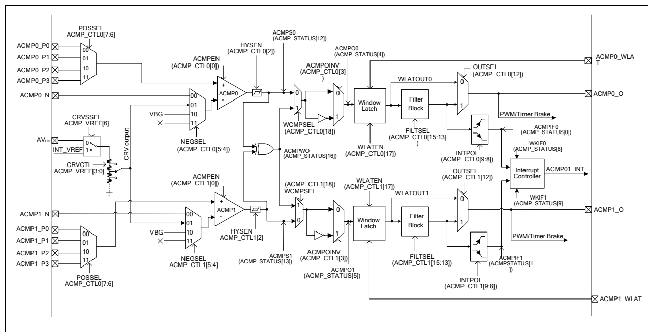
Figure 6.5-1 Analog Comparator Block Diagram
