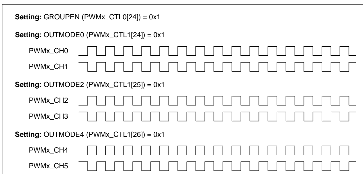
Figure 6.13-21 PWM Group Function Waveform
