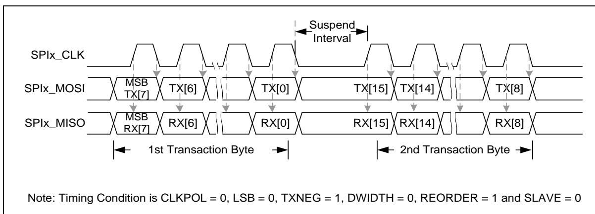
Figure 6.16-9 Timing Waveform for Byte Suspend
