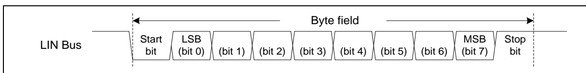
Figure 6.23-18 Structure of LIN Byte
