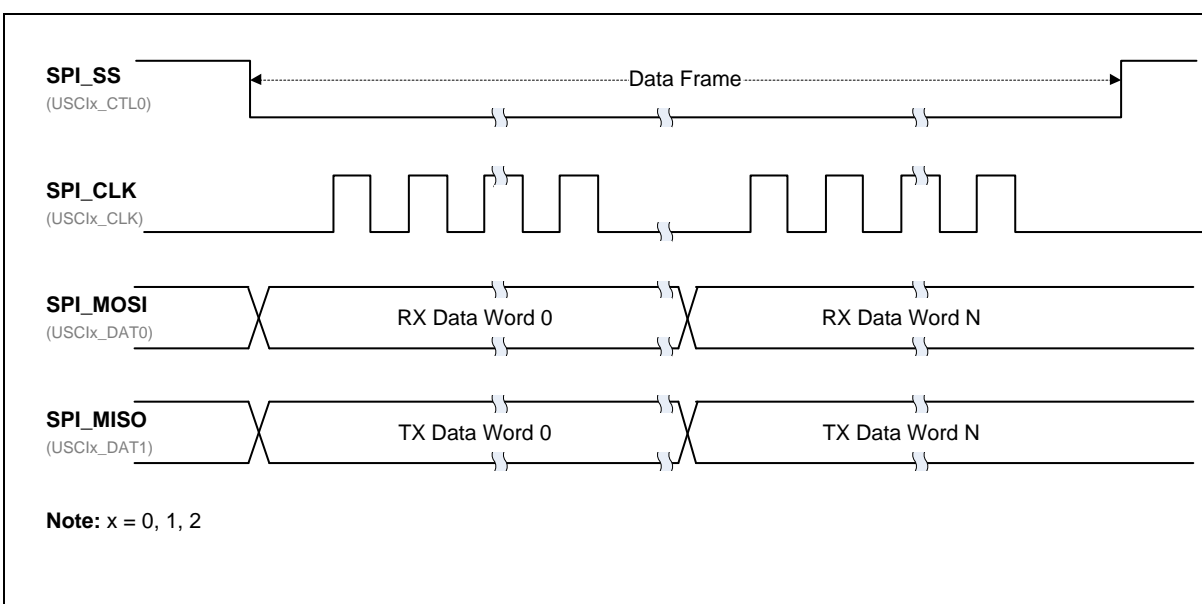
Figure 6.21-5 Wire Full-Duplex SPI Communication Signals (Slave Mode)
