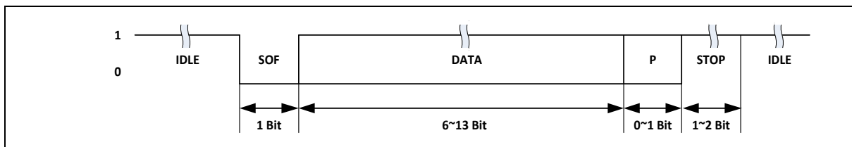
Figure 6.20-3 UART Standard Frame Format
