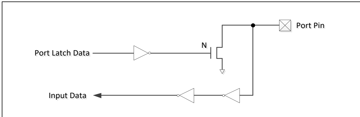
Figure 6.9-3 Open-Drain Output
