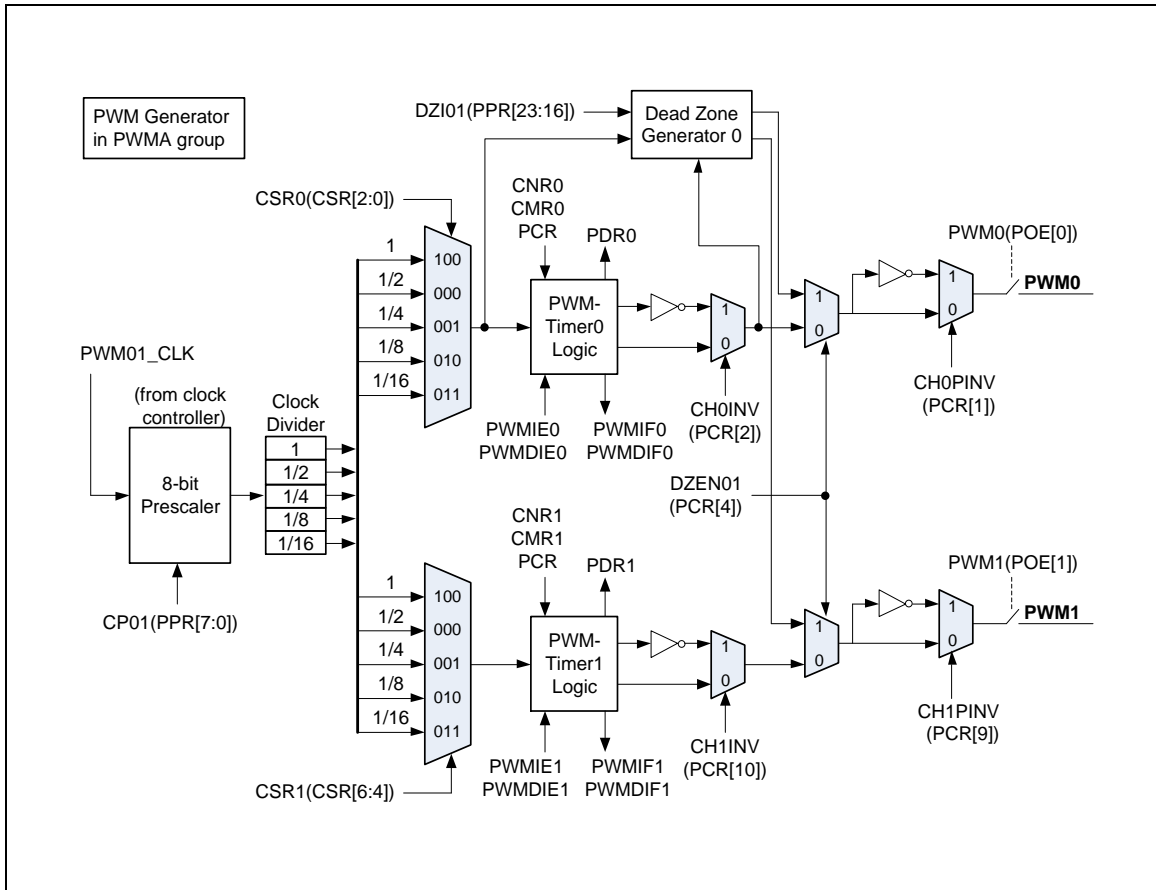
Figure 5-46 PWM Generator 0 Architecture Diagram
