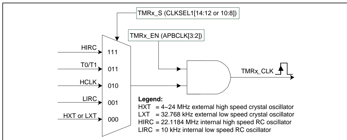
Figure 5-42 Clock Source of Timer Controller for NUC029FAE
