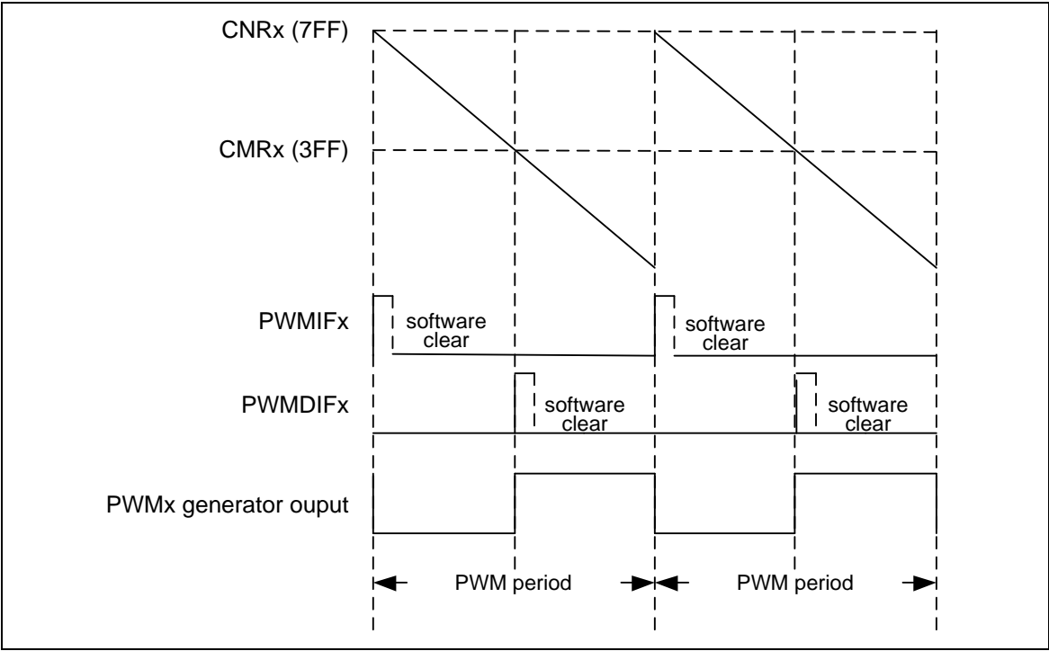
Figure 5-55 PWM Period Interrupt Generate Timing Waveform
