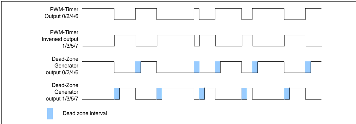
Figure 5-60 Paired-PWM Output with Dead-zone Generation Operation
