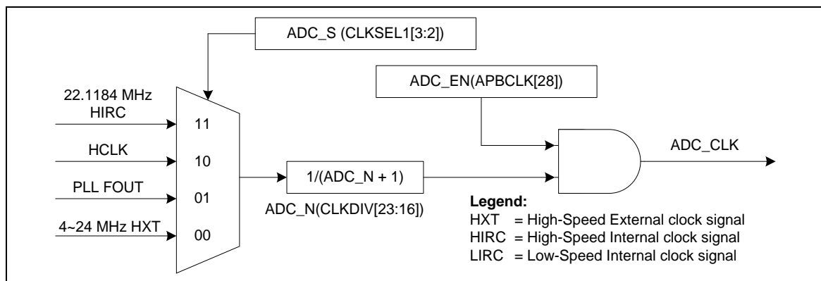
Figure 5-135 ADC Peripheral Clock Control for NUC029xAN
