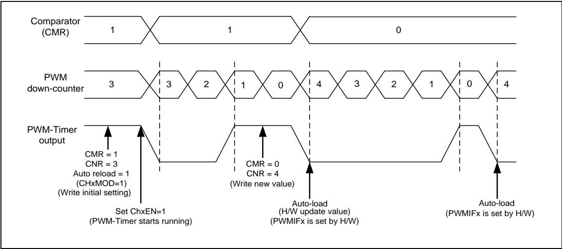
Figure 5-54 PWM Timer Operation Timing
