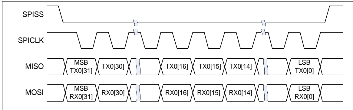
Figure 5-125 32-bit in One Transaction
