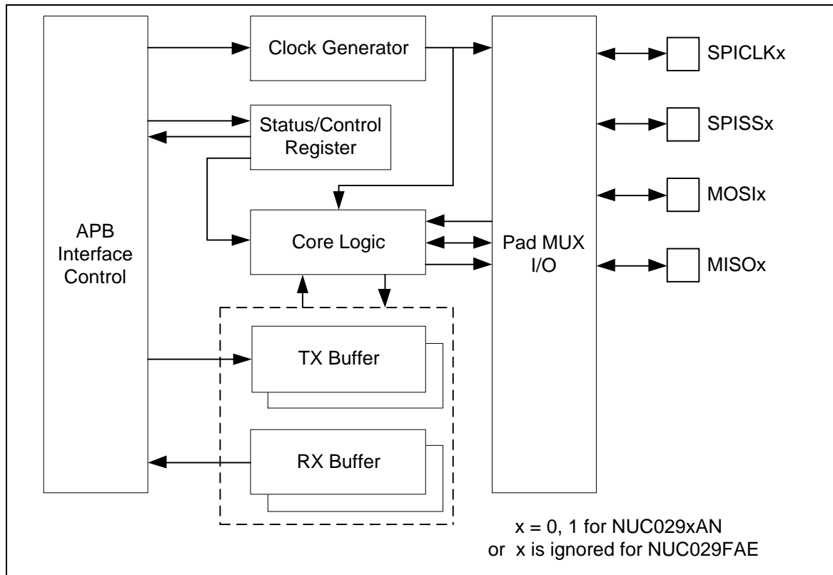
Figure 5-122 SPI Block Diagram
