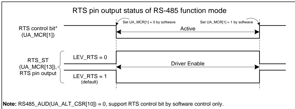
Figure 5-101 RS-485 RTS Driving Level with Software Control
