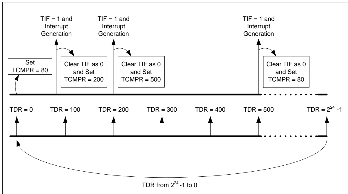
Figure 5-43 Continuous Counting Mode
