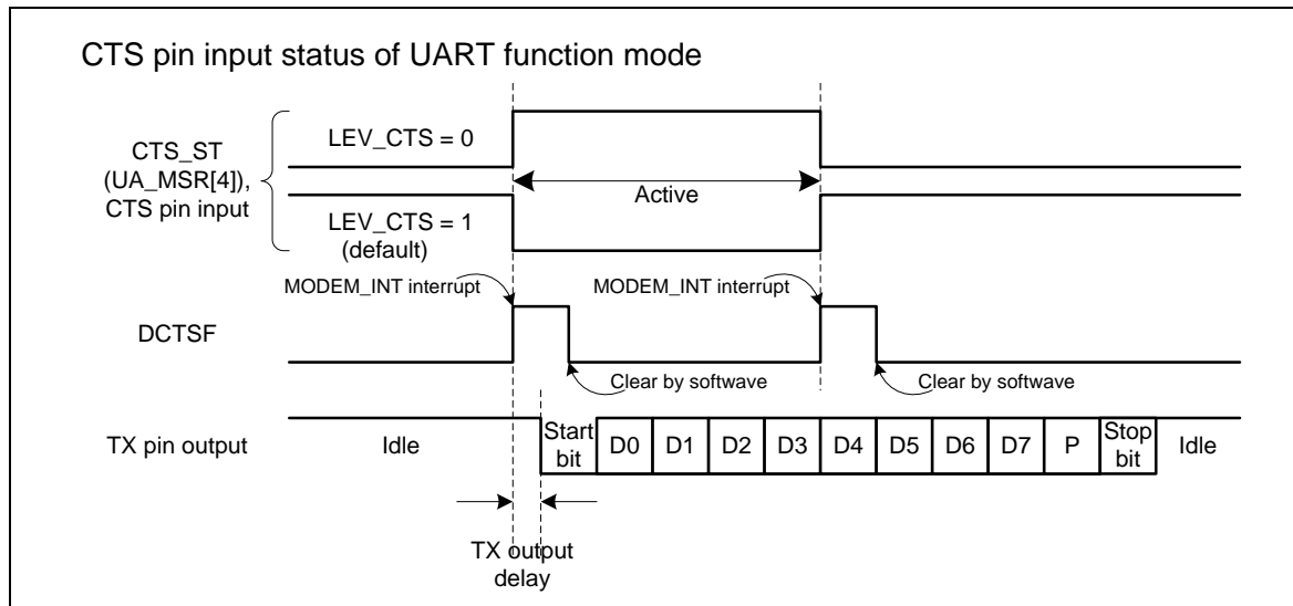
Figure 5-95 UART CTS Auto Flow Control Enabled
