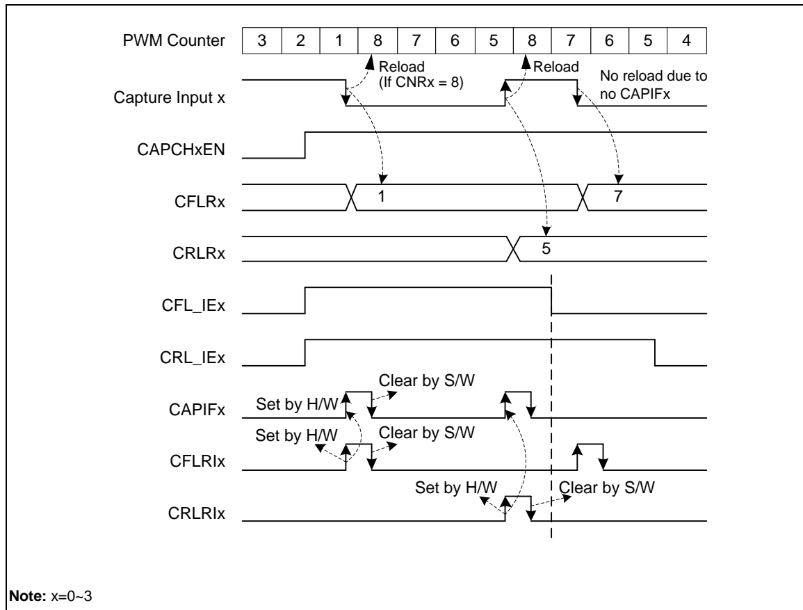
Figure 5-64 Capture Operation Timing
