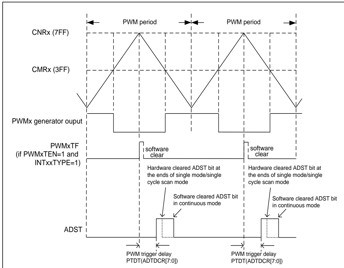
Figure 5-63 PWM Trigger ADC Start-of-Conversion in Center-aligned Type
