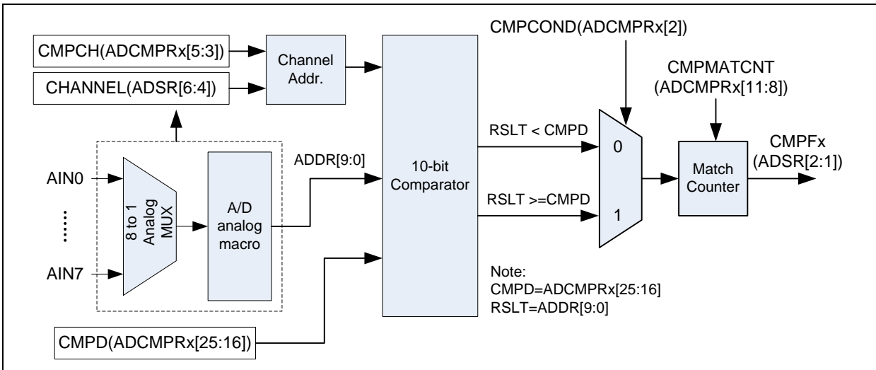
Figure 5-142 A/D Conversion Result Monitor Logic Diagram for NUC029FAE
