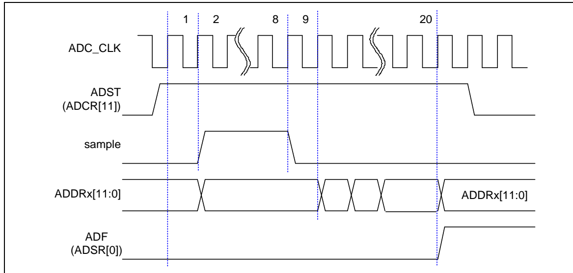
Figure 5-137 Single Mode Conversion Timing Diagram for NUC029xAN
