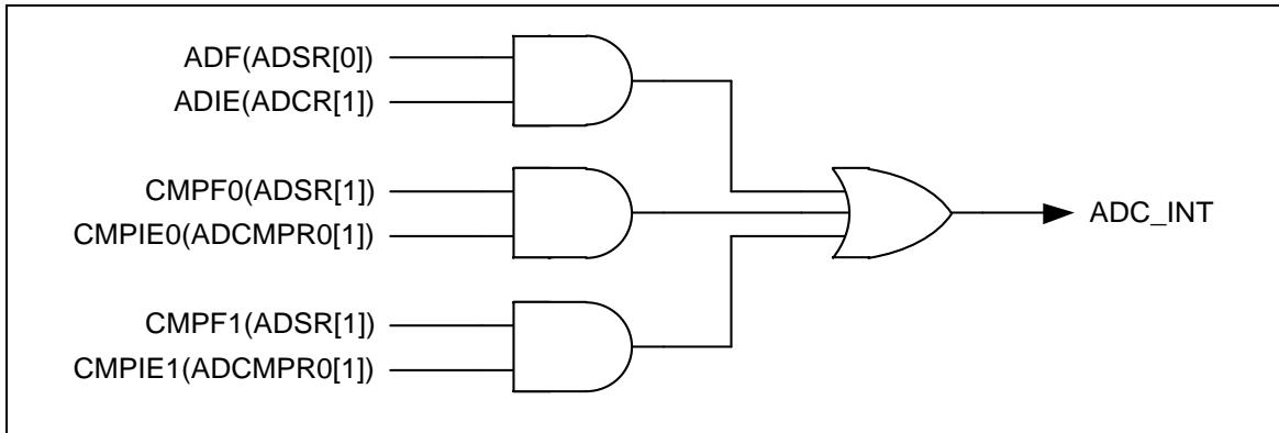
Figure 5-143 A/D Controller Interrupt
