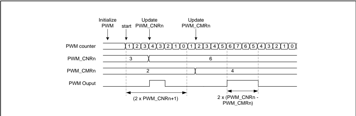
Figure 5-77 Center-aligned Mode Operation Timing
