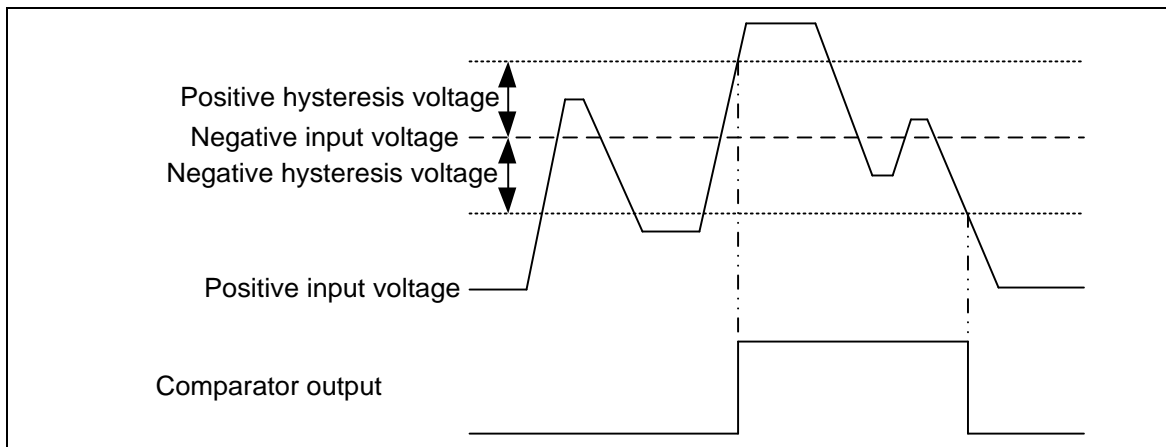
Figure 5-152 Comparator Hysteresis Function
