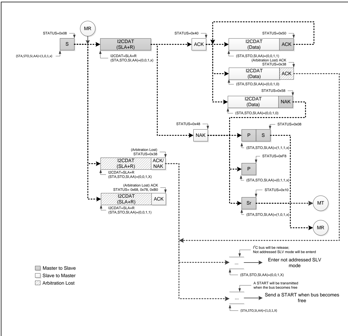
Figure 5-117 Master Receiver Mode Control Flow
