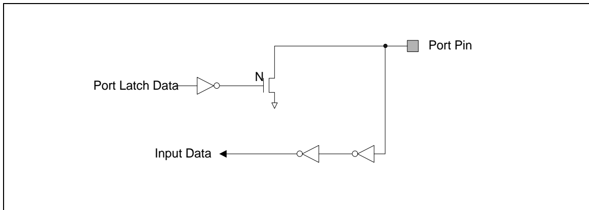
Figure 5-37 Open-Drain Output
