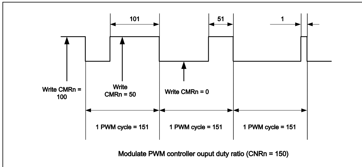
Figure 5-81 PWM Controller Output Duty Ratio
