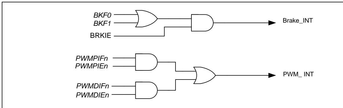
Figure 5-84 Motor Control PWM Architecture
