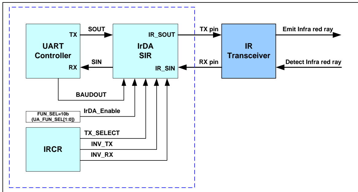
Figure 5-98 IrDA Control Block Diagram
