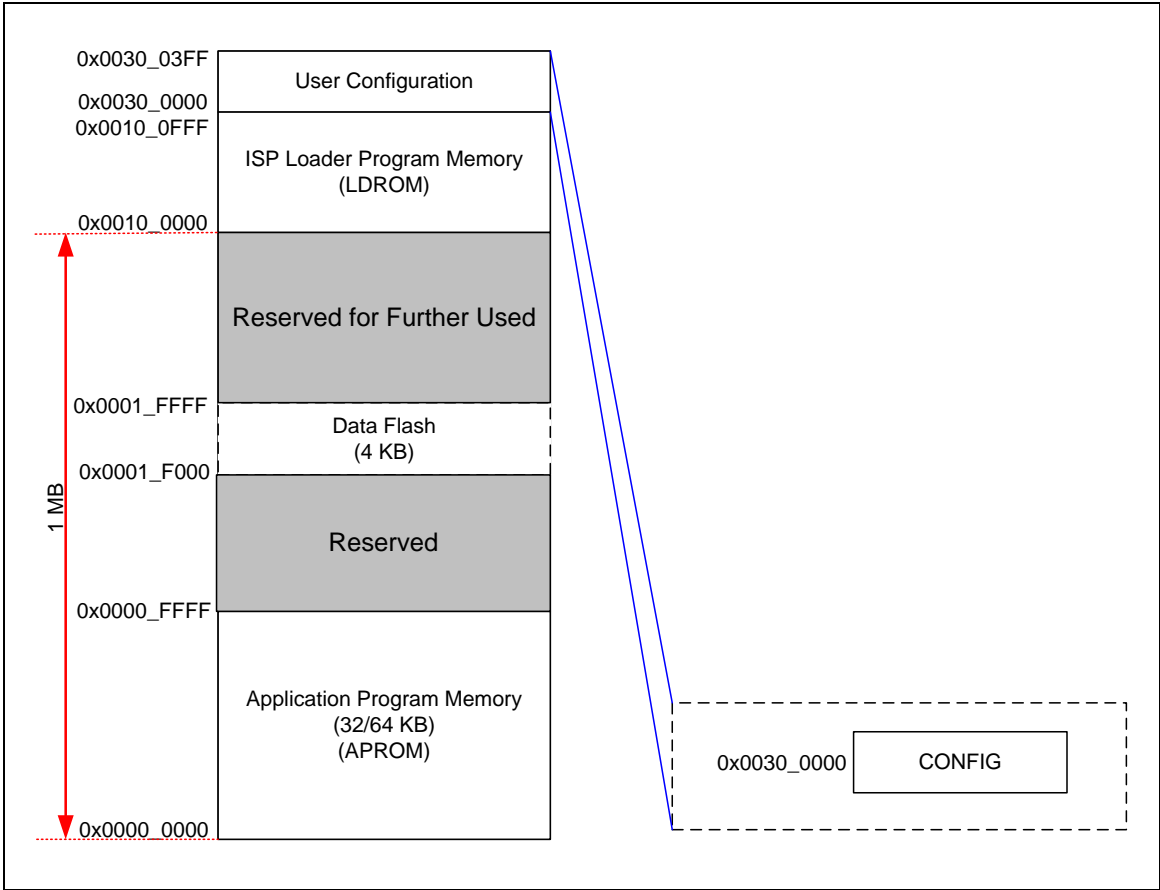
Figure 5-20 Flash Memory Organization for NUC029xAN
