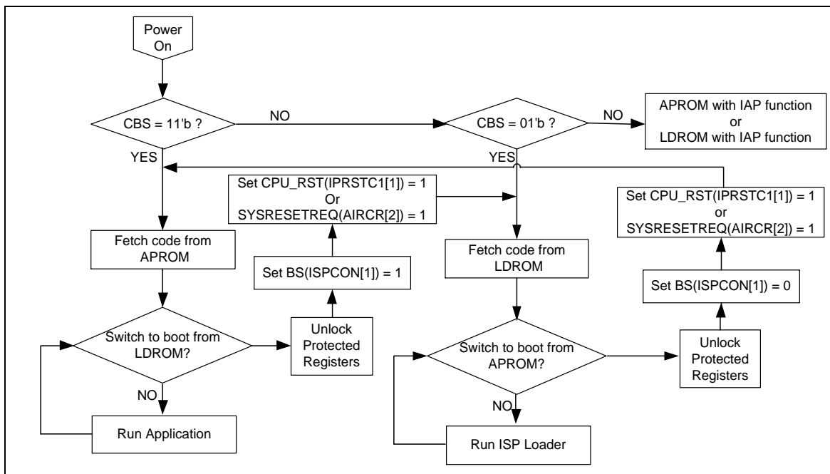
Figure 5-27 Example Flow of Boot Selection by BS Bit when CBS[0] = 1
