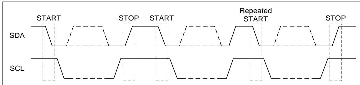
Figure 5-106 START and STOP Conditions
