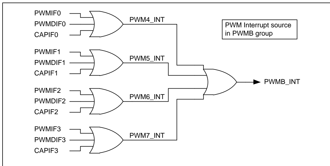
Figure 5-66 PWM Group B PWM-Timer Interrupt Architecture Diagram
