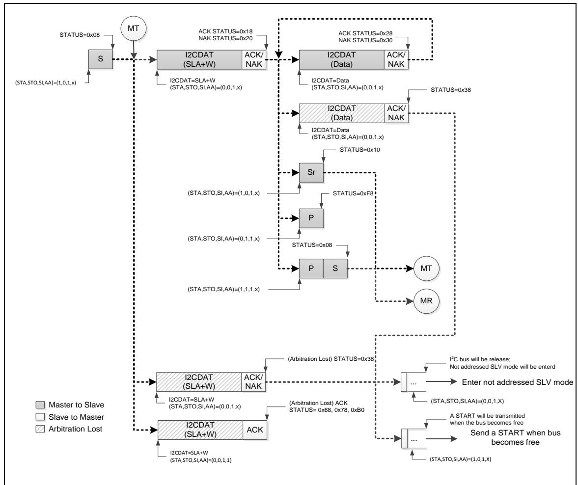
Figure 5-116 Master Transmitter Mode Control Flow
