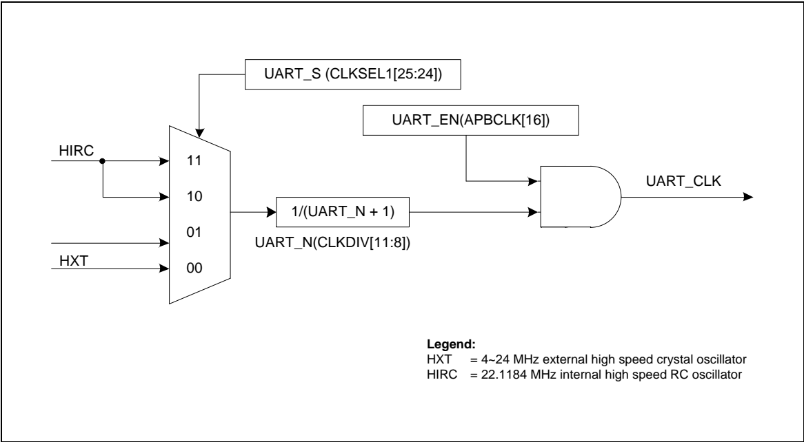
Figure 5-92 UART Controller Clock Control for NUC029FAE
