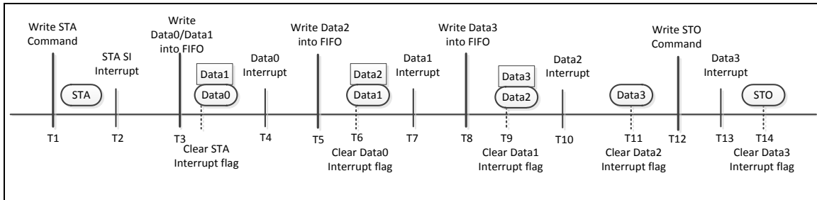
Figure 5-111 Timing of Two Level FIFO Transmit in Master Write
