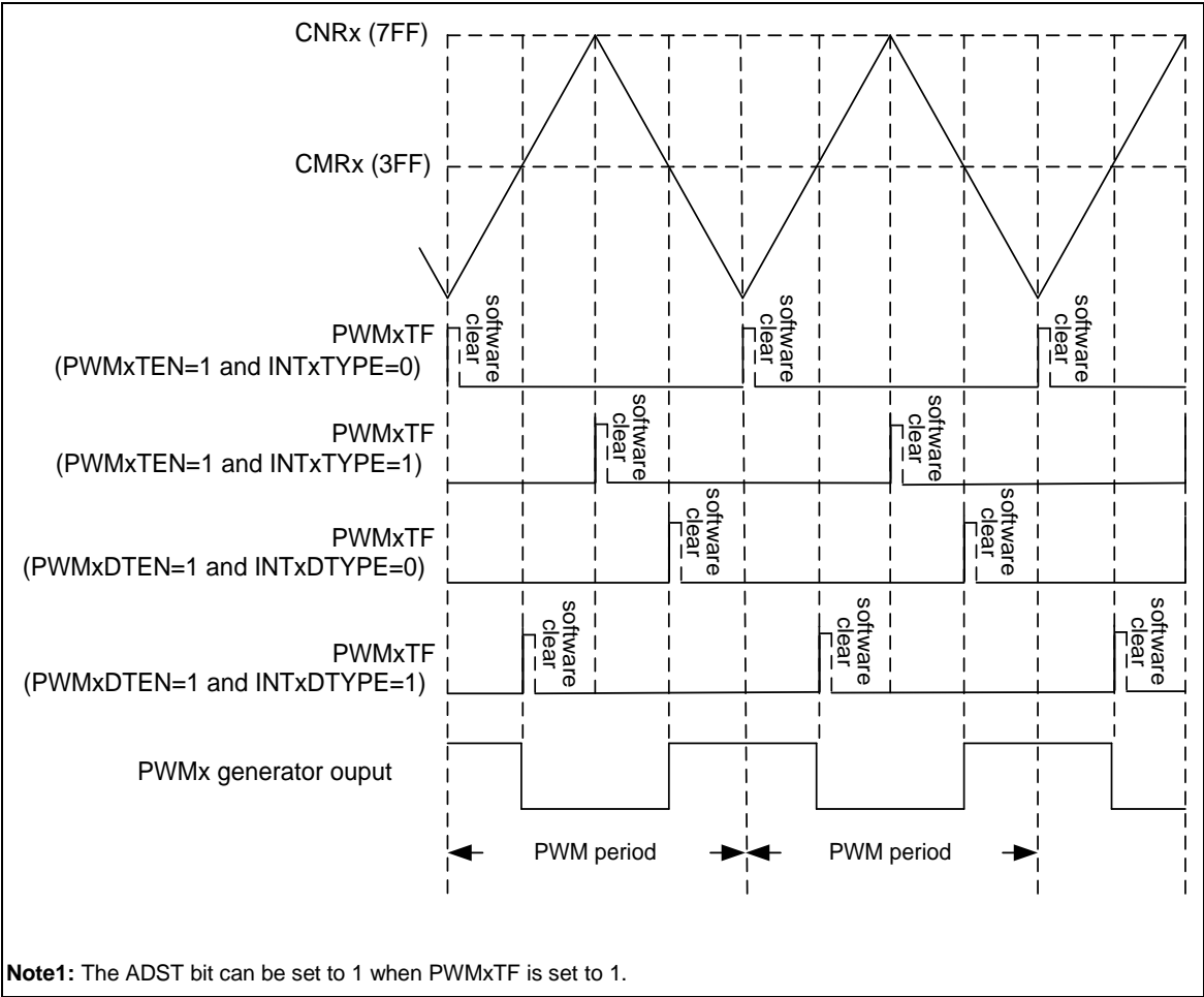
Figure 5-61 PWM Trigger ADC Flag (PWMxTF) in Center-aligned Type Timing Waveform
