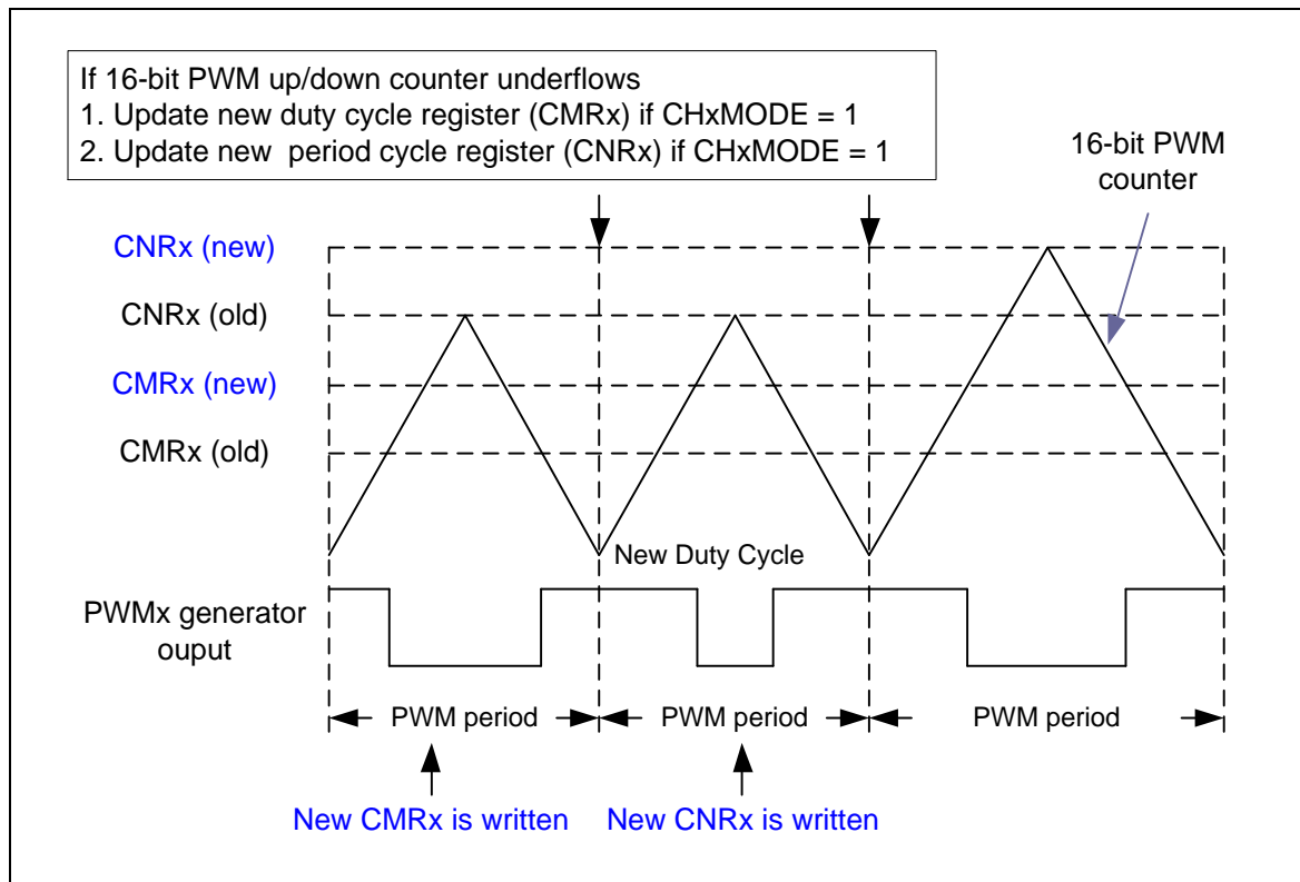
Figure 5-56 Center-aligned type Output Waveform
