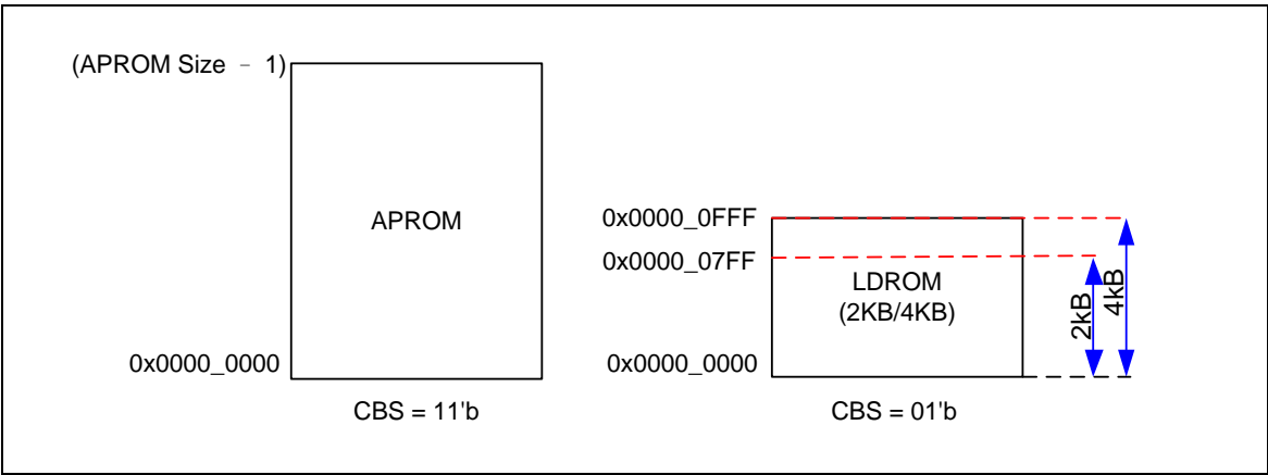
Figure 5-25 Program Executing Range for Booting from APROM and LDROM
