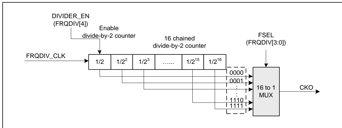
Figure 5-12 NuMicro® NUC029xAN Frequency Divider Block Diagram
