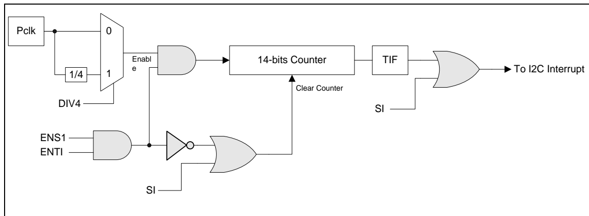
Figure 5-114 I 2 C Time-out Count Block Diagram
