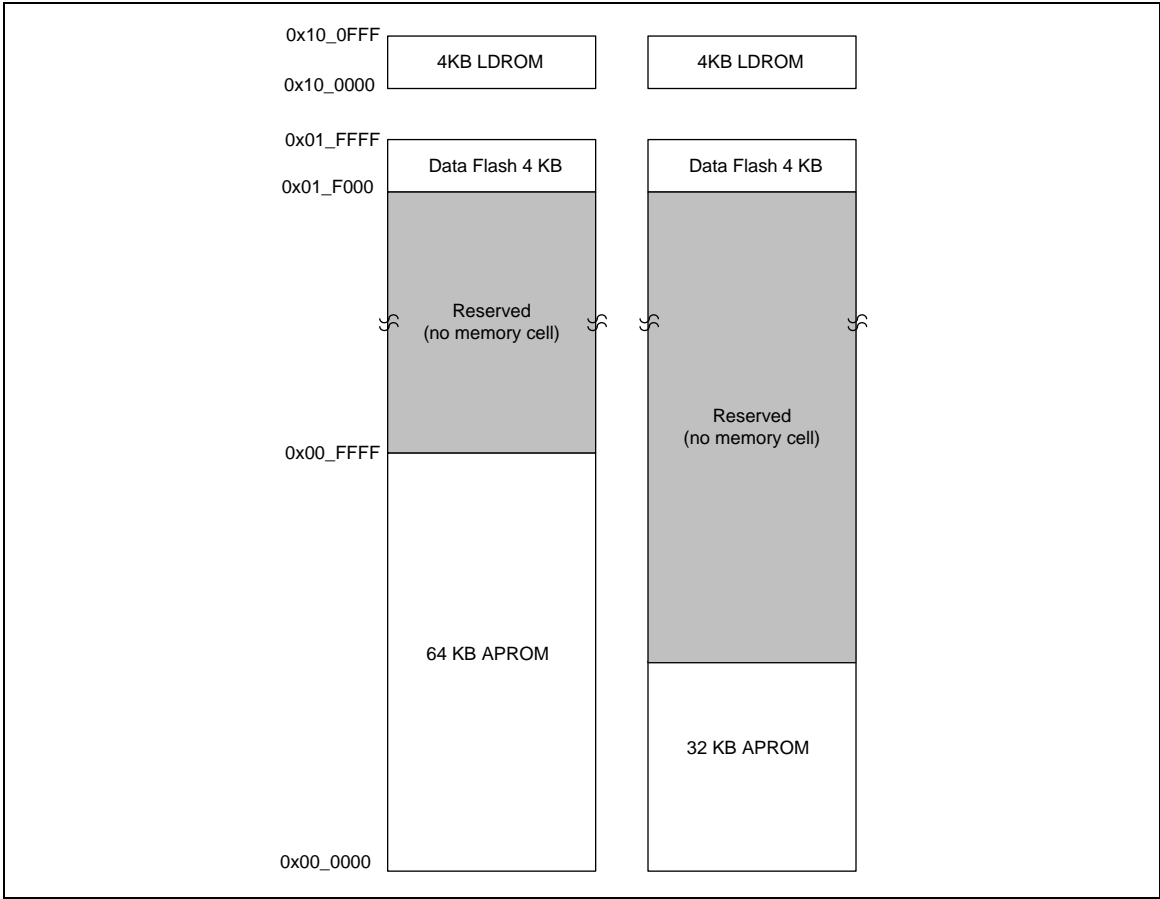
Figure 5-22 Flash Memory Structure for NUC029xAN
