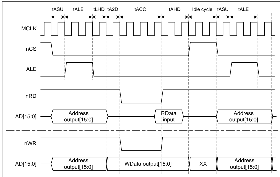
Figure 5-35 EBI Timing Control Waveform for Insert Idle Cycle
