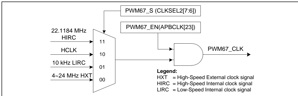
Figure 5-51 PWM Generator 6 Clock Source Control
