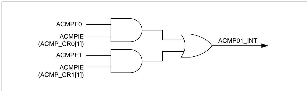
Figure 5-151 Analog Comparator Controller Interrupt Sources for NUC029FAE
