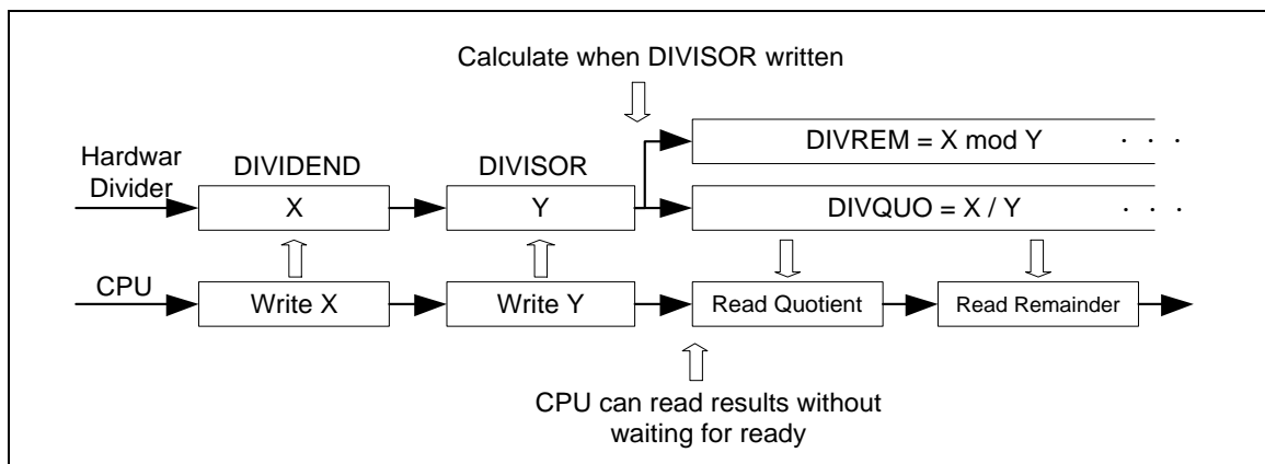
Figure 5-154 Hardware Divider Operation Flow
