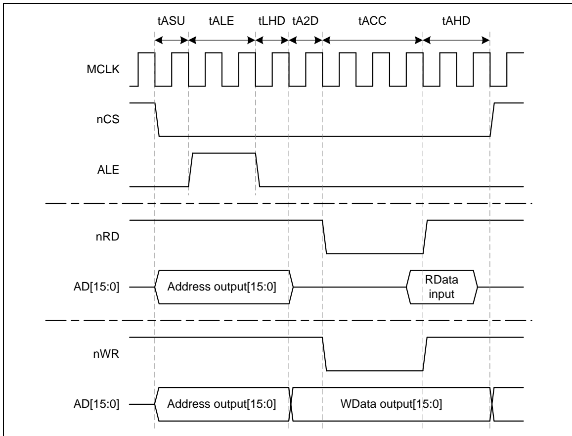
Figure 5-33 EBI Timing Control Waveform for 16-bit Data Width
