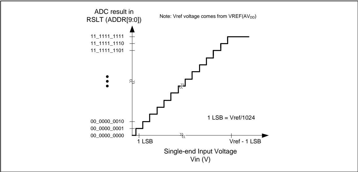
Figure 5-146 Conversion Result Mapping Diagram of ADC Single-end Input
