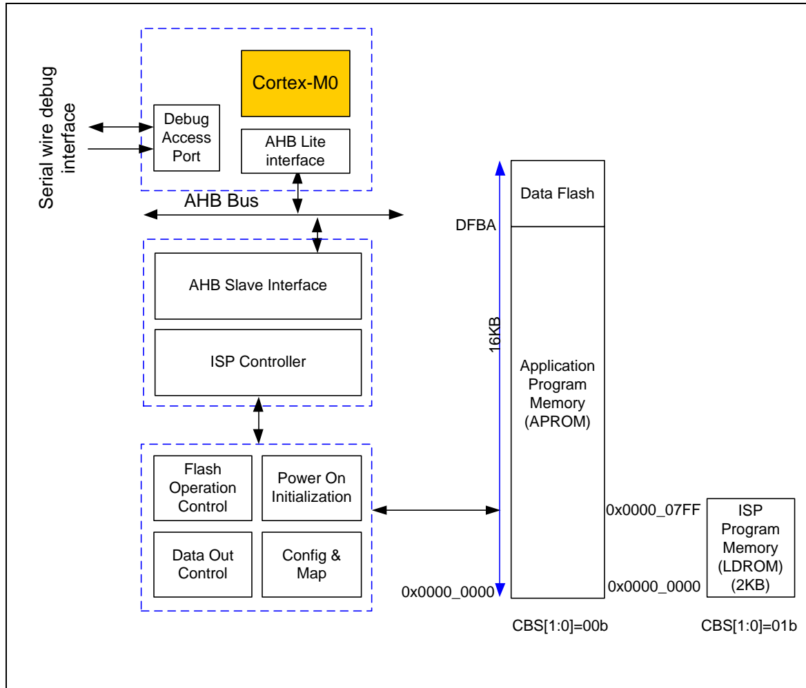
Figure 5-19 Flash Memory Control Block Diagram for NUC029FAE
