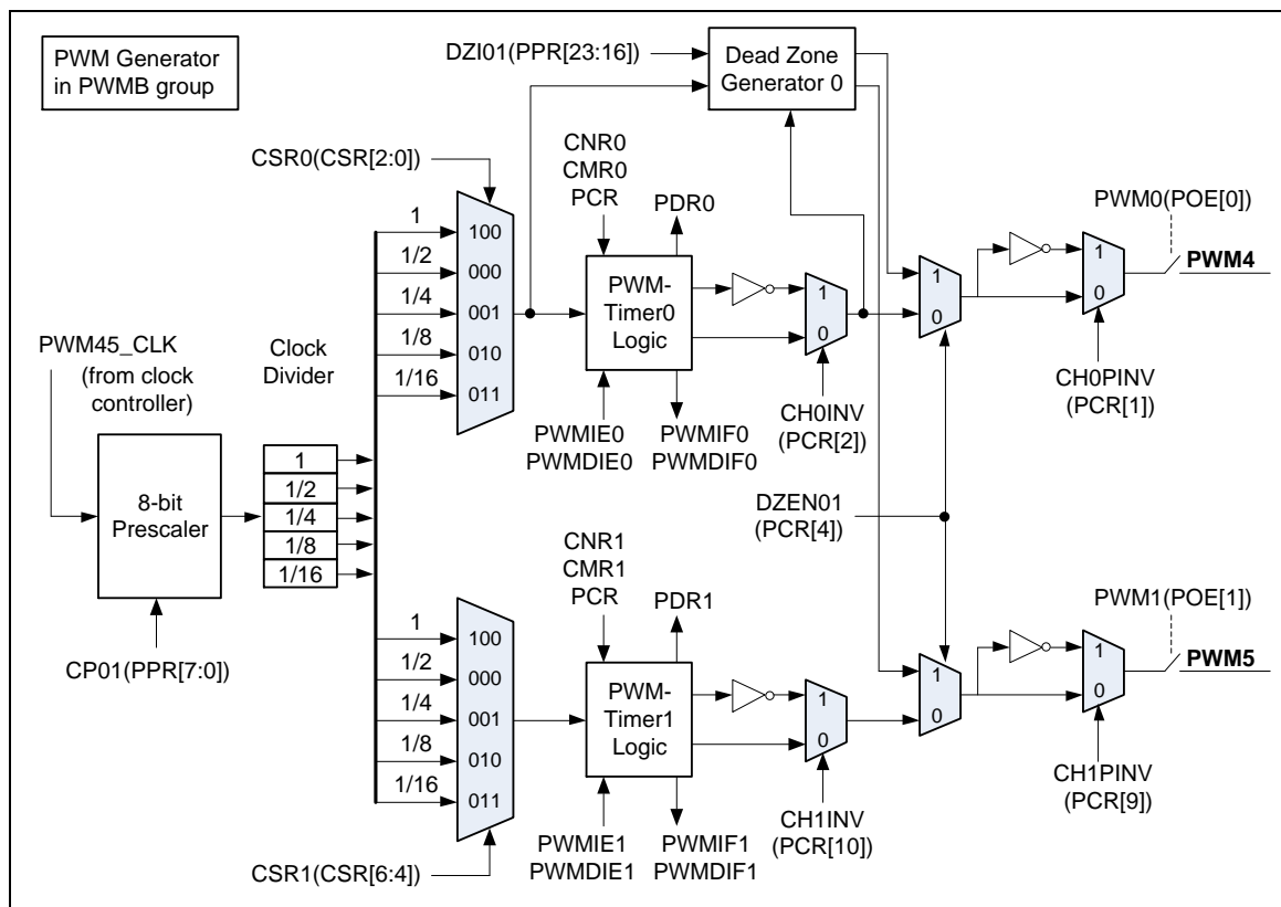
Figure 5-50 PWM Generator 4 Architecture Diagram
