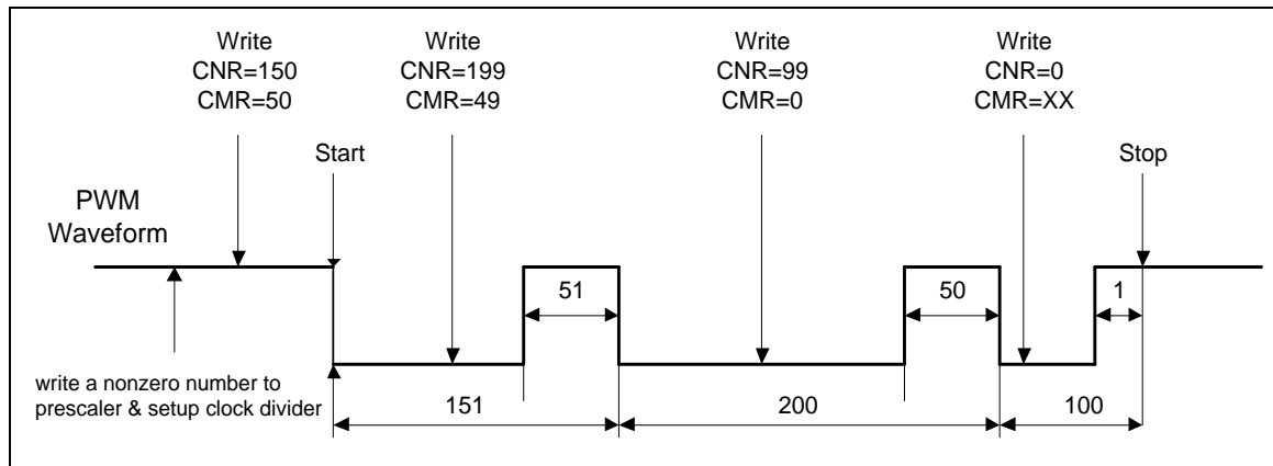
Figure 5-58 PWM Double Buffering Illustration
