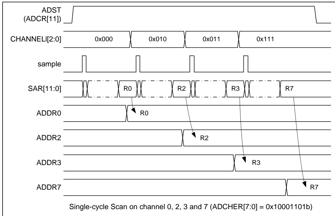
Figure 5-139 Single-Cycle Scan Mode on Enabled Channels Timing Diagram
