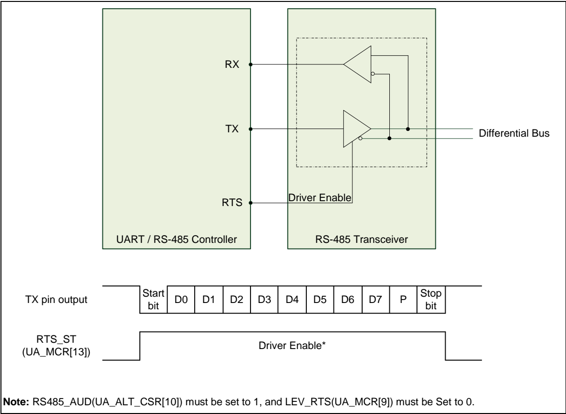
Figure 5-102 Structure of RS-485 Frame
