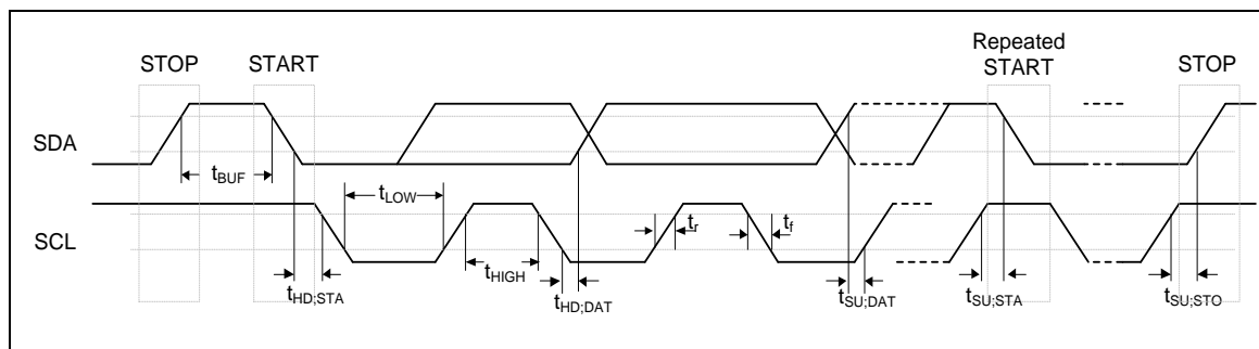
Figure 5-104 I 2 C Bus Timing
