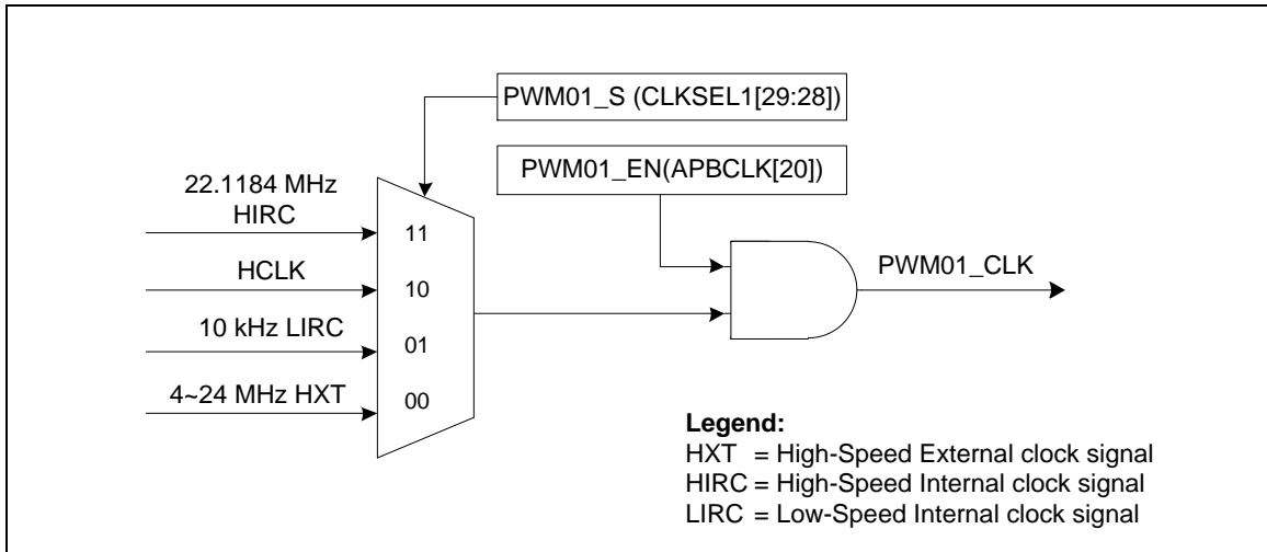
Figure 5-45 PWM Generator 0 Clock Source Control
