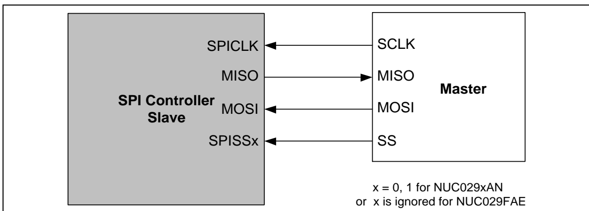
Figure 5-124 SPI Slave Mode Application Block Diagram
