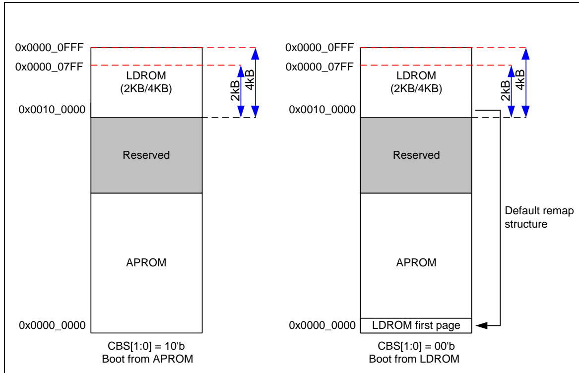
Figure 5-26 Executable Range of Code with IAP Function Enabled
