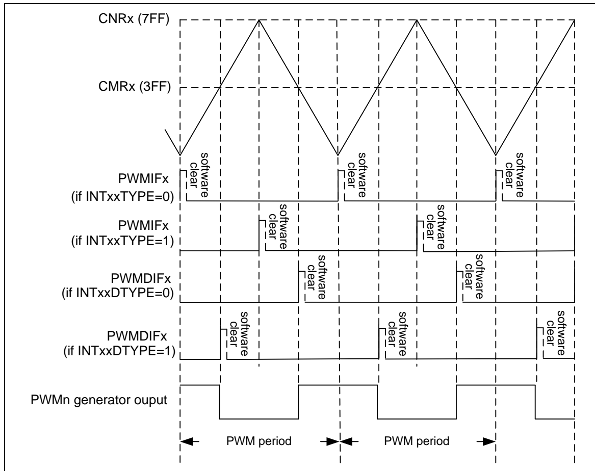
Figure 5-57 PWM Center-aligned Interrupt Generate Timing Waveform
