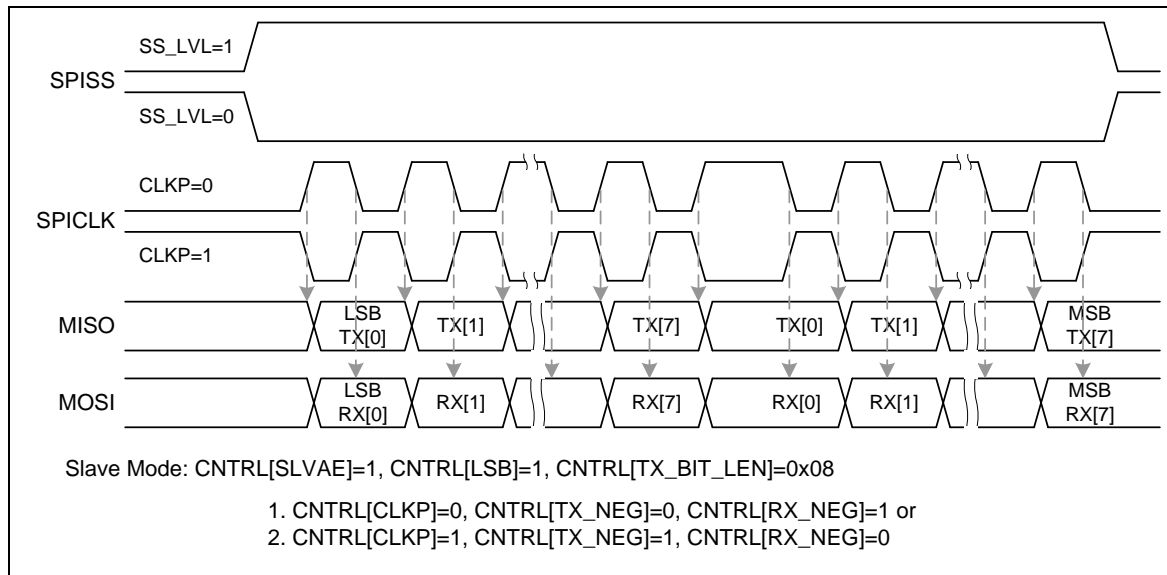
Figure 5-132 SPI Timing in Slave Mode (Alternate Phase of SPICLK)
