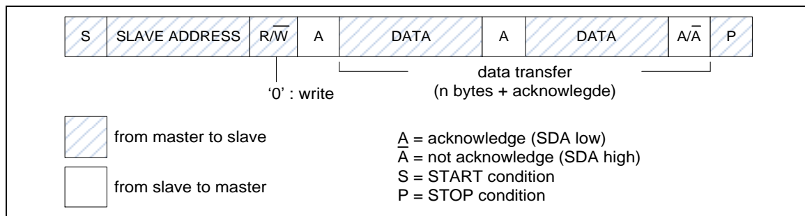
Figure 5-109 Master Transmits Data to Slave
