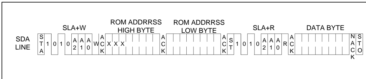
Figure 5-120 EEPROM Random Read
