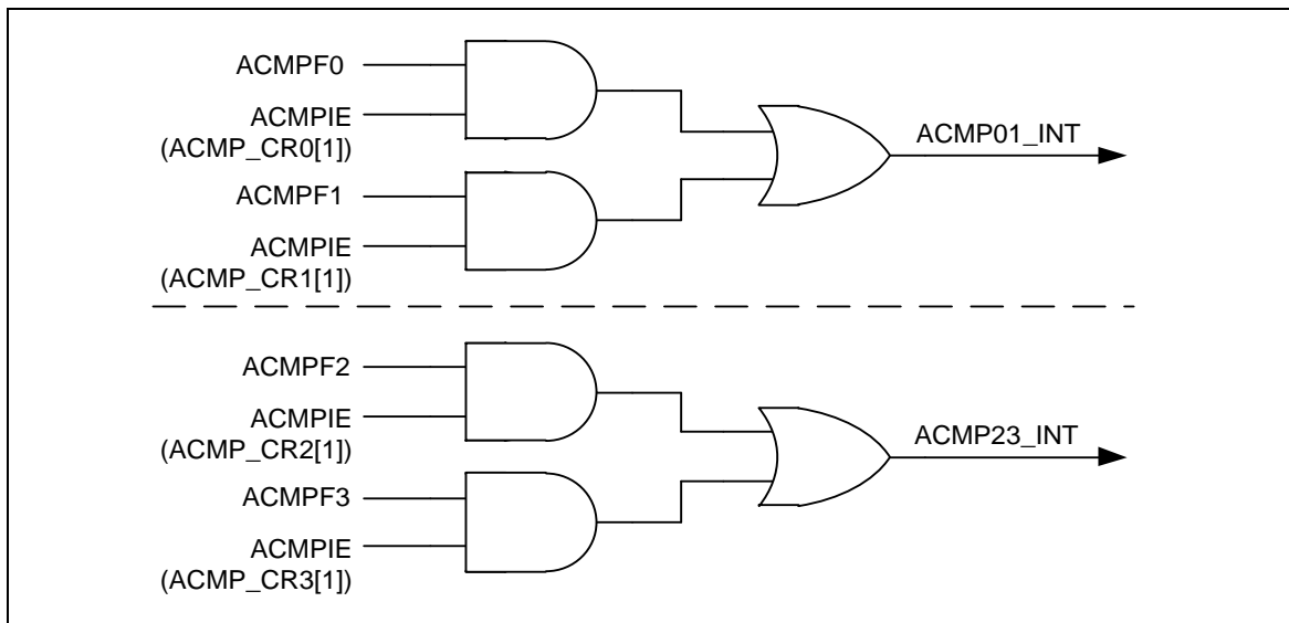
Figure 5-150 Analog Comparator Controller Interrupt Sources for NUC029xAN
