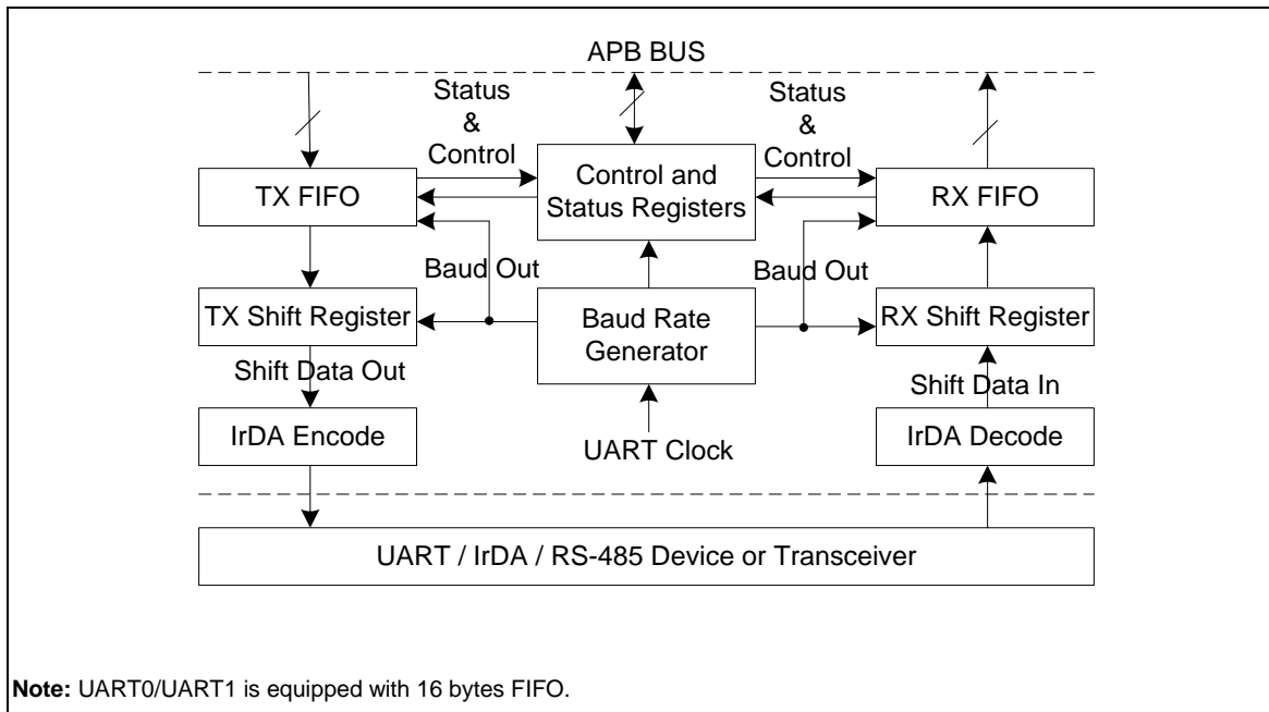
Figure 5-93 UART Controller Block Diagram
