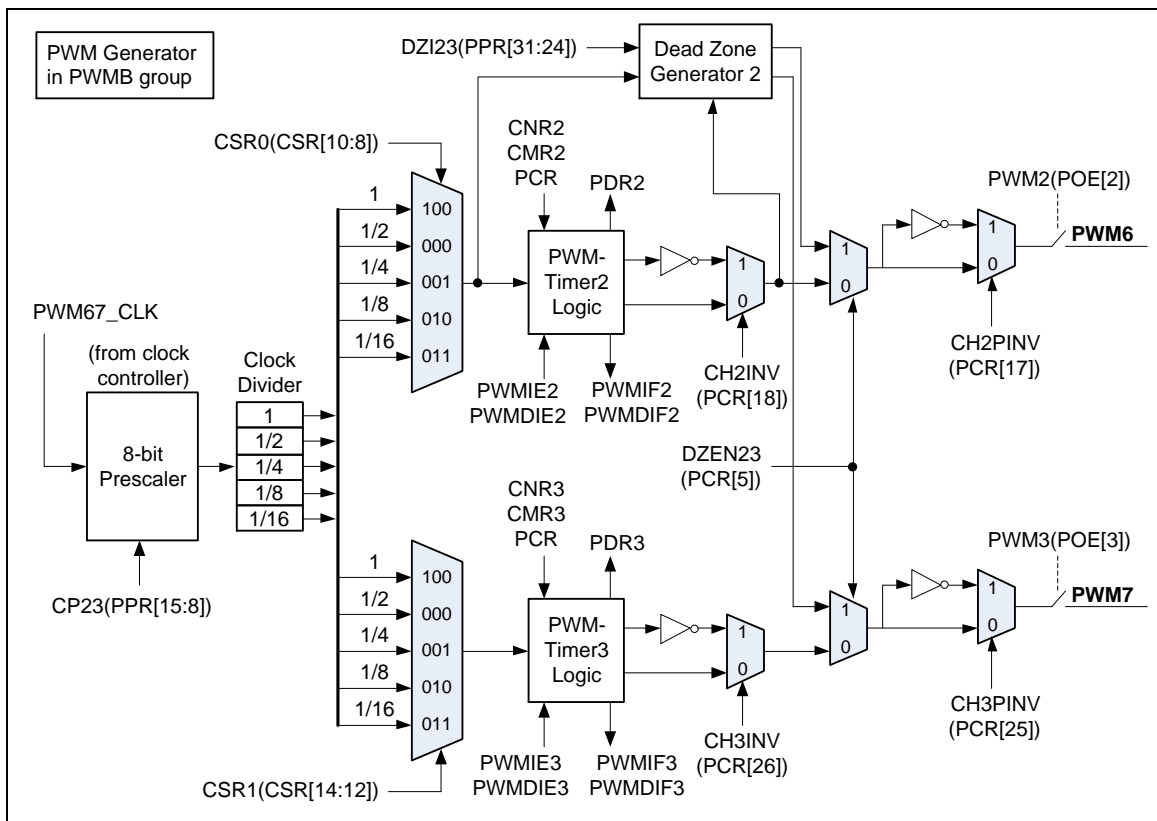
Figure 5-52 PWM Generator 6 Architecture Diagram
