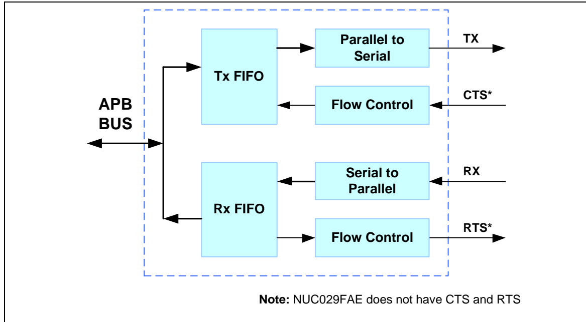
Figure 5-94 Auto Flow Control Block Diagram
