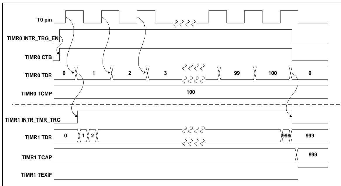
Figure 5-44 Inter-Timer Trigger Capture Timing
