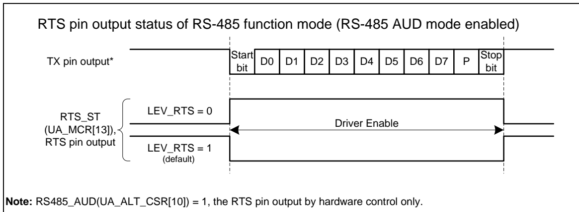
Figure 5-100 RS-485 RTS Driving Level in Auto Direction Mode
