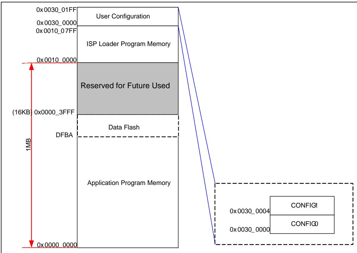
Figure 5-21 Flash Memory Organization for NUC029FAE
