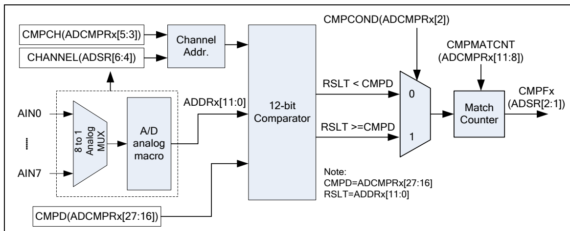
Figure 5-141 A/D Conversion Result Monitor Logic Diagram for NUC029xAN
