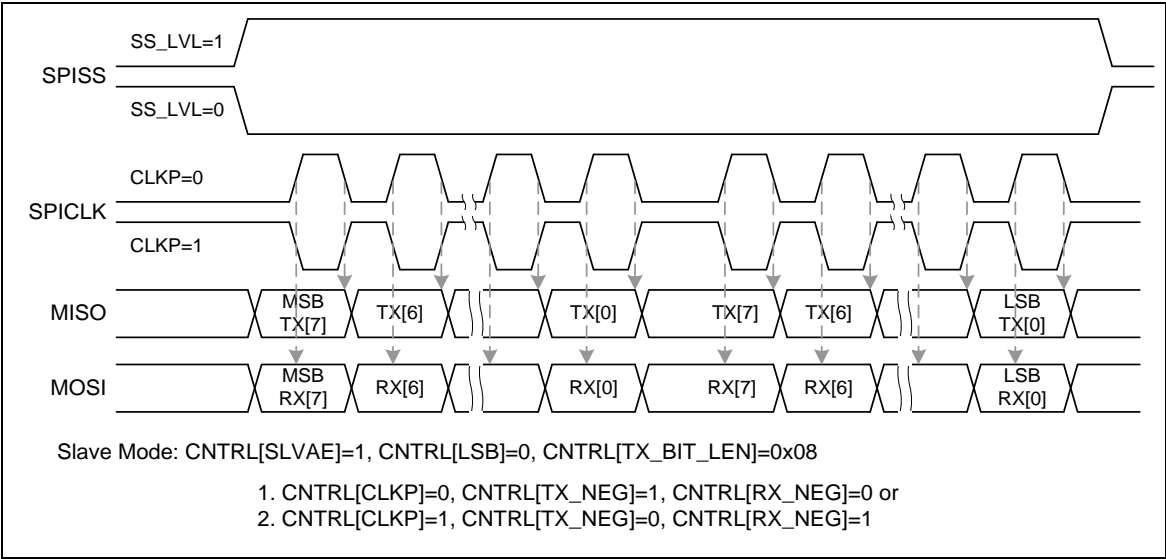
Figure 5-131 SPI Timing in Slave Mode
