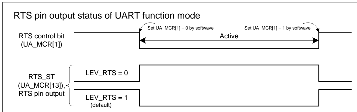
Figure 5-97 UART RTS Flow with Software Control
