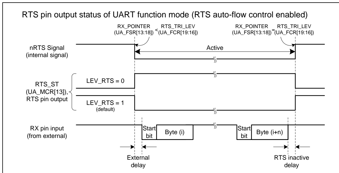
Figure 5-96 UART RTS Auto Flow Control Enabled
