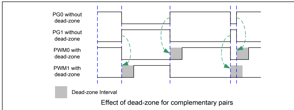
Figure 5-82 Dead-zone Insertion
