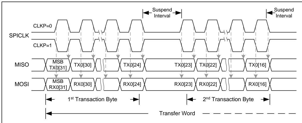
Figure 5-127 Timing Waveform for Byte Suspend
