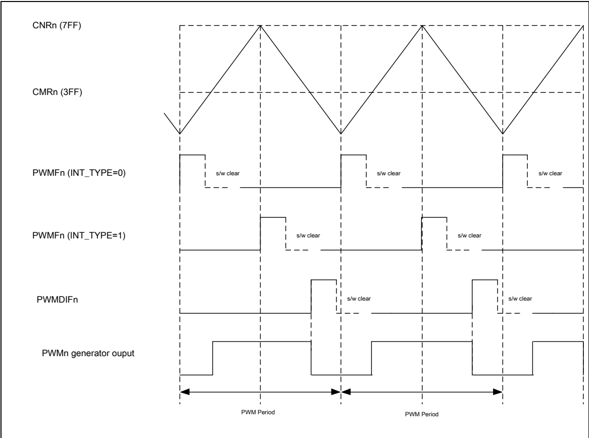
Figure 5-78 PWM Center-aligned Waveform Output
