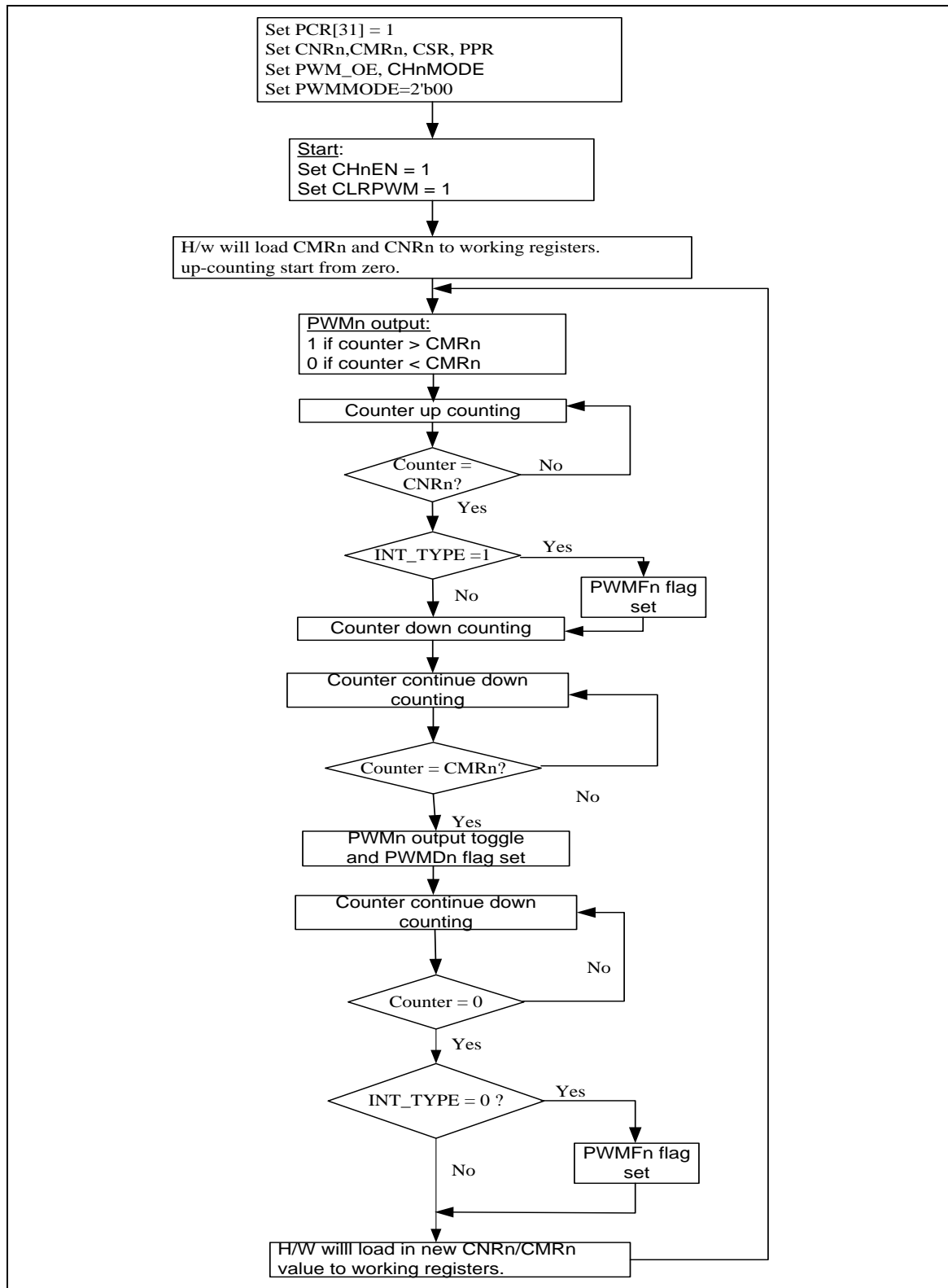
Figure 5-79 Center-aligned Flow Diagram ( INT\_TYPE = 0 )
