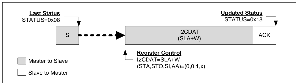
Figure 5-115 Control I 2 C Bus according to Current I 2 C Status
