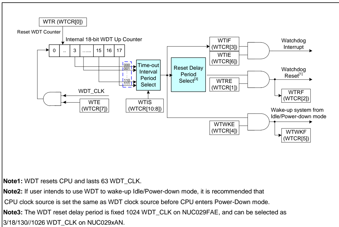
Figure 5-86 Watchdog Timer Block Diagram
