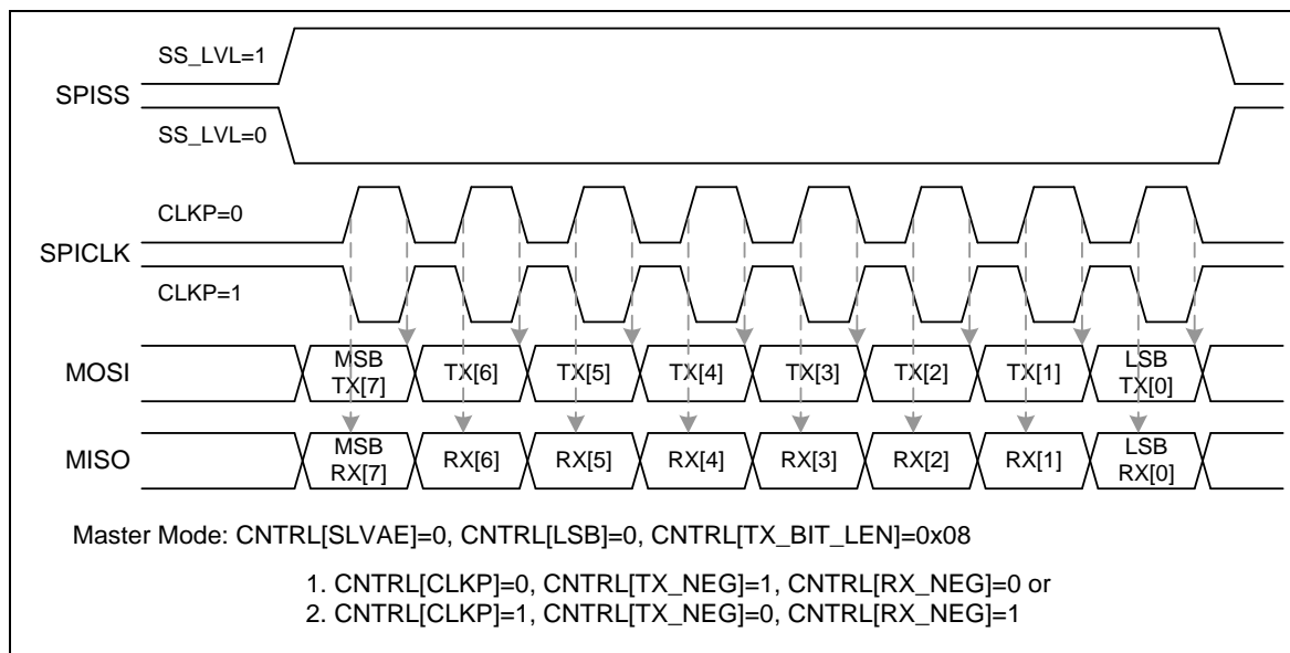
Figure 5-129 SPI Timing in Master Mode
