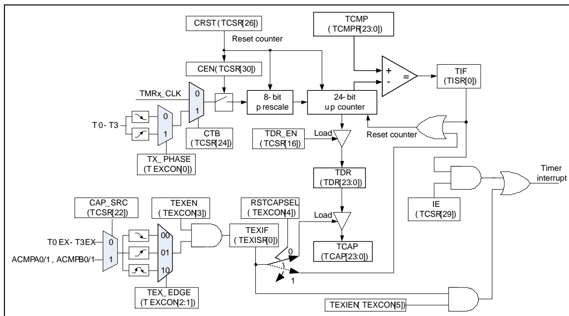
Figure 5-39 Timer Controller Block Diagram for NUC029xAN
