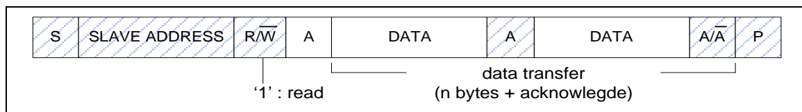
Figure 5-110 Master Reads Data from Slave
