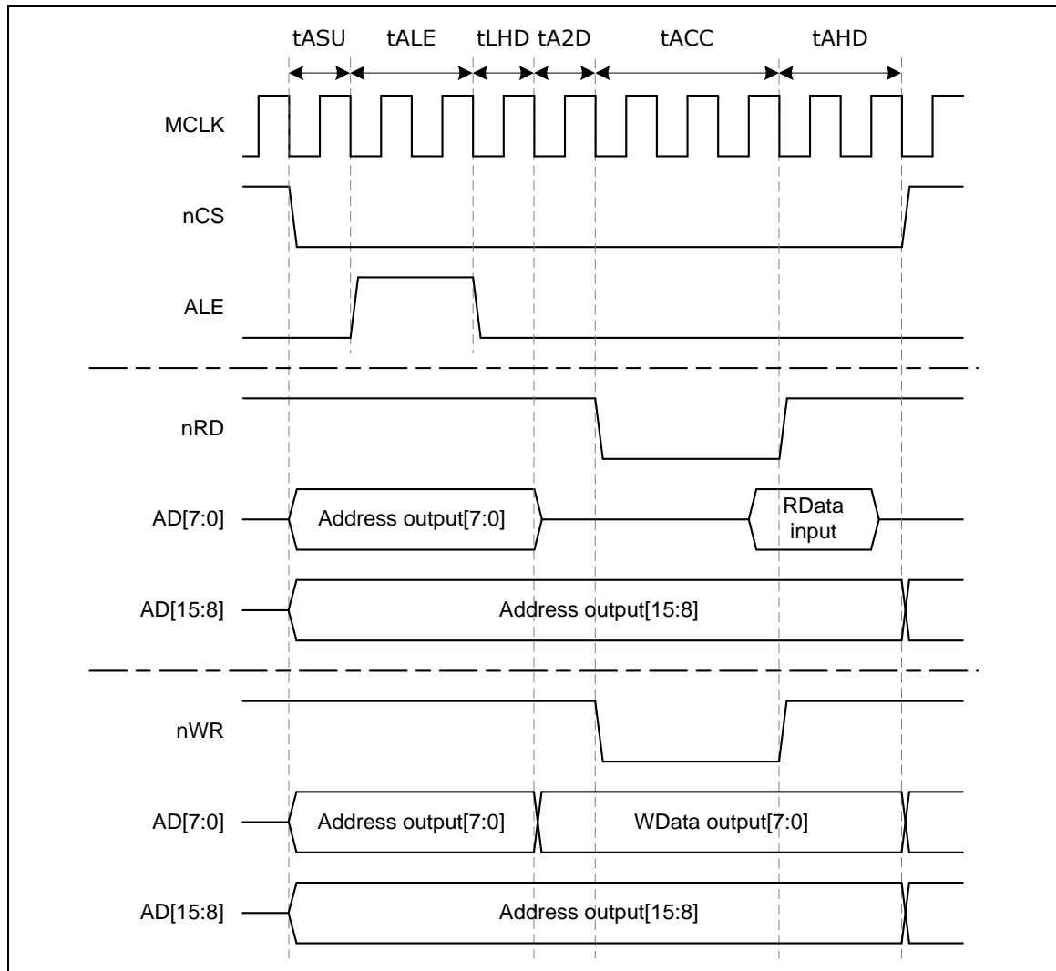
Figure 5-34 EBI Timing Control Waveform for 8-bit Data Width
