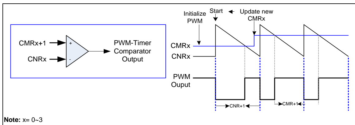
Figure 5-53 Legend of Internal Comparator Output of PWM-Timer
