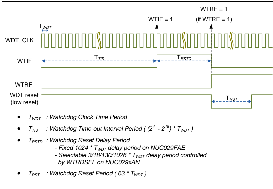
Figure 5-87 Watchdog Timer Time-out Interval and Reset Period Timing
