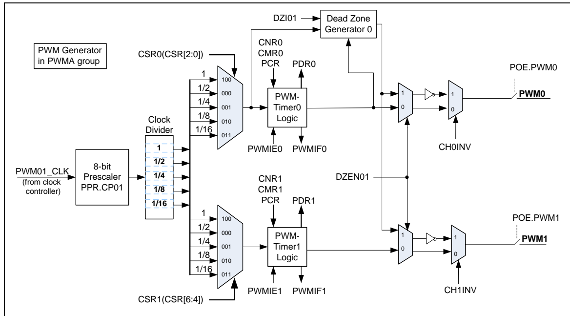
Figure 5-68 PWM Generator 0 Architecture Diagram
