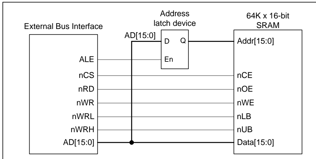
Figure 5-31 Connection of 16-bit EBI Data Width with 16-bit Device
