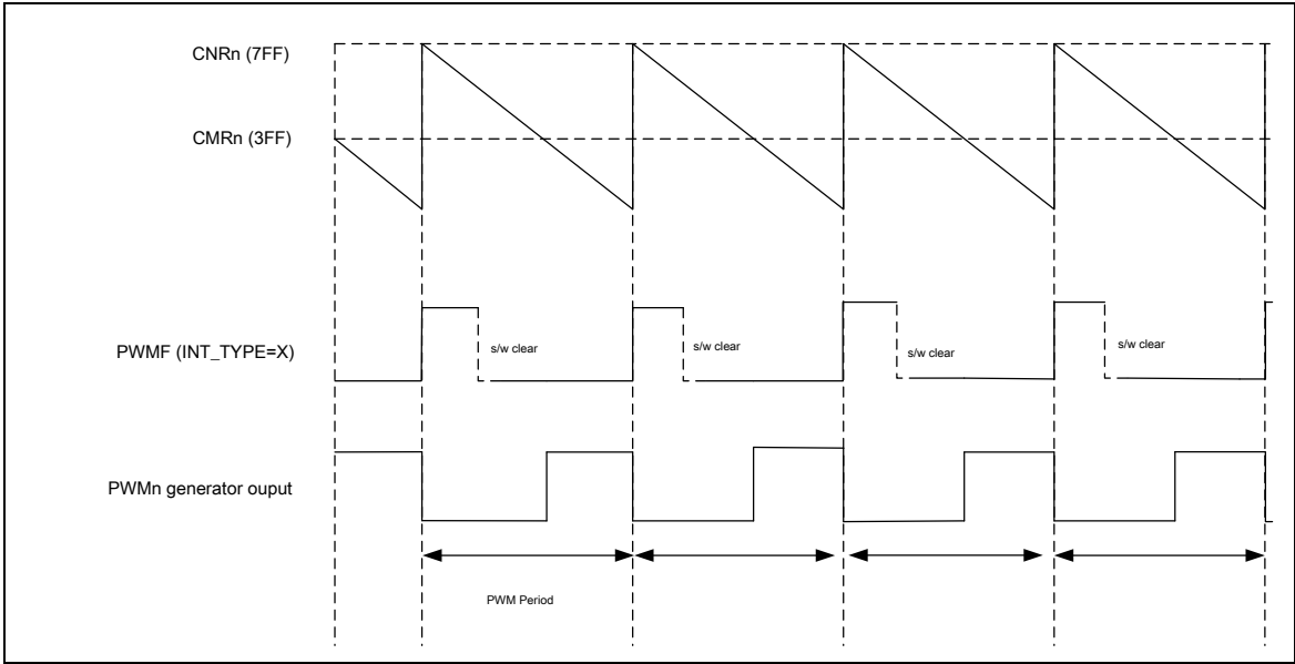
Figure 5-72 PWM Edge-aligned Waveform Output
