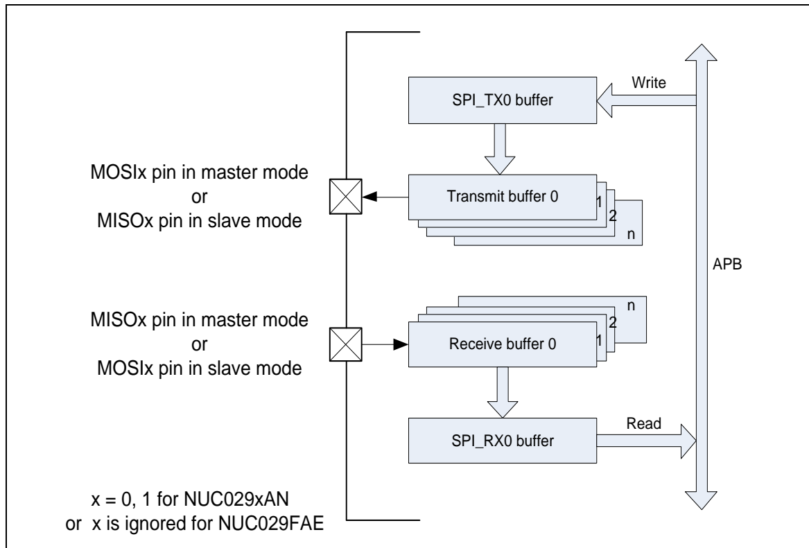
Figure 5-128 FIFO Mode Block Diagram
