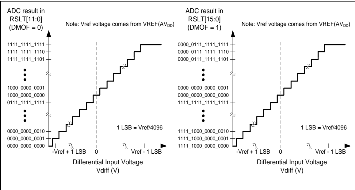
Figure 5-145 Conversion Result Mapping Diagram of ADC Differential Input
