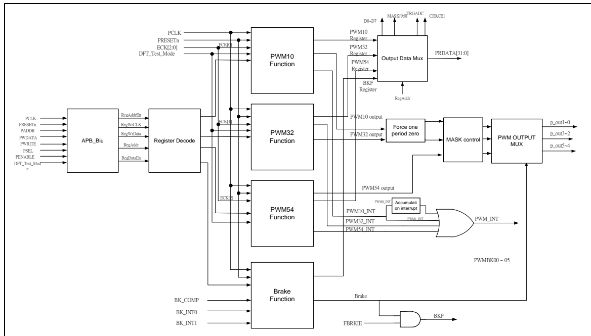
Figure 5-67 PWM Block Diagram
