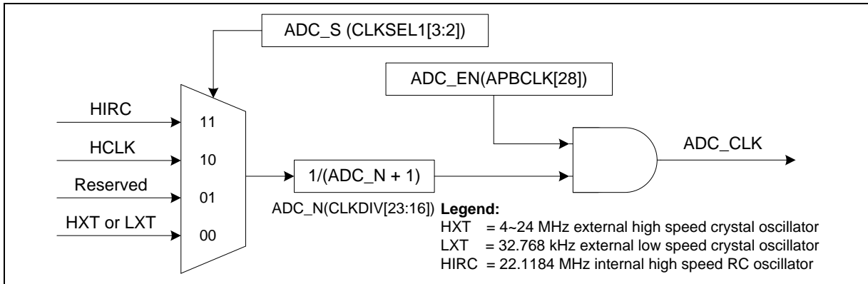
Figure 5-136 ADC Peripheral Clock Control for NUC029FAE
