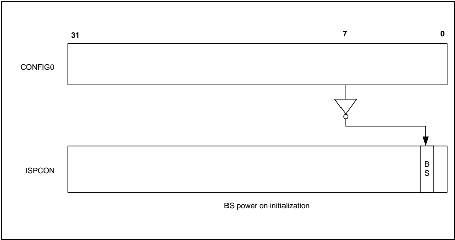
Figure 5-24 Boot Select (BS) for Power-on Action
