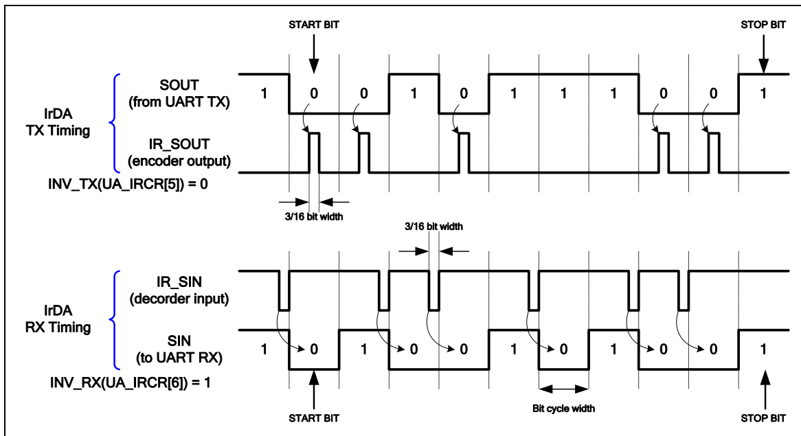
Figure 5-99 IrDA TX/RX Timing Diagram
