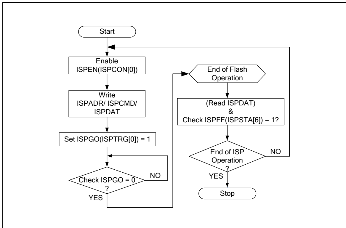
Figure 5-28 ISP Flow Example
