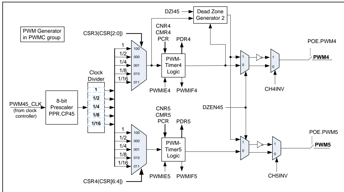
Figure 5-70 PWM Generator 4 Architecture Diagram
