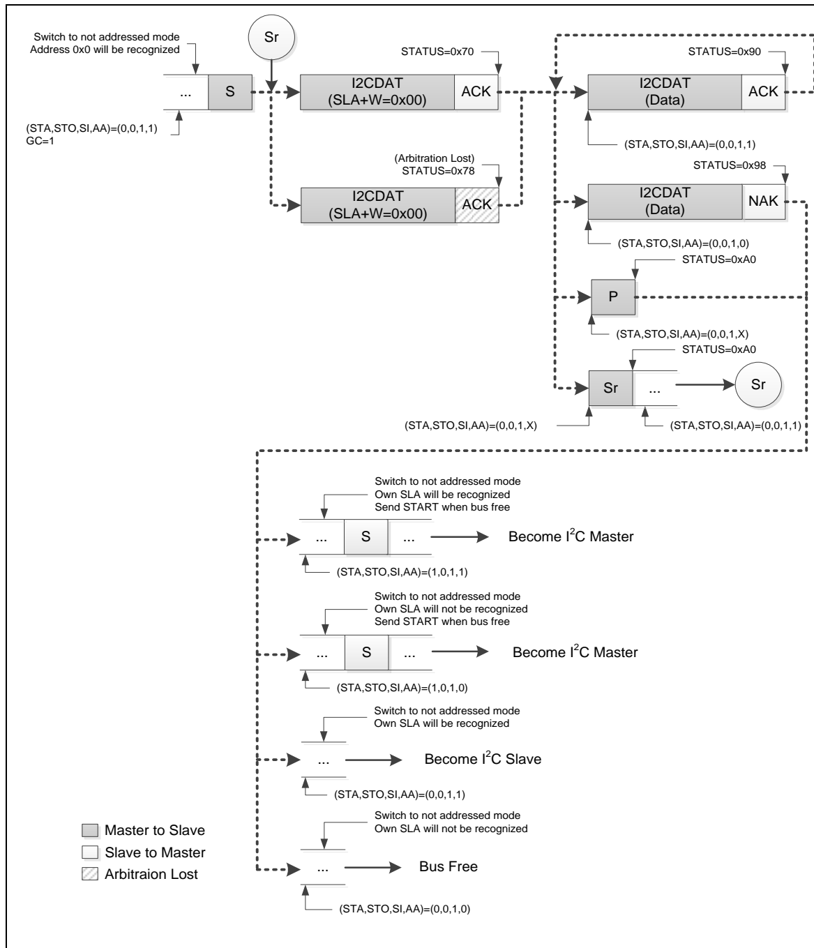
Figure 5-119 GC Mode
