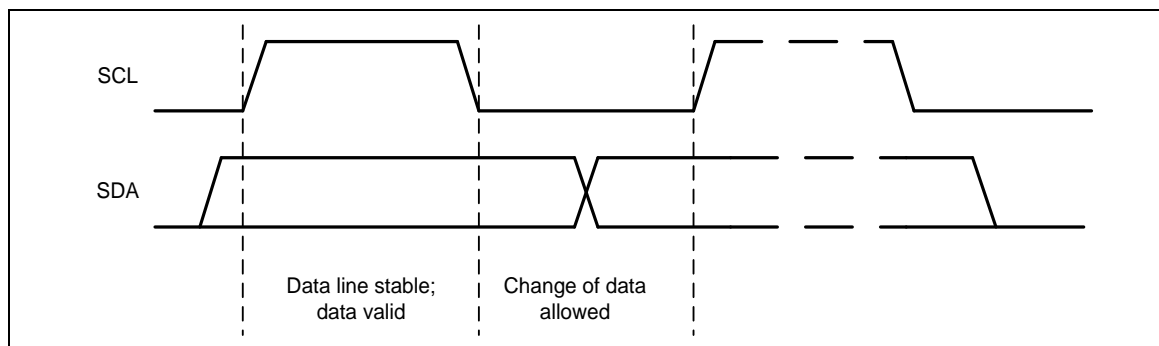
Figure 5-107 Bit Transfer on the I 2 C Bus
