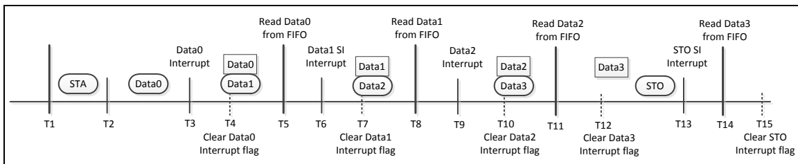
Figure 5-112 Timing of Two Level FIFO Transmit in Slave Read
