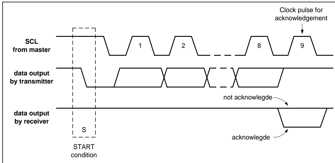
Figure 5-108 Acknowledge on the I 2 C Bus
