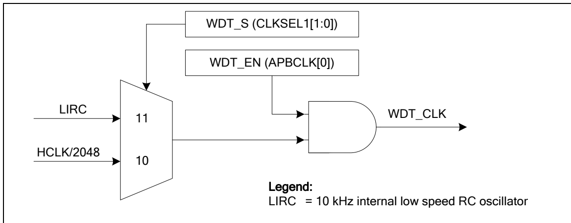
Figure 5-85 Watchdog Timer Clock Control
