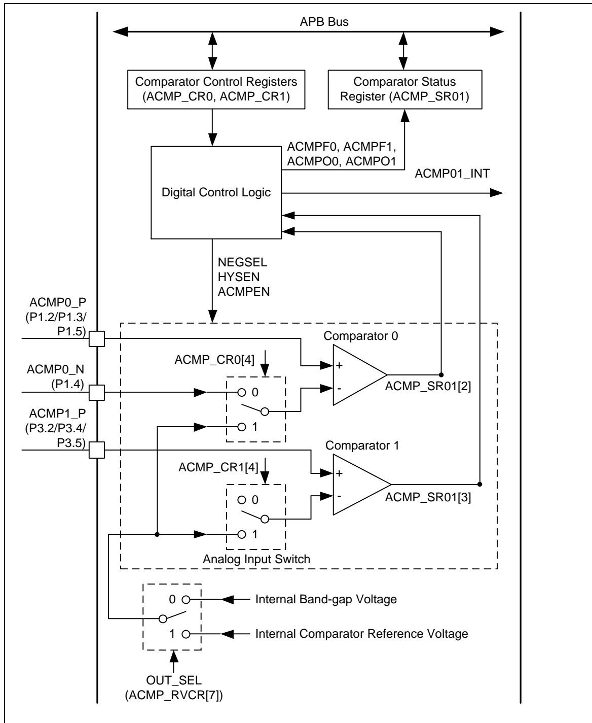
Figure 5-149 Analog Comparator Block Diagram for NUC029FAE
