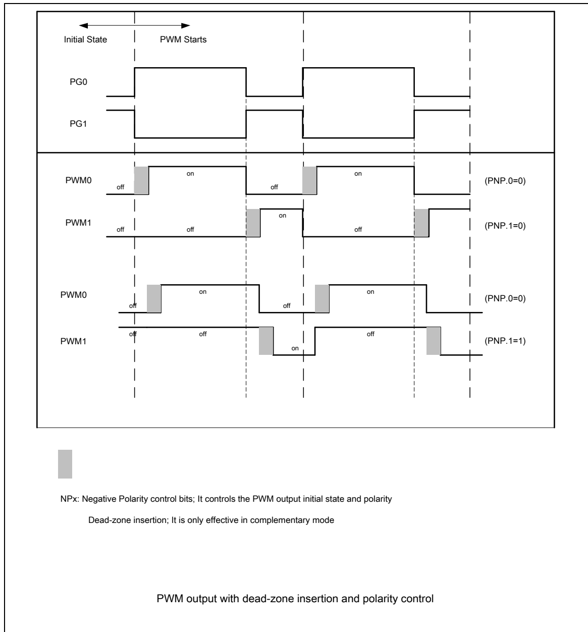
Figure 5-83 Initial State and Polarity Control with Rising Edge Dead-zone Insertion
