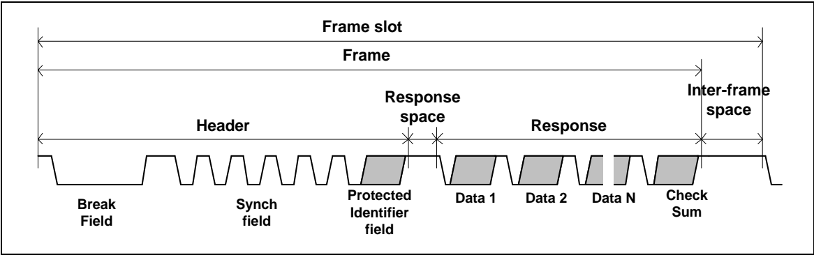
Figure 5-103 Structure of LIN Frame
