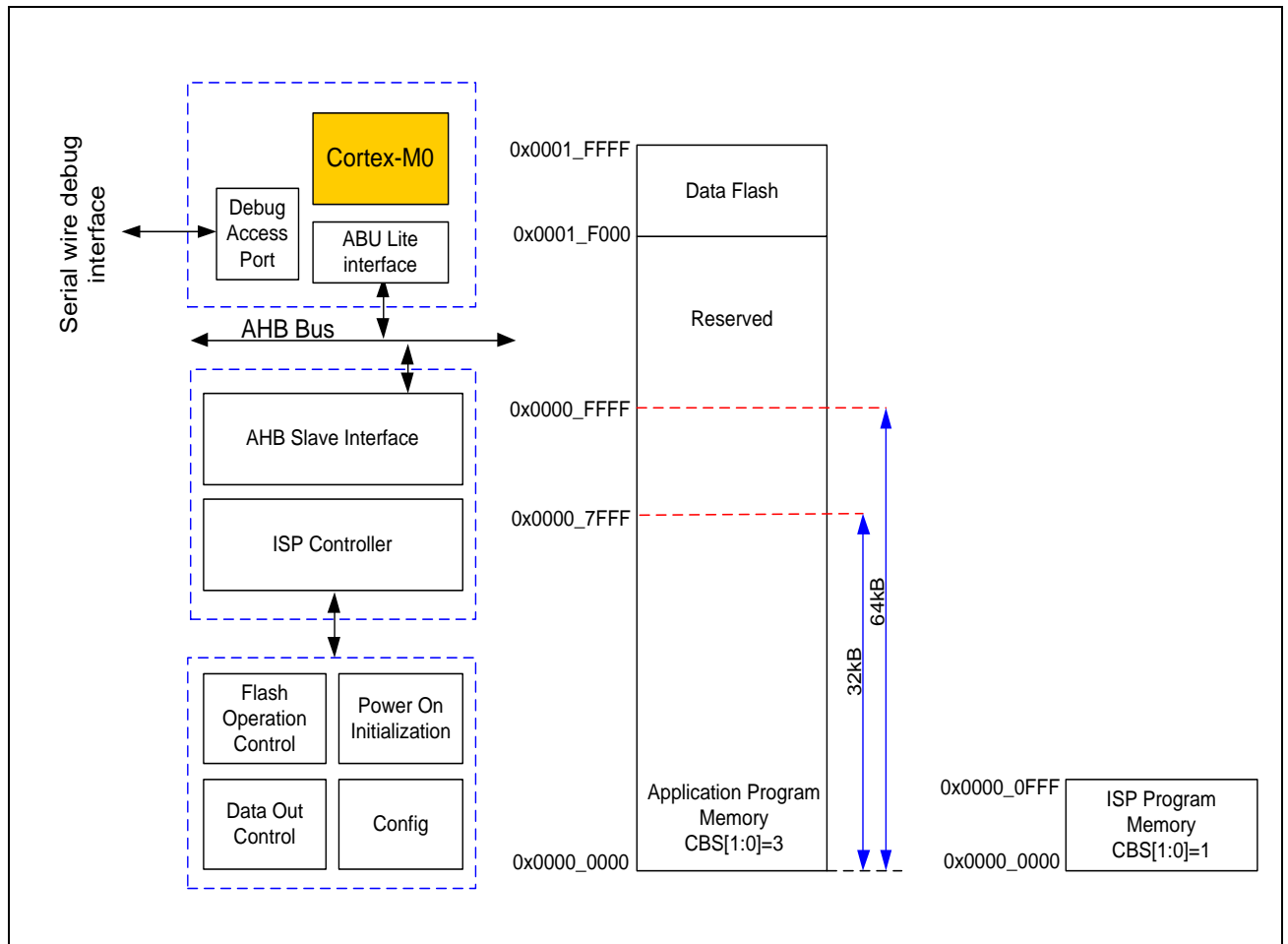
Figure 5-18 Flash Memory Control Block Diagram for NUC029xAN
