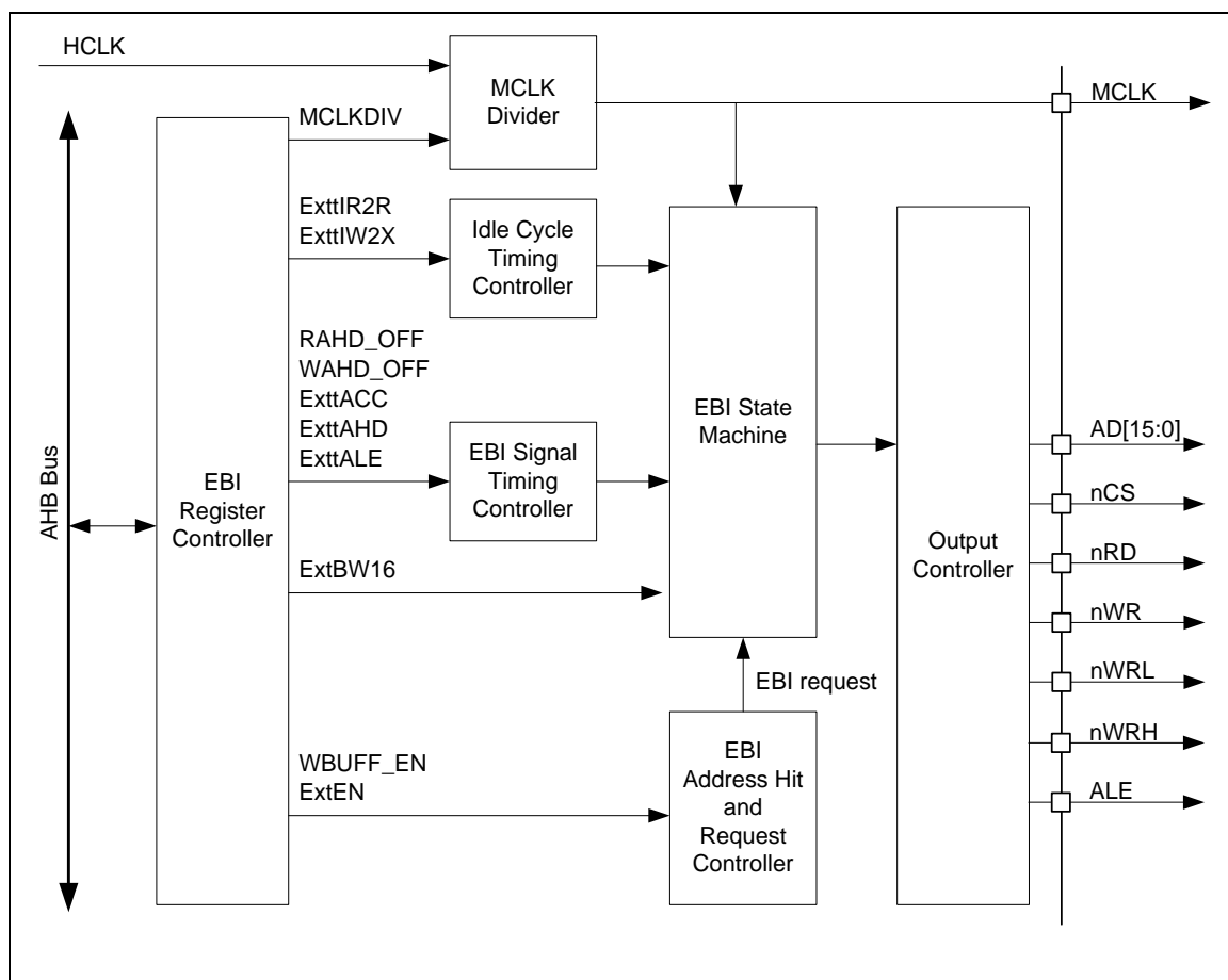
Figure 5-30 EBI Block Diagram
