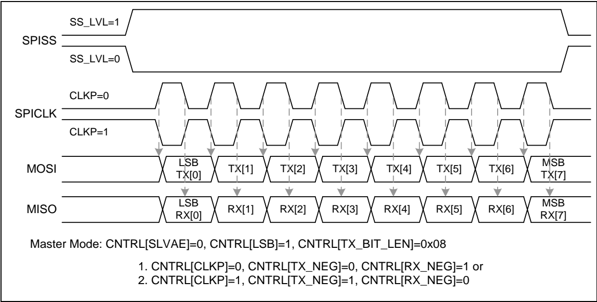
Figure 5-130 SPI Timing in Master Mode (Alternate Phase of SPICLK)
