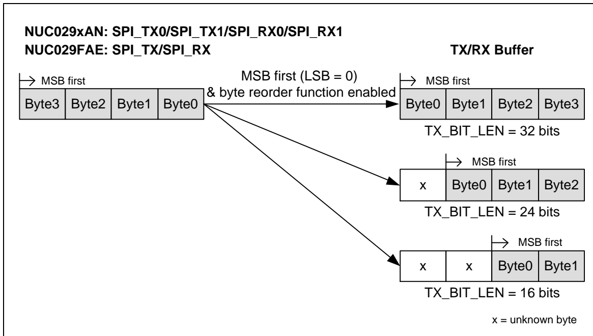
Figure 5-126 Byte Reorder
