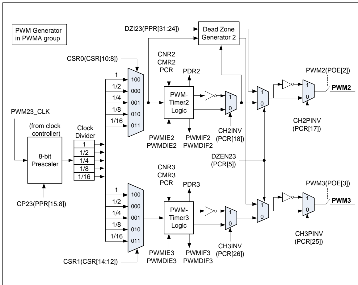
Figure 5-48 PWM Generator 2 Architecture Diagram
