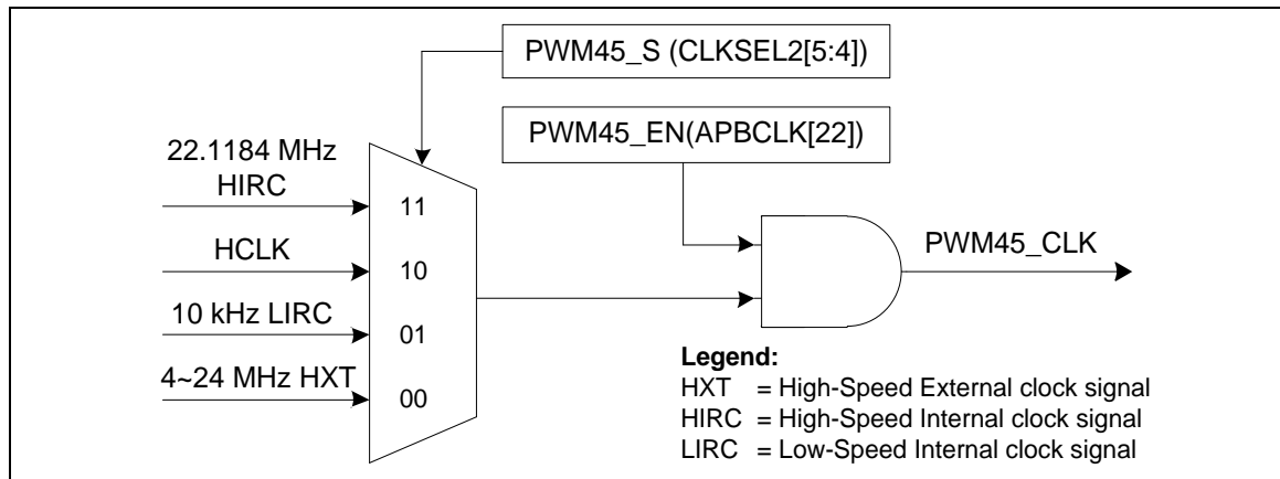
Figure 5-49 PWM Generator 4 Clock Source Control
