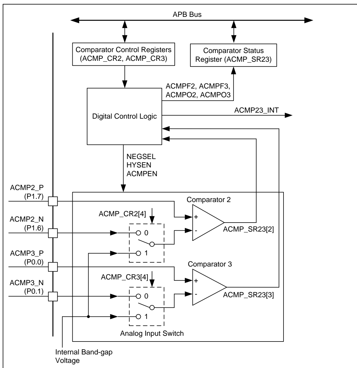
Figure 5-148 Analog Comparator 2/3 Block Diagram for NUC029xAN
