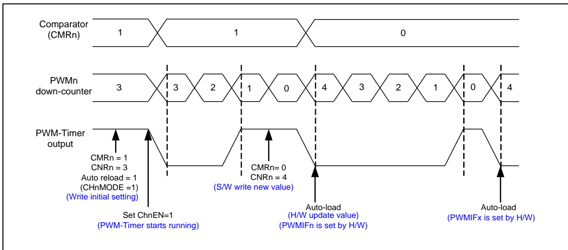
Figure 5-75 PWM-Timer Operation Timing
