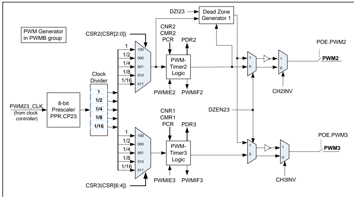
Figure 5-69 PWM Generator 2 Architecture Diagram
