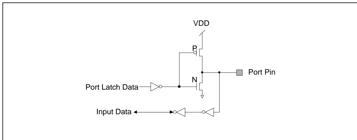
Figure 5-36 Push-Pull Output
