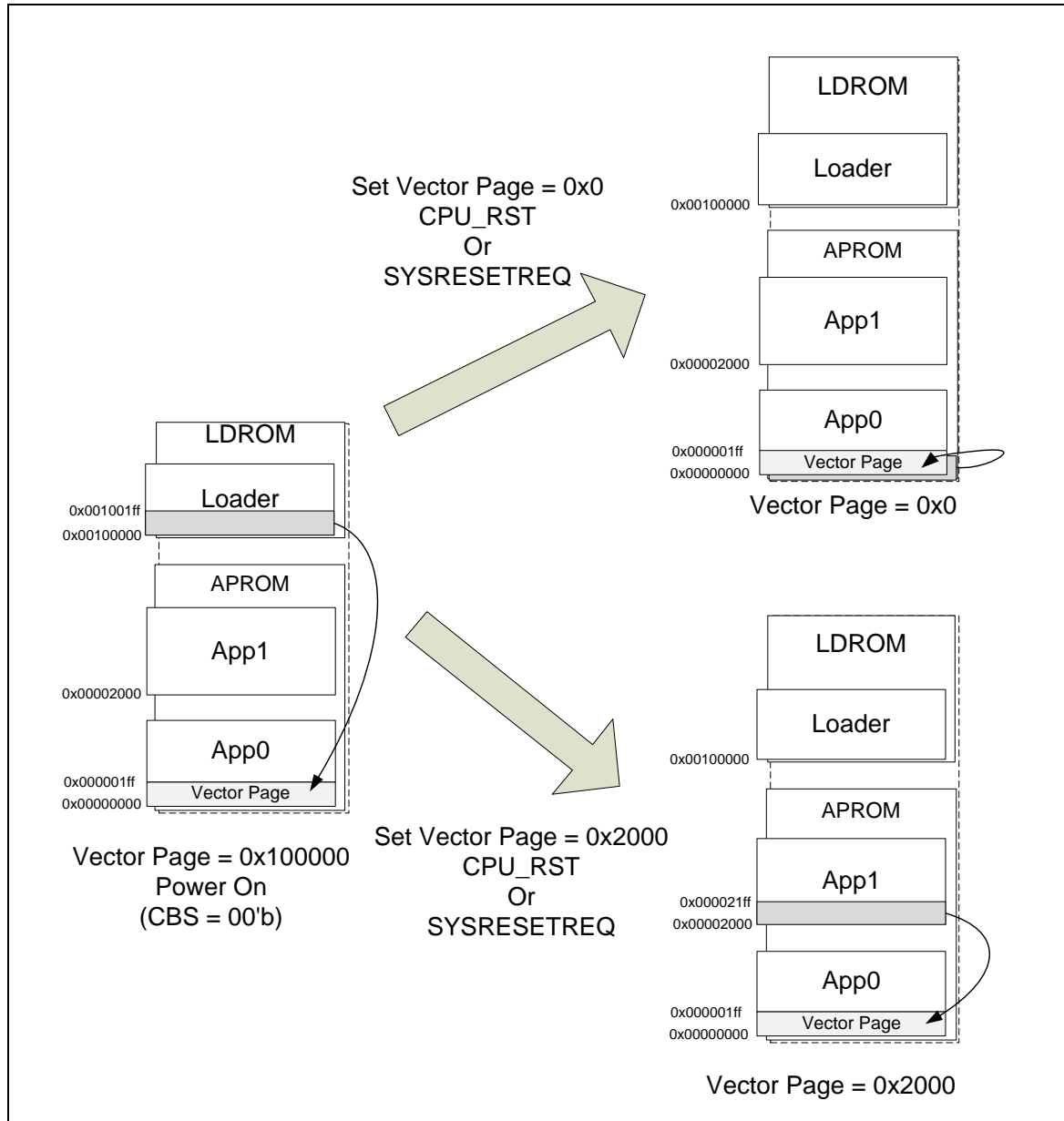
Figure 5-29 Multi-booting by Vector Page Remapping
