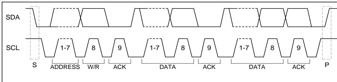
Figure 5-105 I 2 C Protocol
