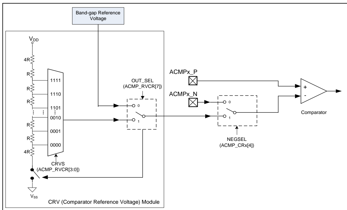
Figure 5-153 Comparator Reference Voltage Block Diagram
