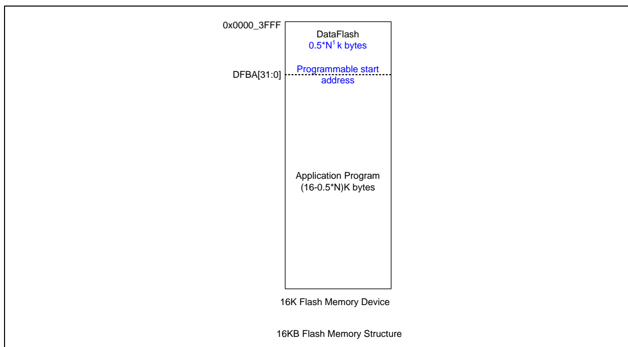
Figure 5-23 Flash Memory Structure for NUC029FAE
