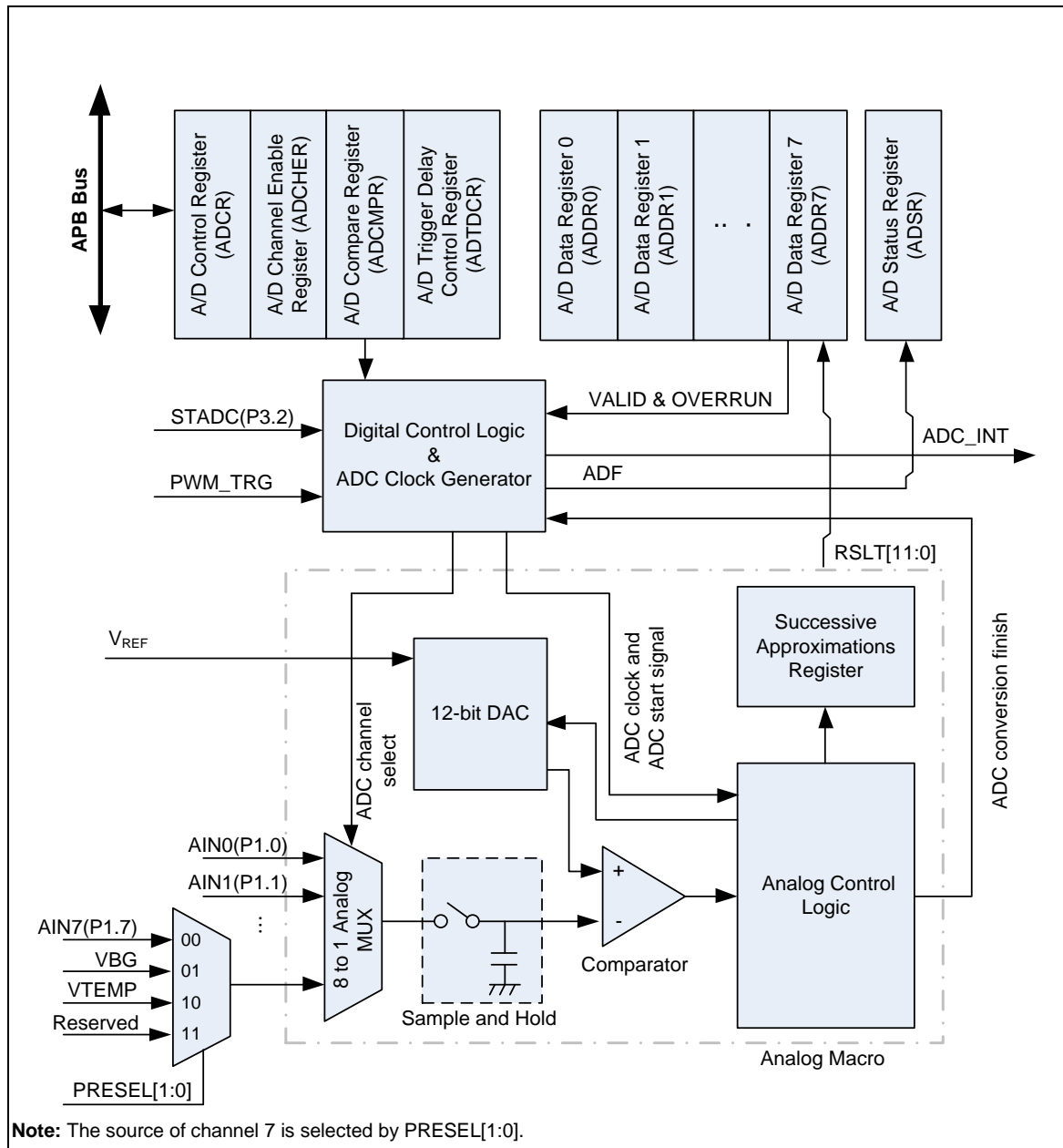
Figure 5-133 A/D Controller Block Diagram for NUC029xAN
