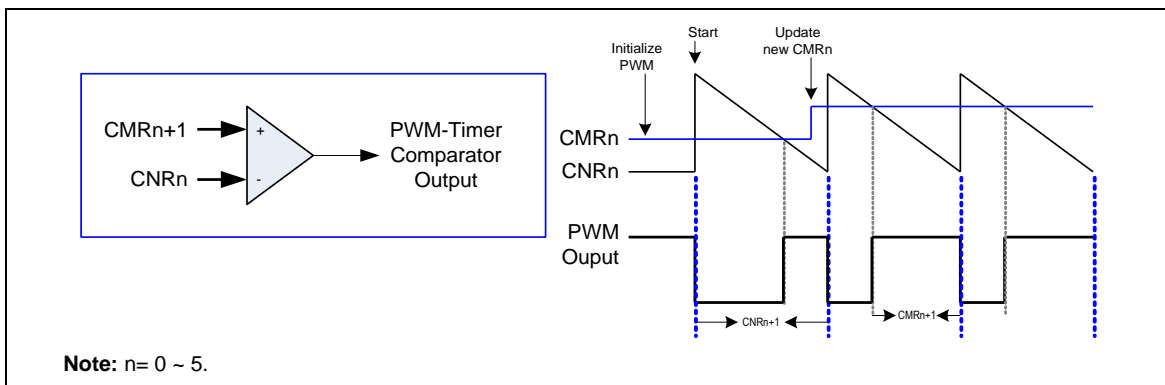
Figure 5-74 Legend of Internal Comparator Output of PWM-Timer
