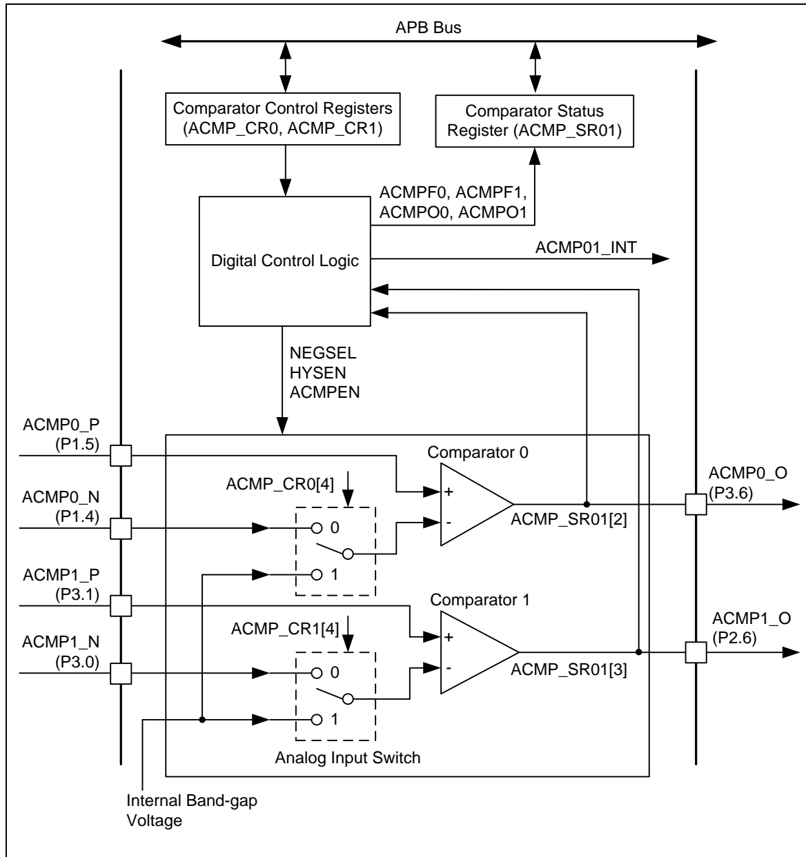
Figure 5-147 Analog Comparator 0/1 Block Diagram for NUC029xAN
