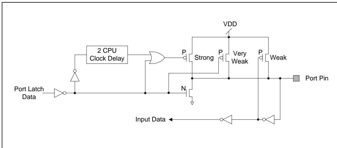
Figure 5-38 Quasi-Bidirectional I/O Mode
