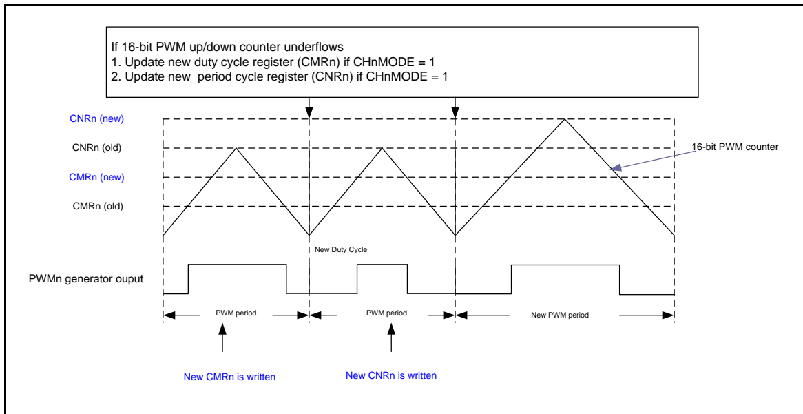
Figure 5-76 Center-aligned Mode
