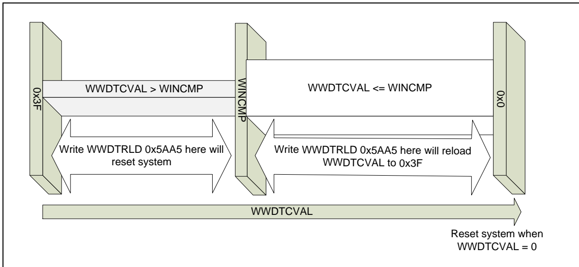
Figure 5-90 Window Watchdog Timer Reset and Reload Behavior
