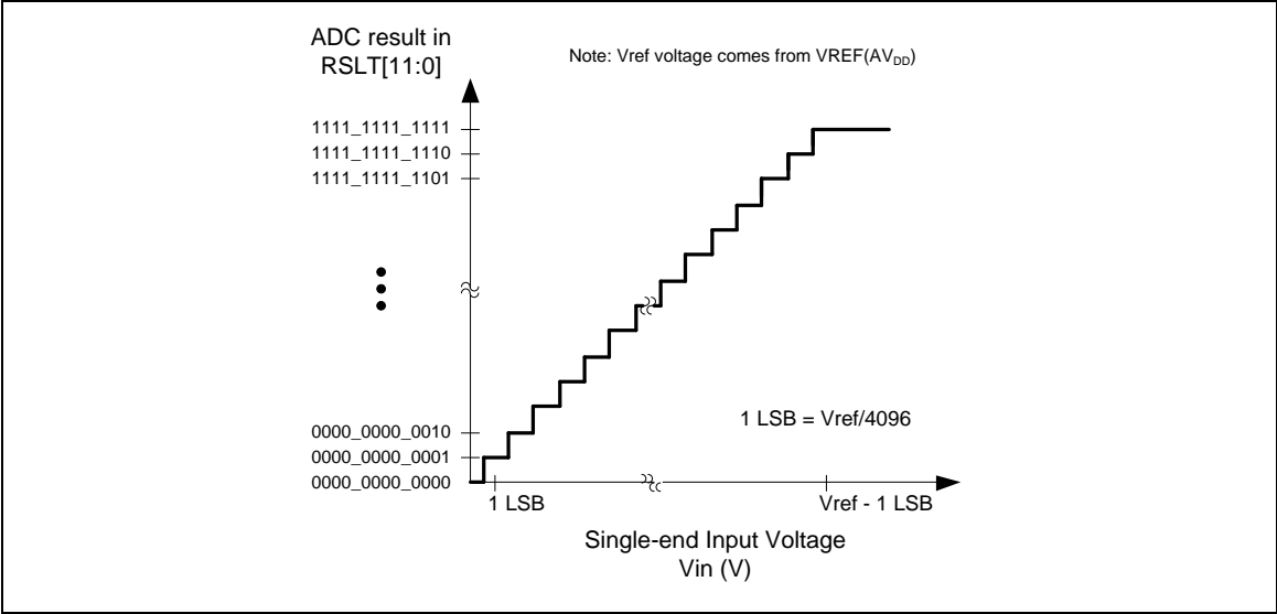
Figure 5-144 Conversion Result Mapping Diagram of ADC Single-end Input
