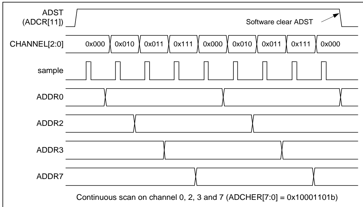
Figure 5-140 Continuous Scan Mode on Enabled Channels Timing Diagram
