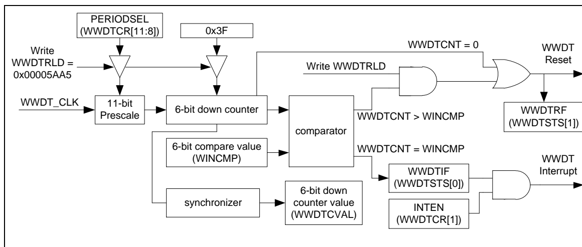
Figure 5-89 Window Watchdog Timer Block Diagram
