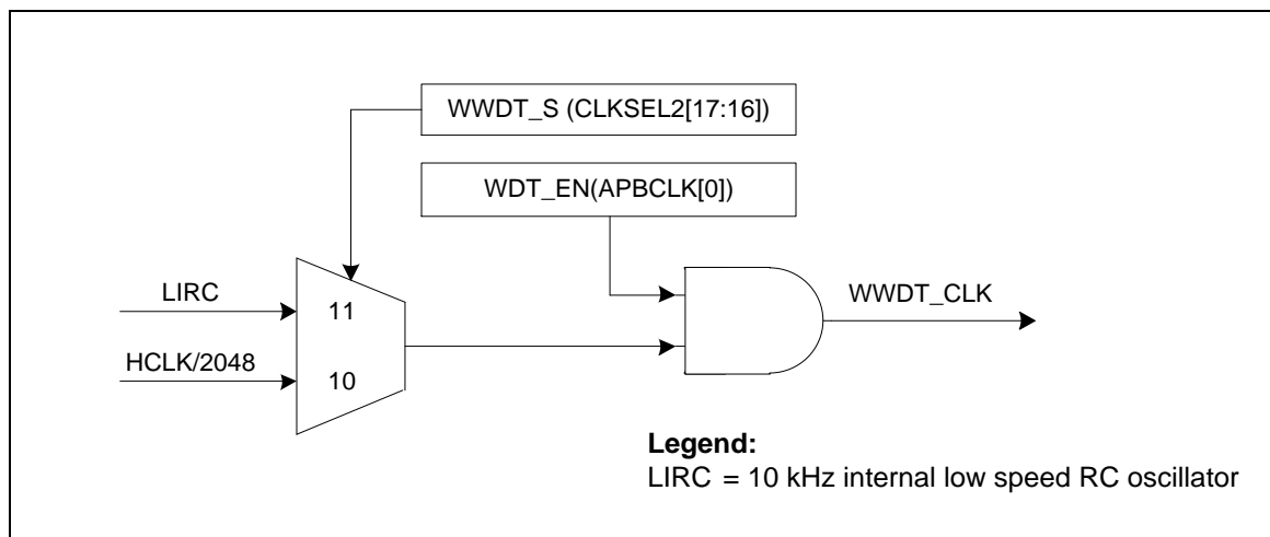
Figure 5-88 Window Watchdog Timer Clock Control
