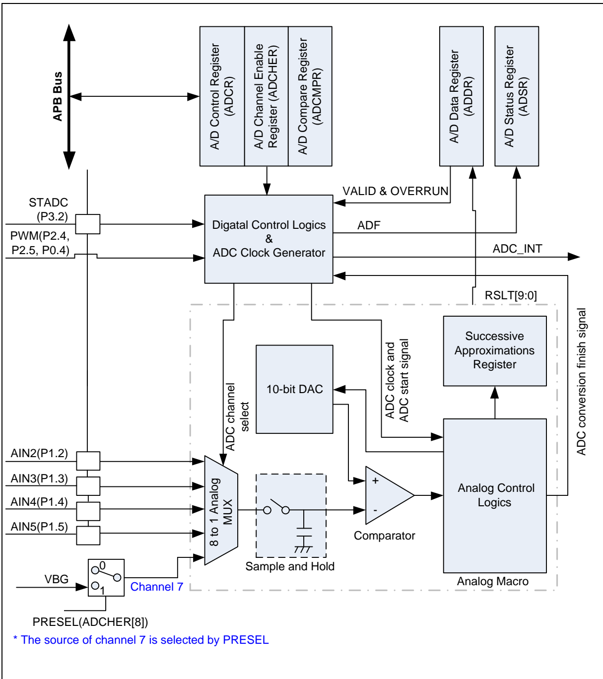
Figure 5-134 A/D Controller Block Diagram for NUC029FAE
