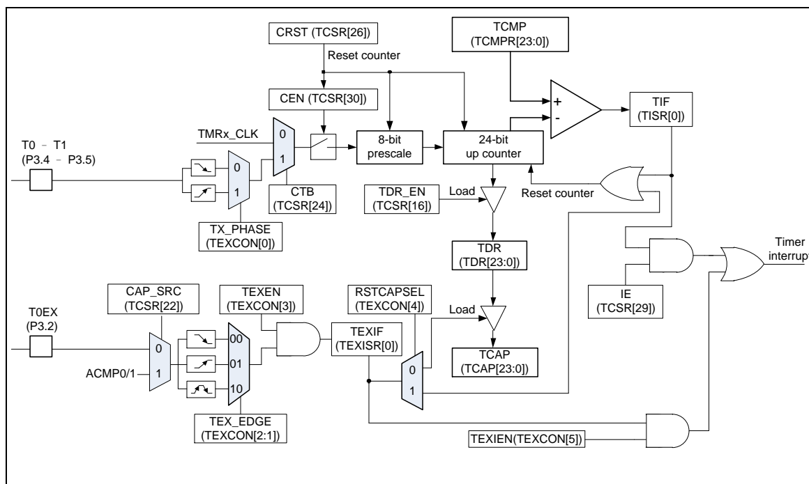
Figure 5-41 Timer Controller Block Diagram for NUC029FAE
