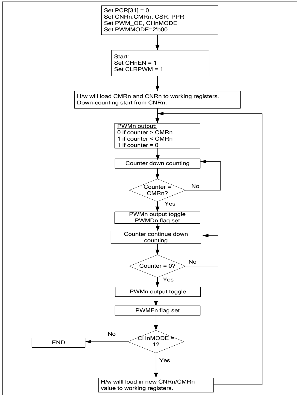
Figure 5-73 Edge-aligned Flow Diagram
