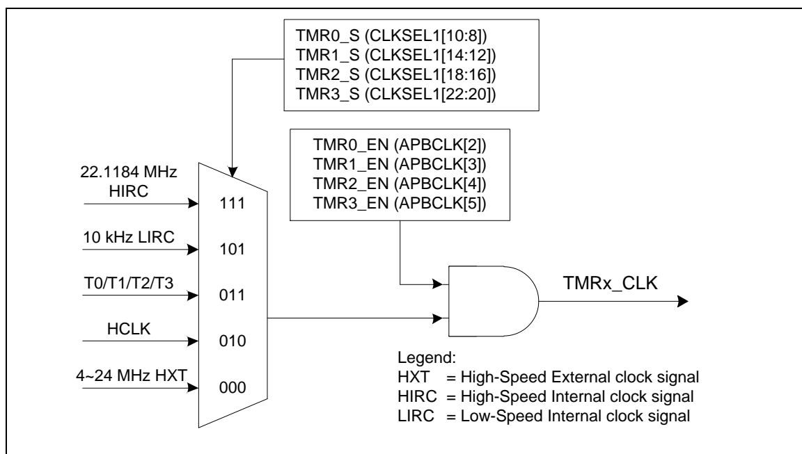
Figure 5-40 Clock Source of Timer Controller for NUC029xAN
