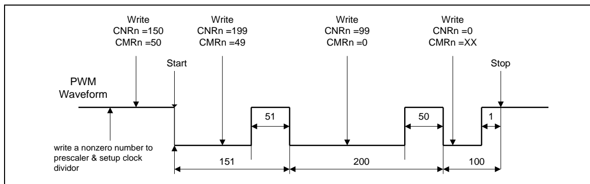
Figure 5-80 PWM Double Buffering Illustration
