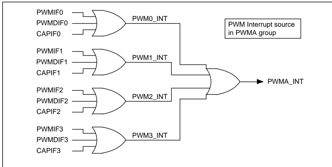
Figure 5-65 PWM Group A PWM-Timer Interrupt Architecture Diagram
