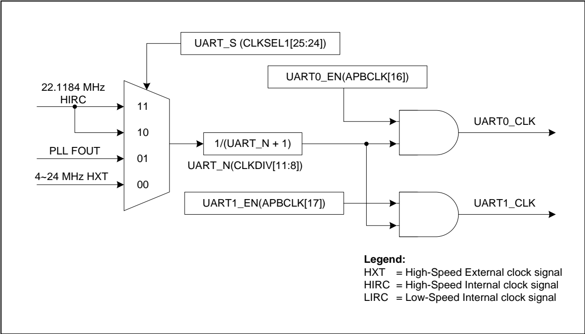
Figure 5-91 UART Controller Clock Control for NUC029xAN
