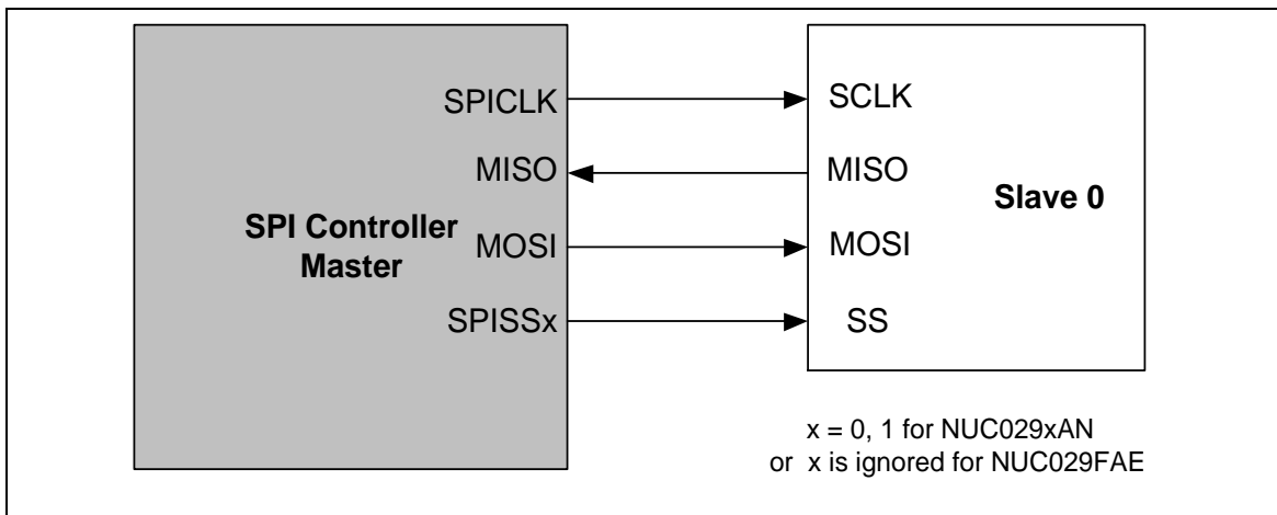
Figure 5-123 SPI Master Mode Application Block Diagram
