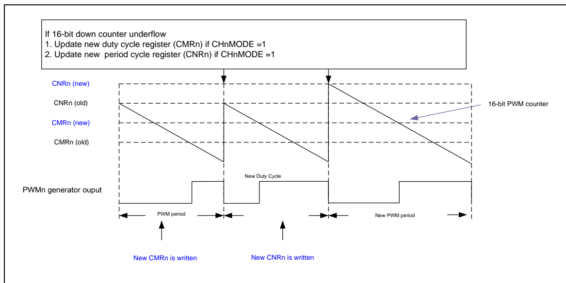
Figure 5-71 Edge-aligned PWM
