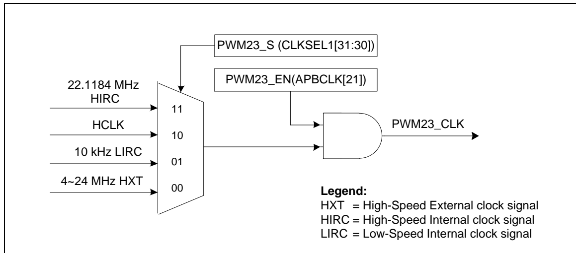
Figure 5-47 PWM Generator 2 Clock Source Control
