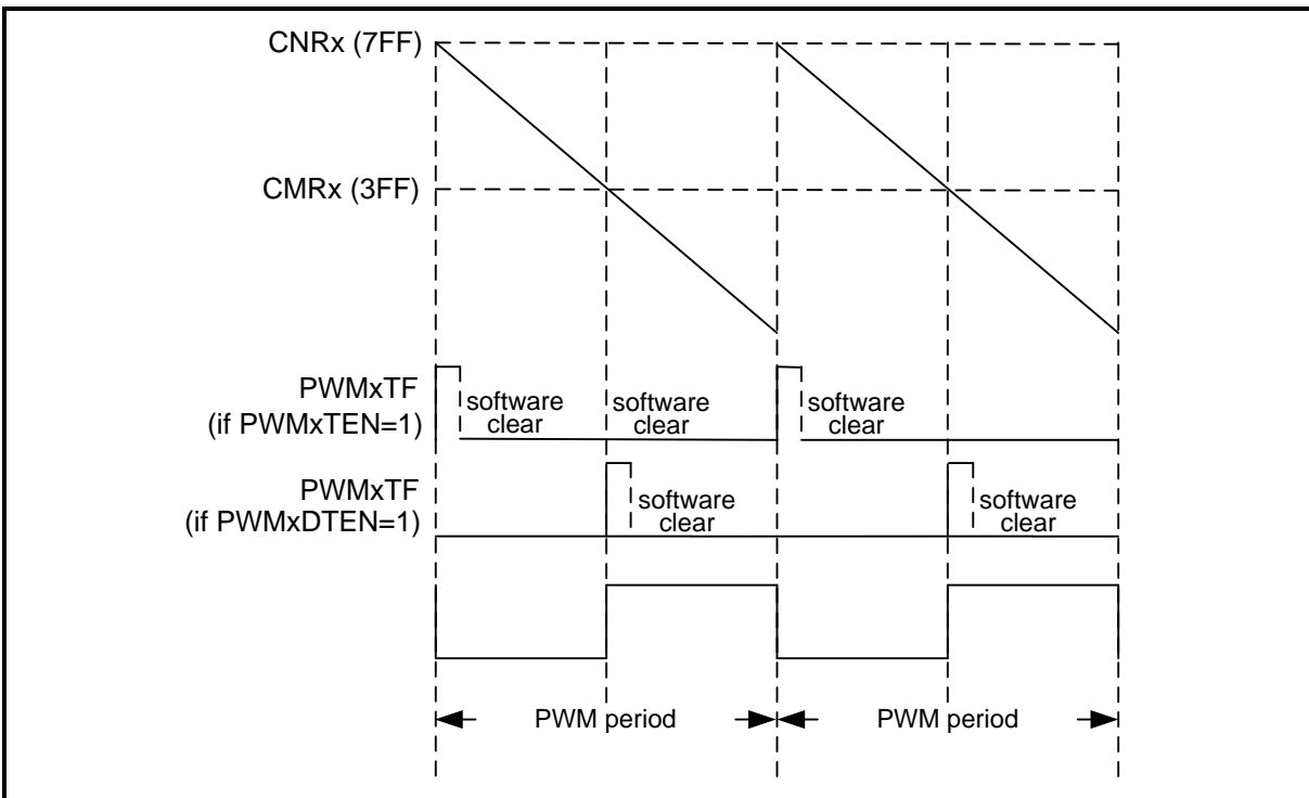
Figure 5-62 PWM Trigger ADC Flag (PWMxTF) in Edge-aligned Type Timing Waveform
