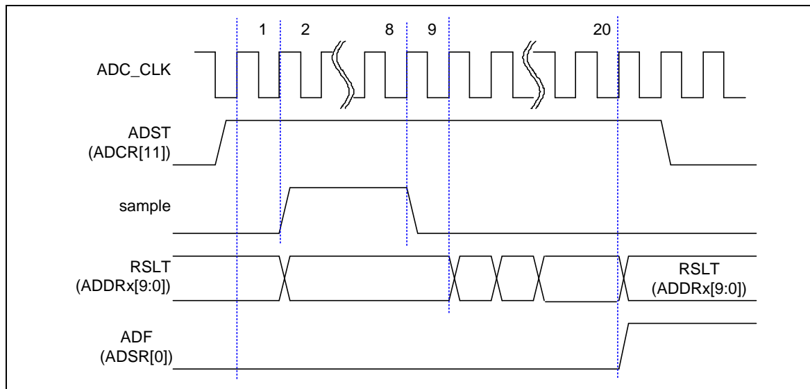
Figure 5-138 Single Mode Conversion Timing Diagram for NUC029FAE
