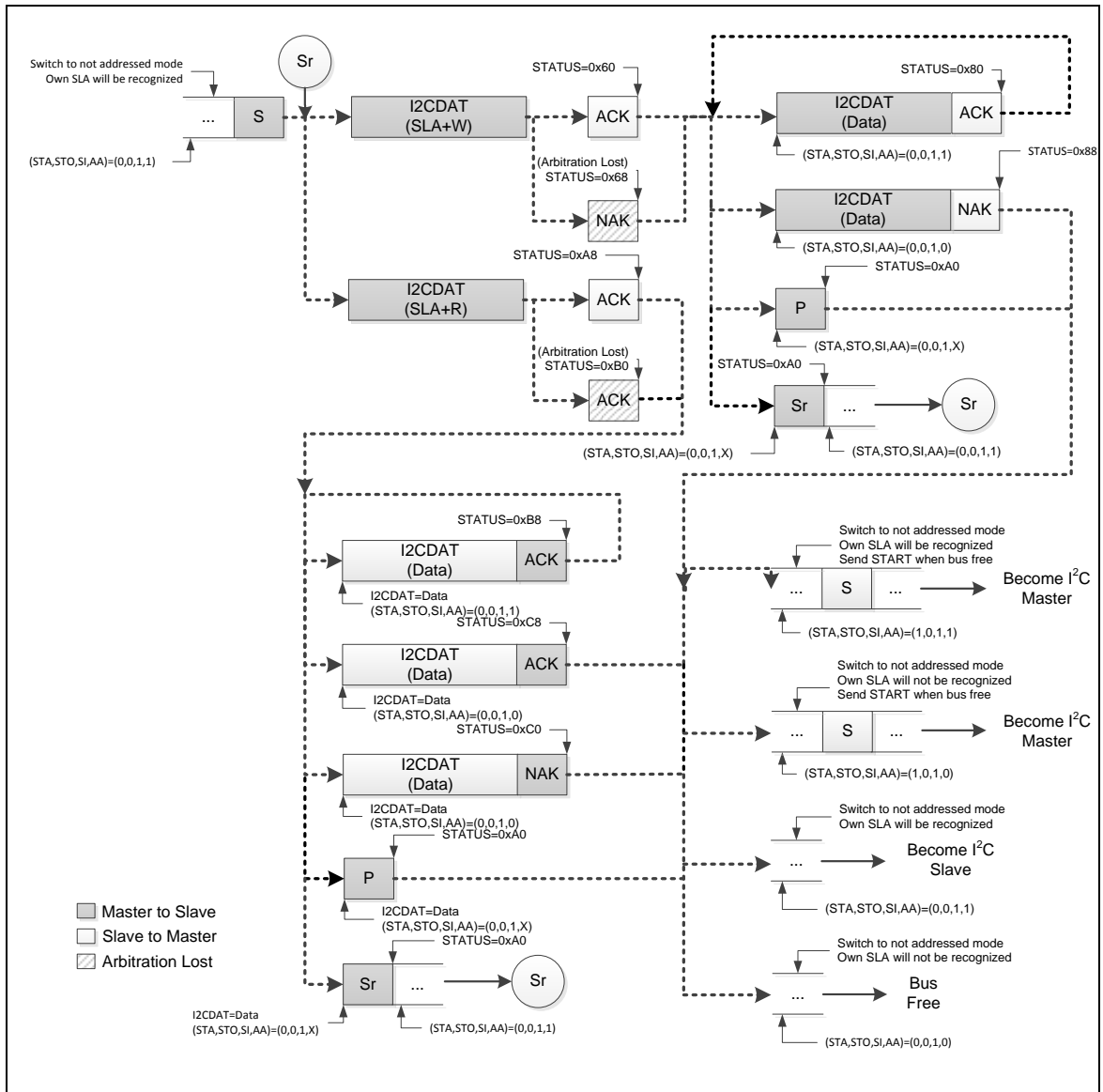
Figure 5-118 Save Mode Control Flow
