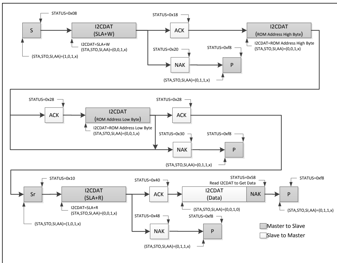
Figure 5-121 Protocol of EEPROM Random Read
