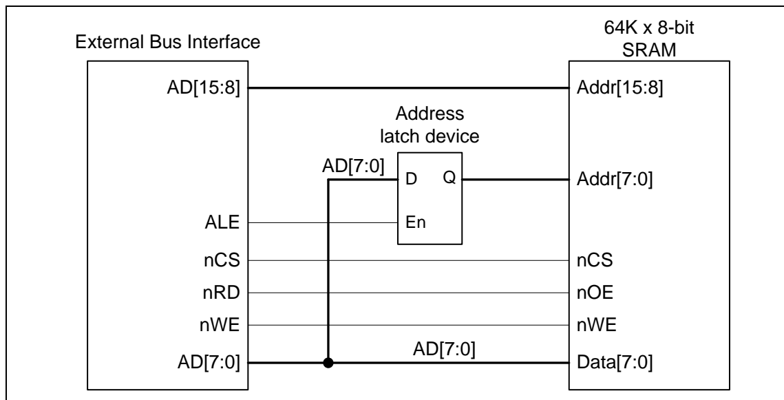
Figure 5-32 Connection of 8-bit EBI Data Width with 8-bit Device
