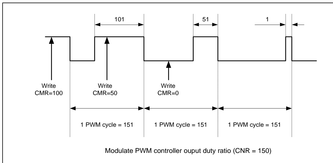
Figure 5-59 PWM Controller Output Duty Ratio
