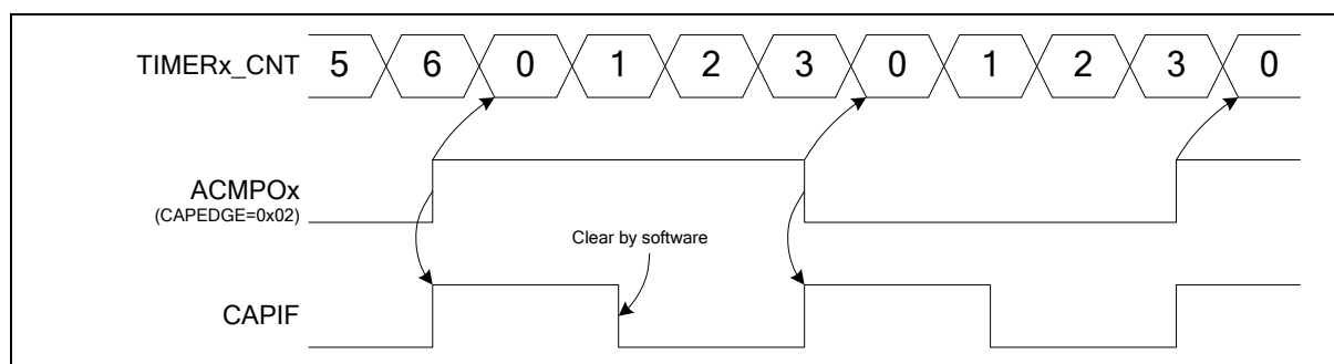
Figure 6.6-5 External Reset Counter Mode
