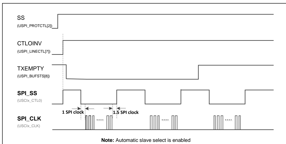
Figure 6.13-12 Auto Slave Select ( SUSPITV \geq 0x3 )
