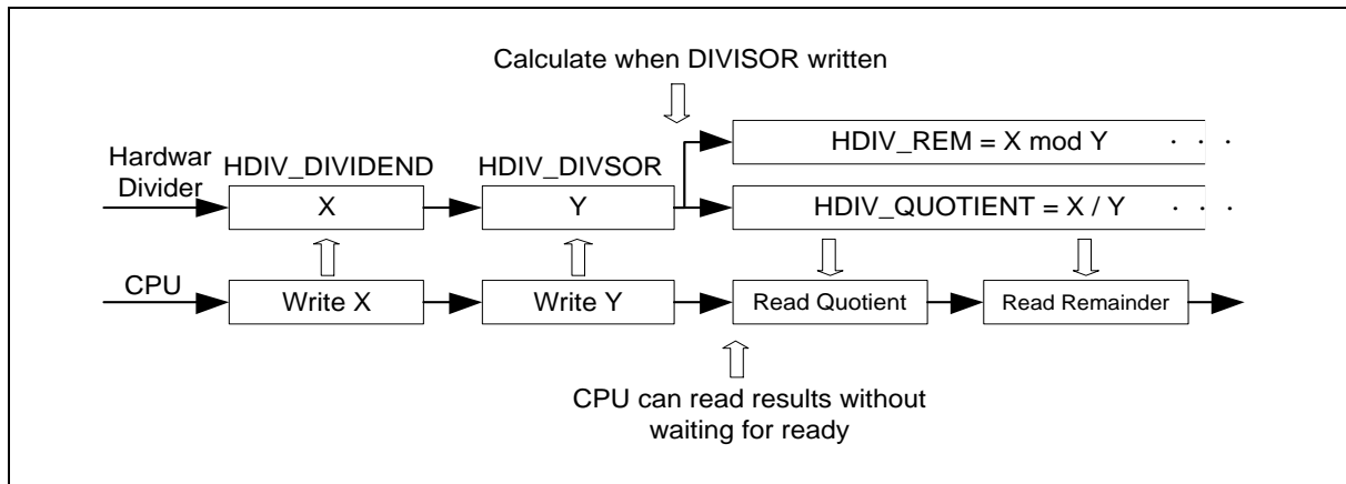
Figure 6.15-1 Hardware Divider Operation Flow
