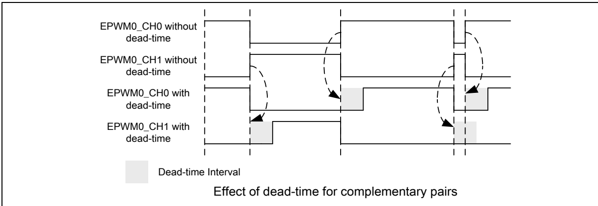
Figure 6.8-17 EPWM Dead-time Insertion
