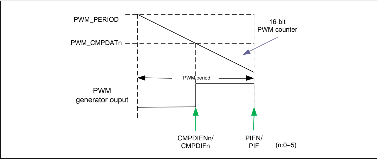
Figure 6.8-8 EPWM Edge-aligned Interrupt Diagram
