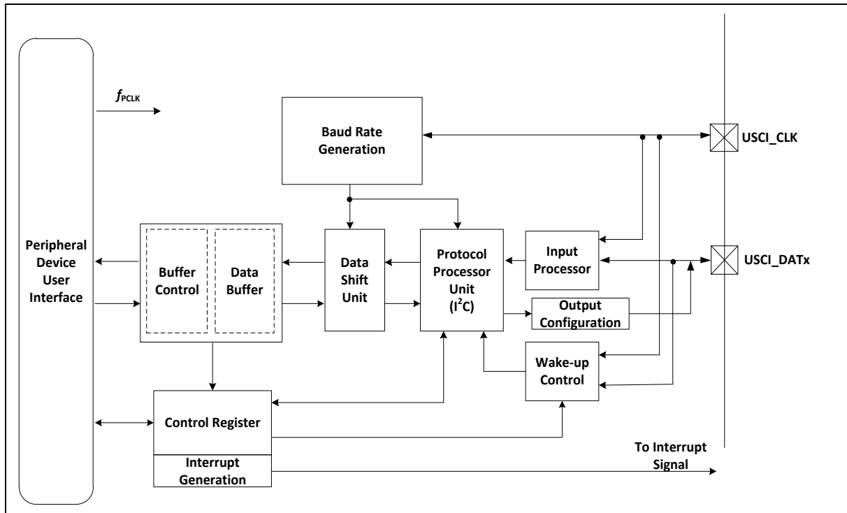
Figure 6.14-2 USCI - I²C Mode Block Diagram
