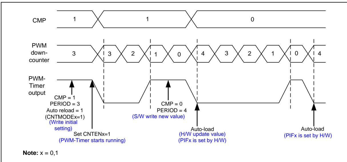
Figure 6.9-3 Legend of Internal Comparator Output of PWM-Timer
