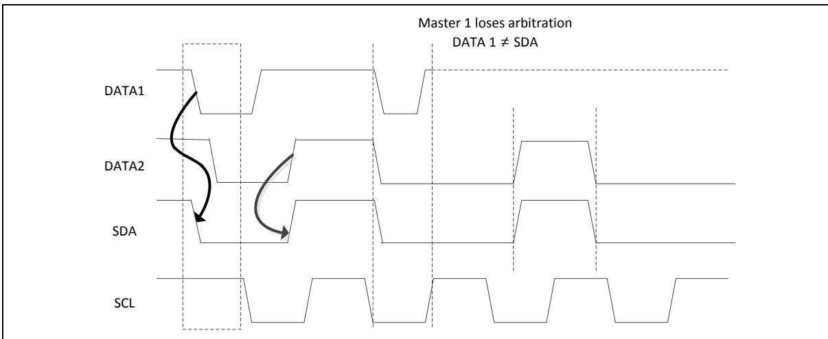
Figure 6.14-7 Arbitration Lost
