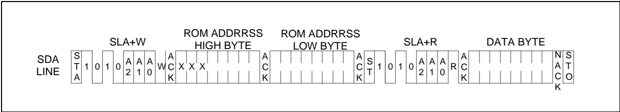
Figure 6.14-20 EEPROM Random Read
