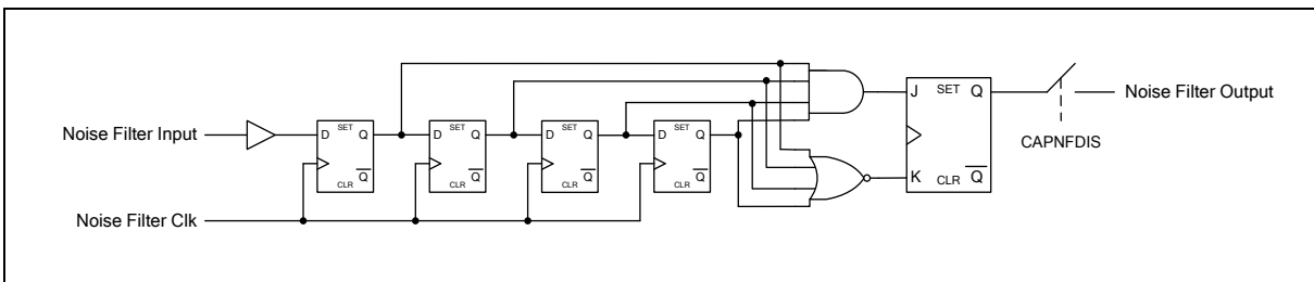
Figure 6.7-4 Noise Filter
