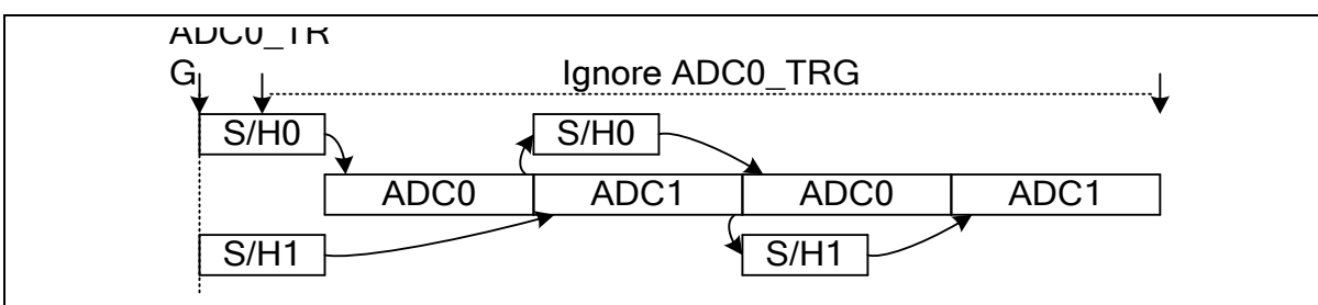
Figure 6.16-7 Simultaneous Sequential 4R Mode Conversion Timing Diagram
