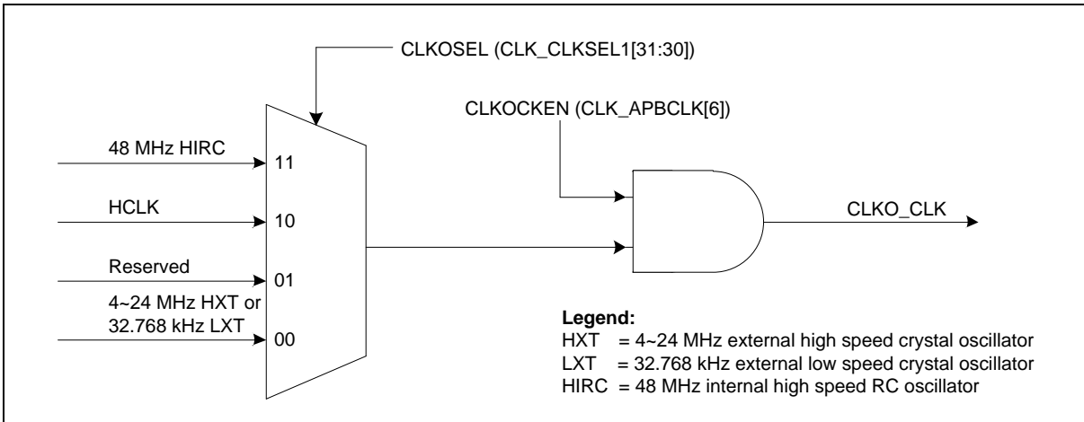
Figure 6.3-6 Clock Source of Frequency Divider
