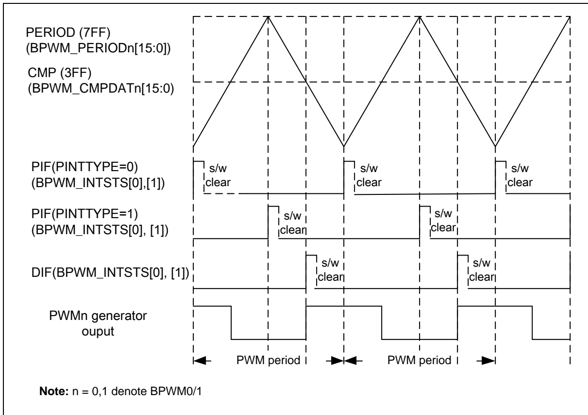
Figure 6.9-7 PWM Center-aligned Interrupt Generate Timing Waveform
