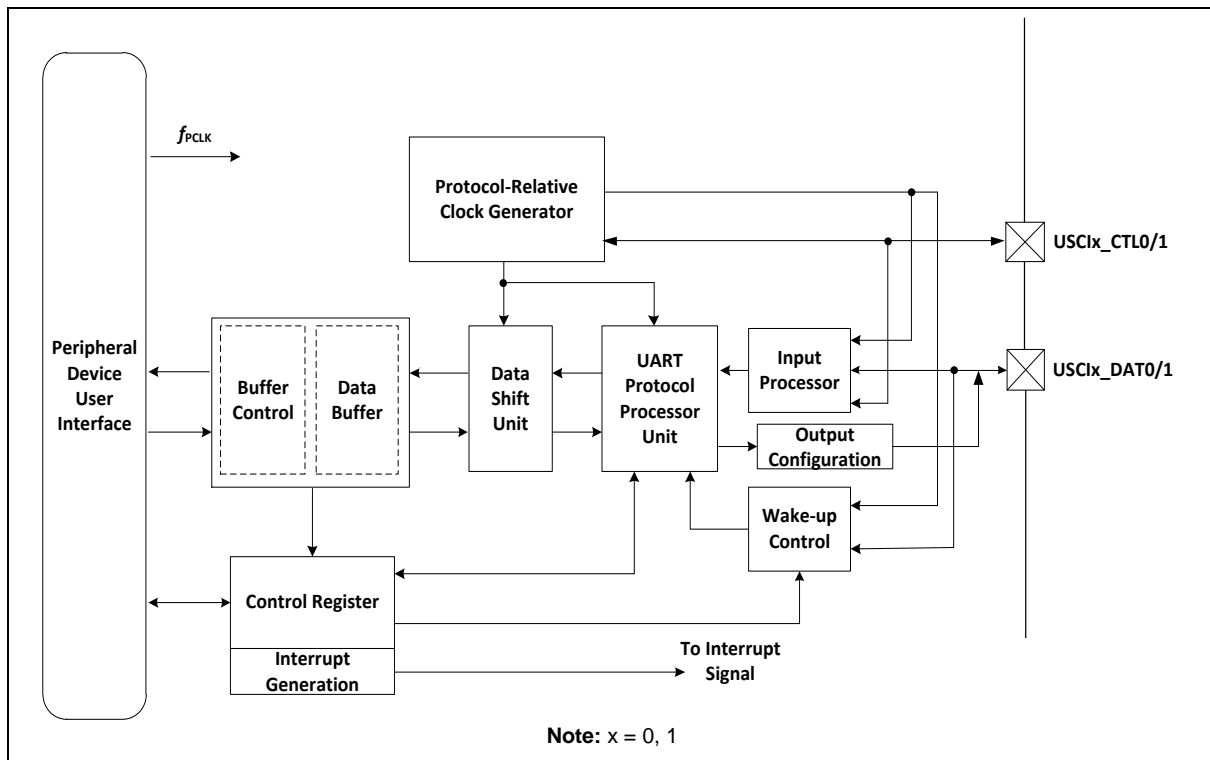
Figure 6.12-1 USCI - UART Mode Block Diagram
