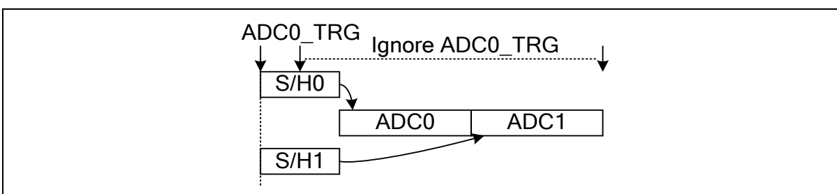
Figure 6.16-6 Simultaneous Simple Mode Conversion Timing Diagram
