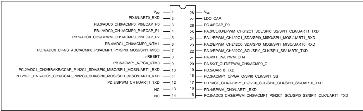
Figure 4.3-4 NuMicro® Mini57 Series TSSOP 28-pin Multi-function Diagram
