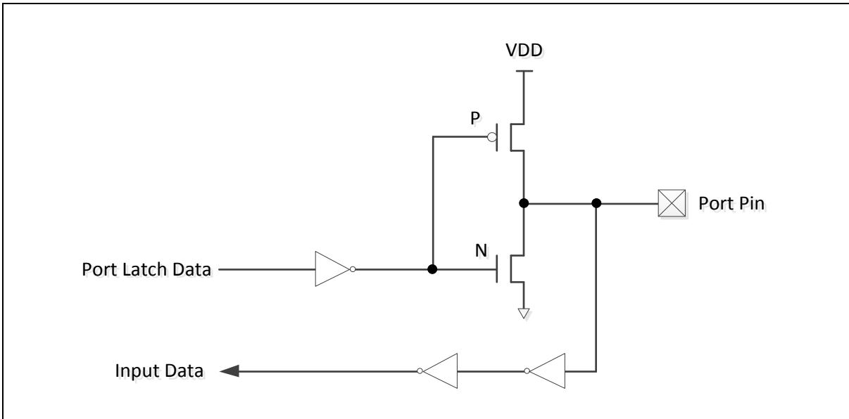
Figure 6.5-3 Push-Pull Output
