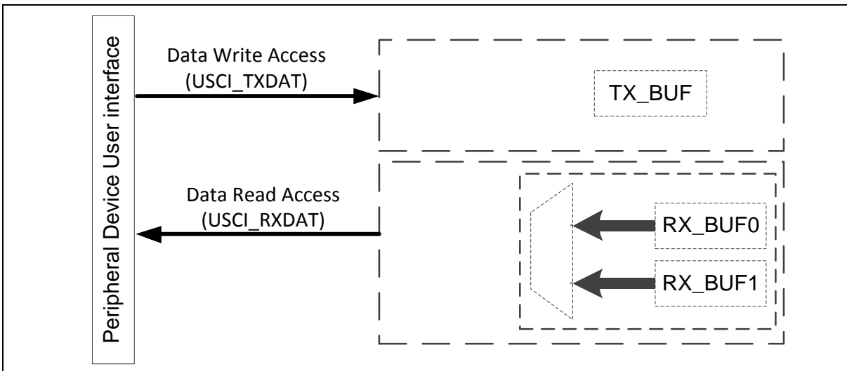
Figure 6.11-5 Data Access Structure
