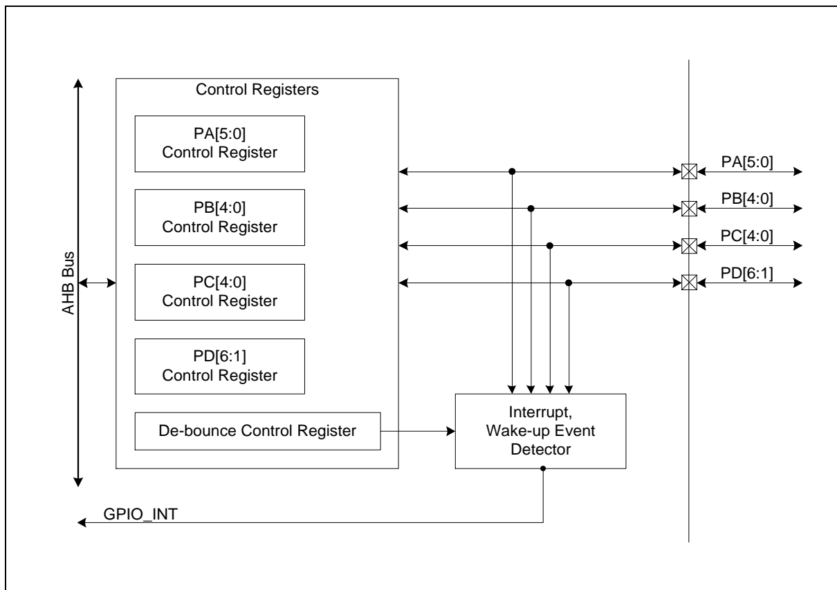
Figure 6.5-2 GPIO Controller Block Diagram
