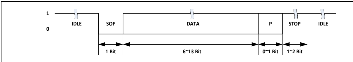
Figure 6.12-3 UART Standard Frame Format
