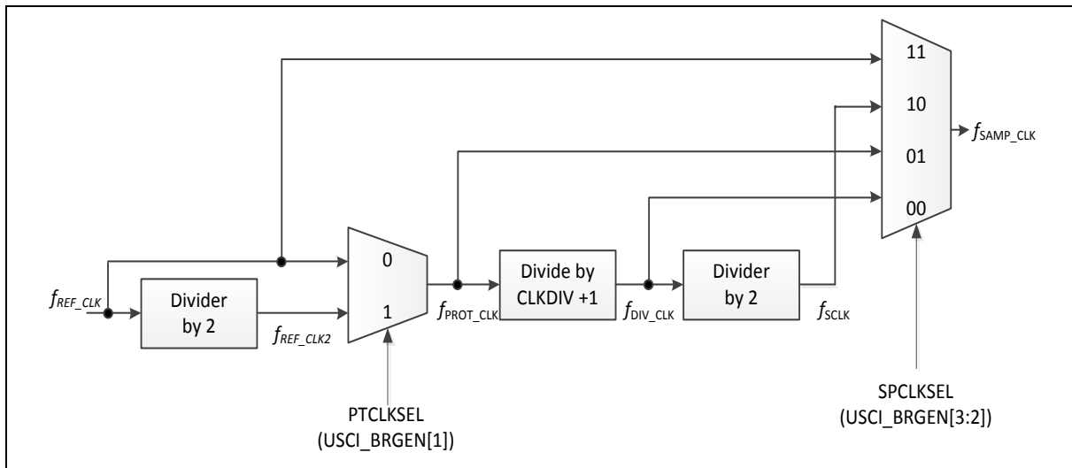
Figure 6.11-9 Basic Clock Divider Counter
