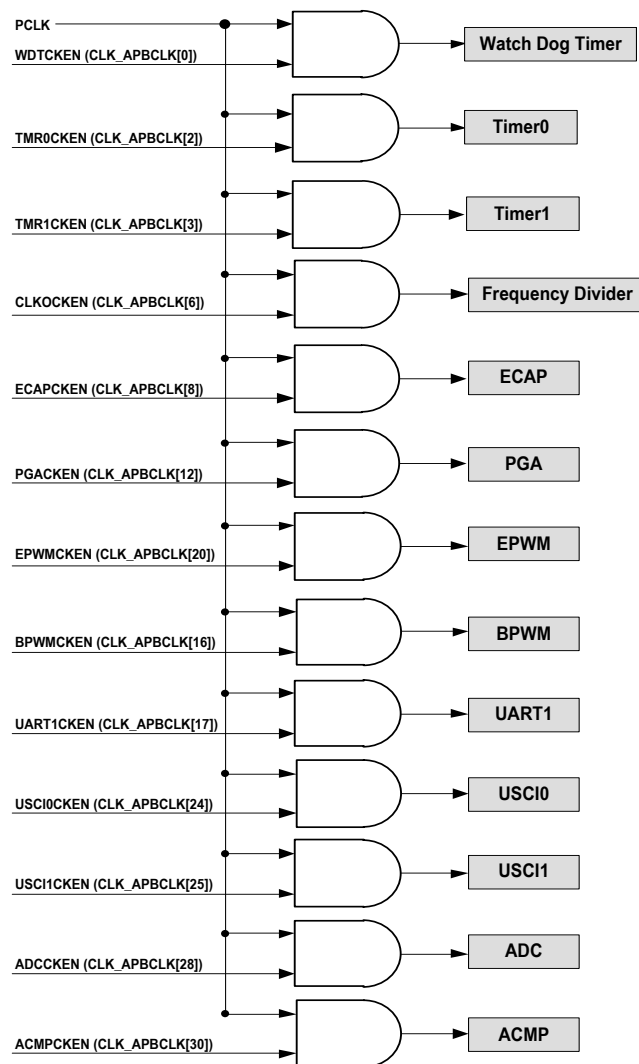
Figure 6.3-5 Peripherals Bus Clock Source Selection for PCLK
