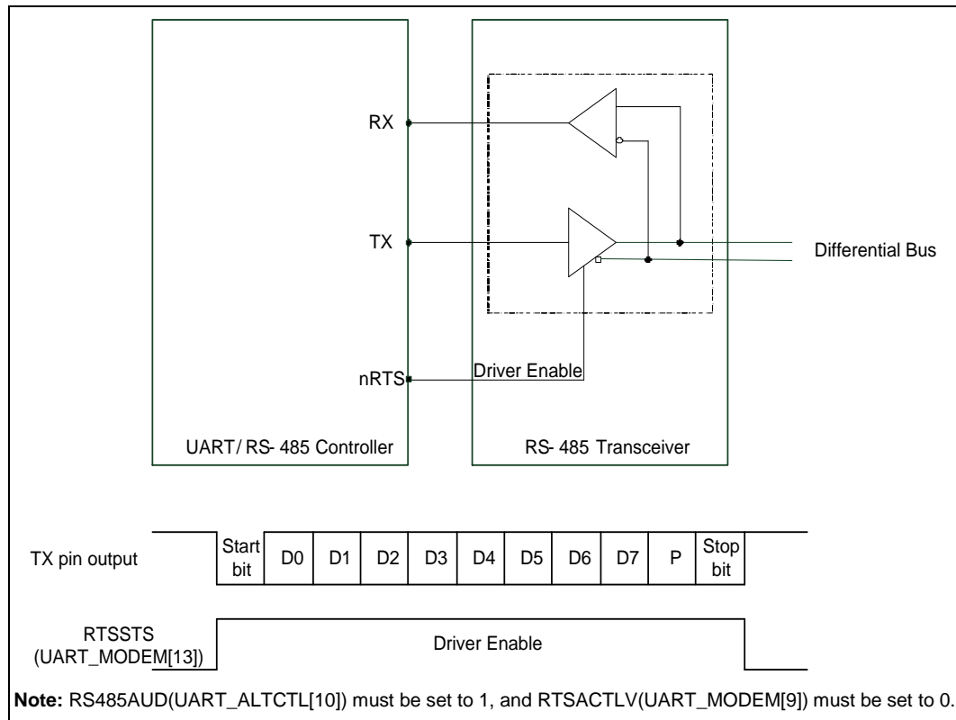
Figure 6.13-16 Structure of RS-485 Frame
