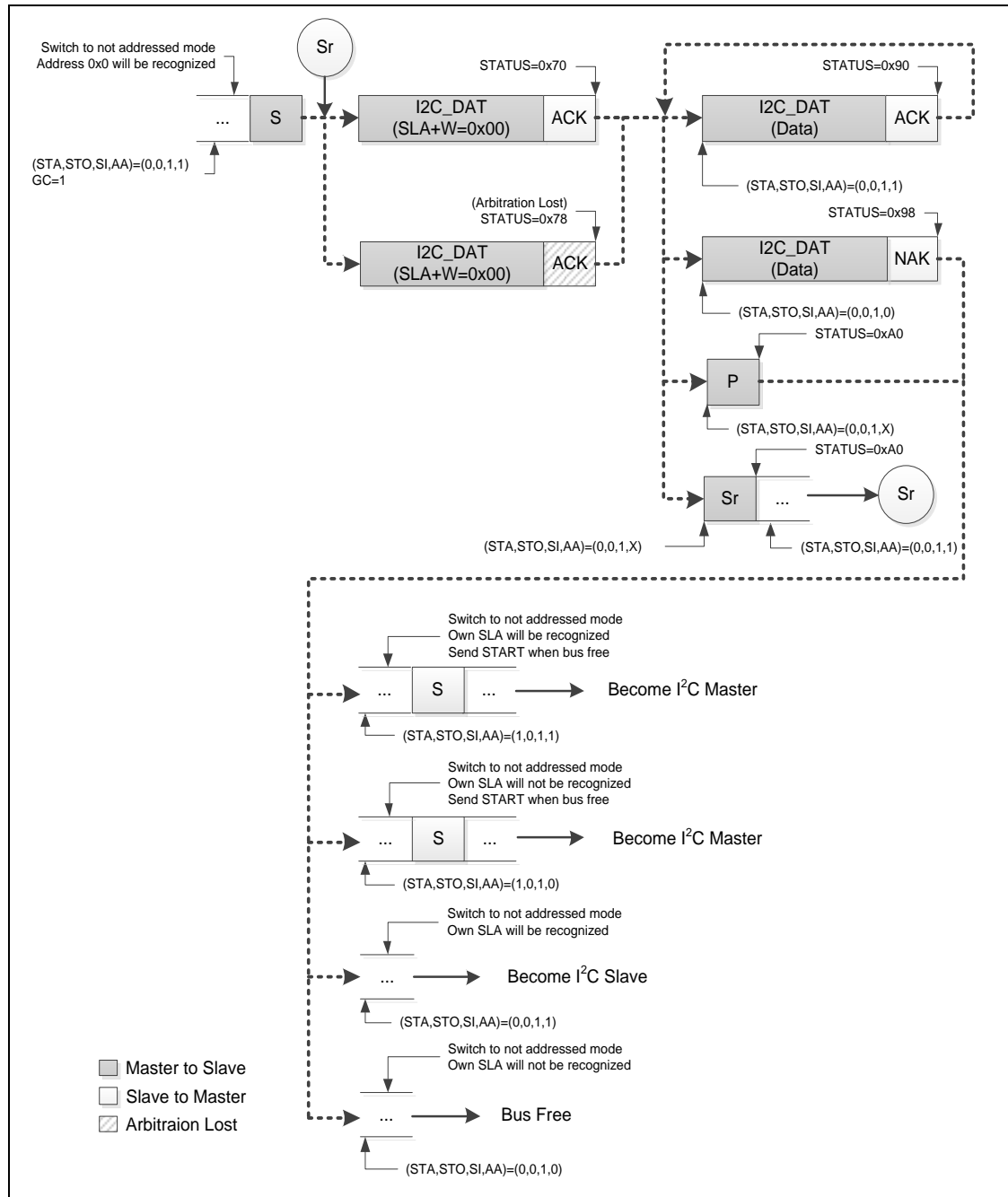
Figure 6.15-13 GC Mode
