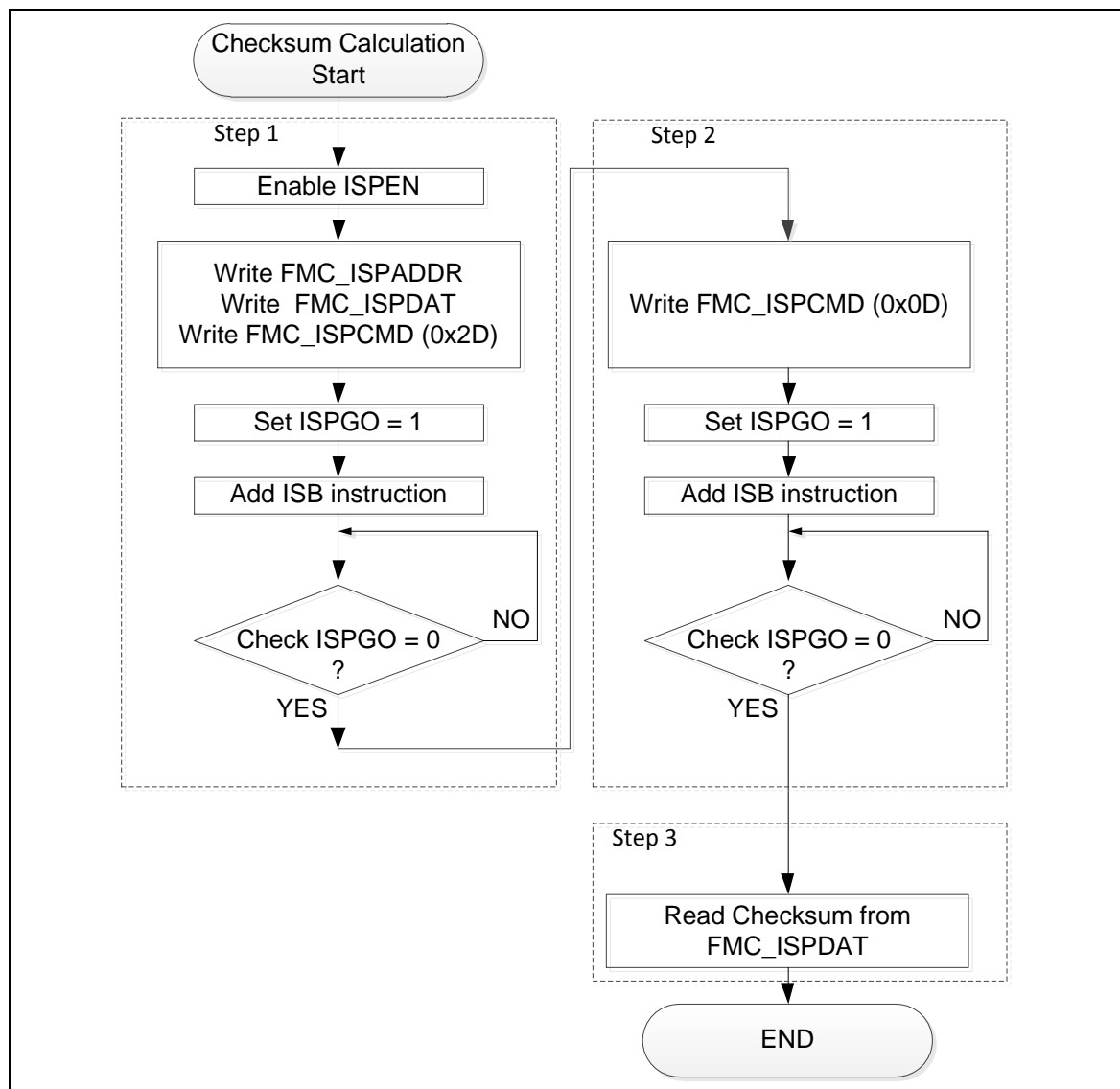
Figure 6.4-18 Checksum Calculation Flow
