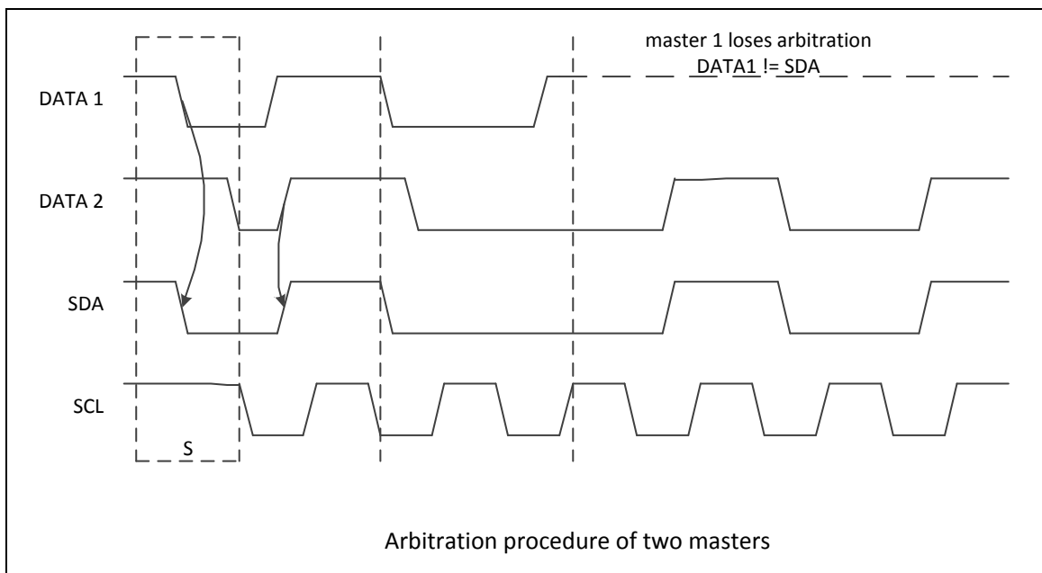
Figure 6.15-14 Arbitration Lost
