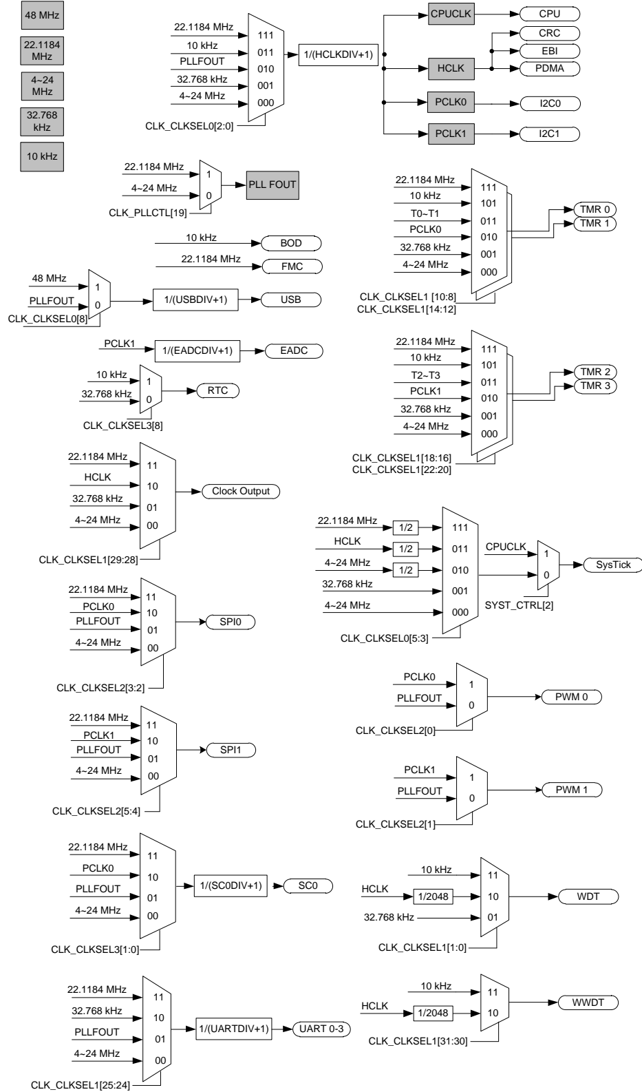
Figure 6.3-1 Clock Generator Global View Diagram
