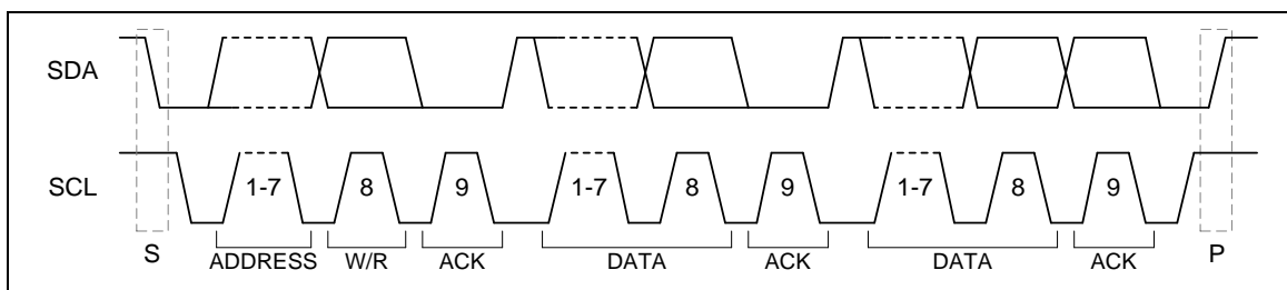
Figure 6.15-3 I²C Protocol
