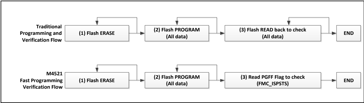
Figure 6.4-16 Verification Flow
