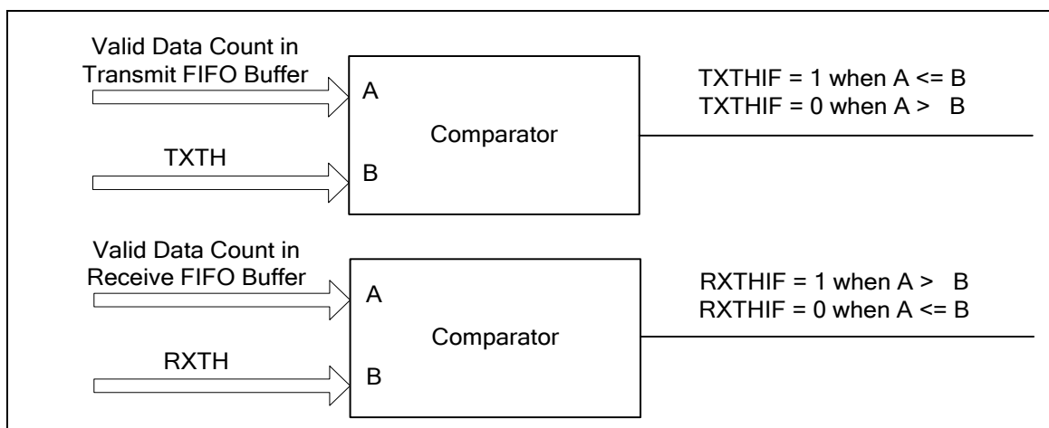
Figure 6.16-17 FIFO Threshold Comparator
