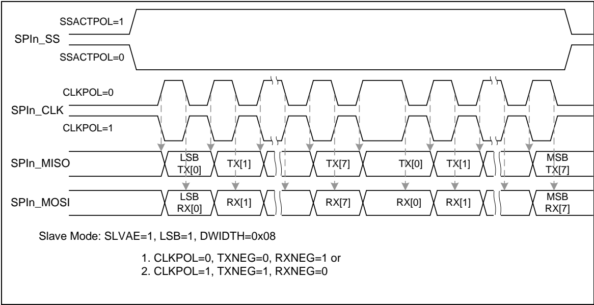
Figure 6.16-28 SPI Timing in Slave Mode (Alternate Phase of SPIn_CLK)
