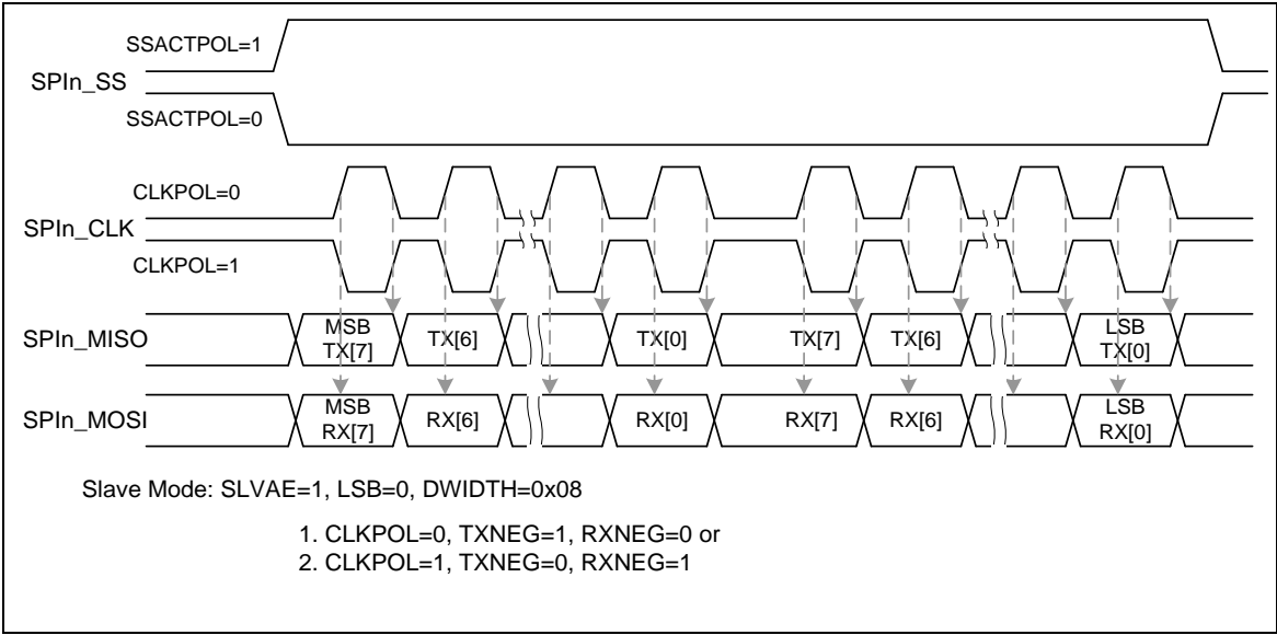
Figure 6.16-27 SPI Timing in Slave Mode
