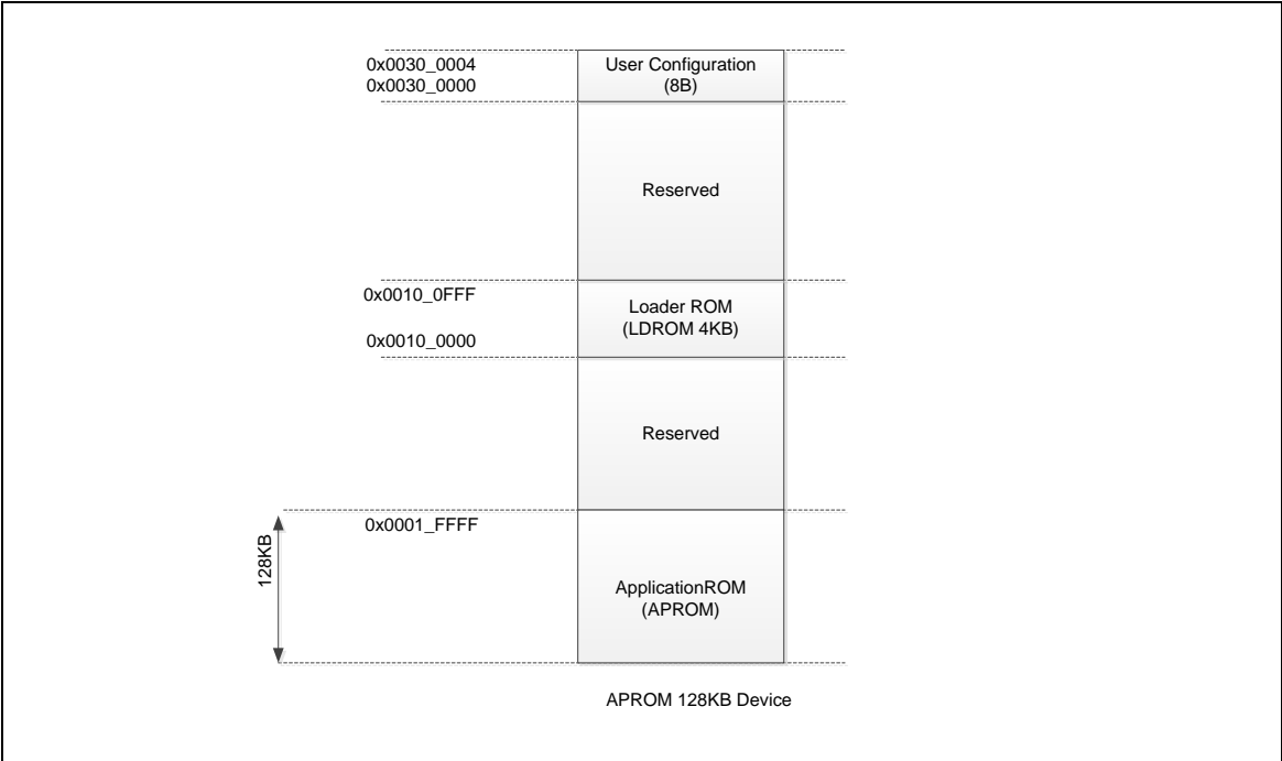
Figure 6.4-3 Flash Memory Map
