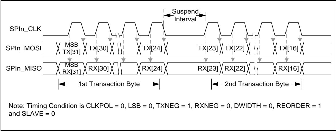
Figure 6.16-10 Timing Waveform for Byte Suspend
