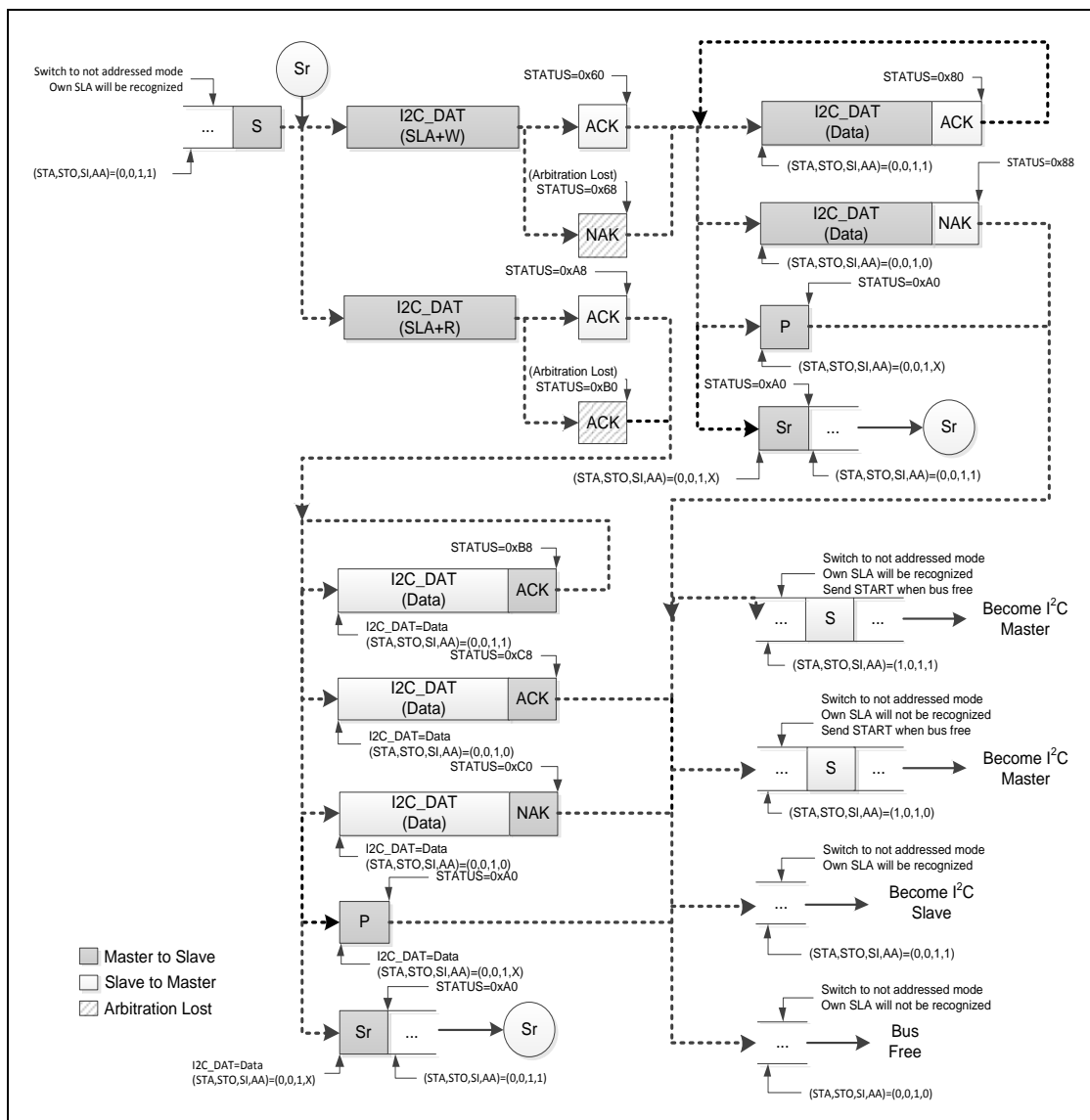
Figure 6.15-12 Save Mode Control Flow
