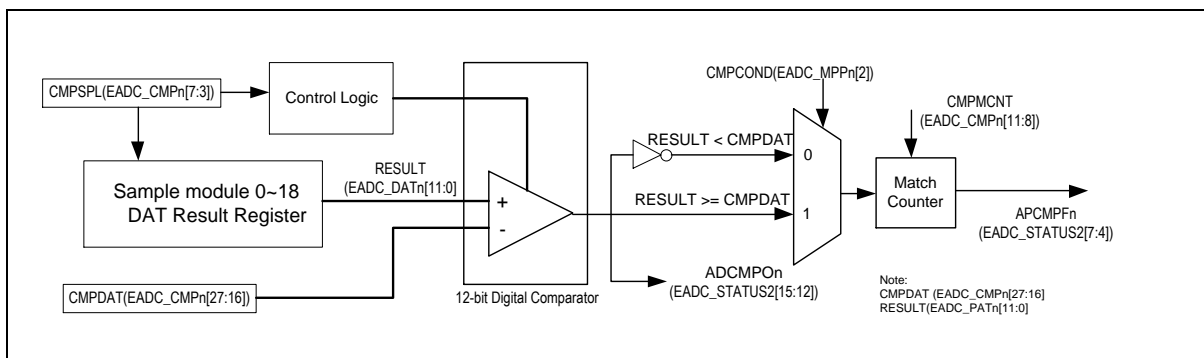
Figure 6.20-14 A/D Conversion Result Monitor Logics Diagram
