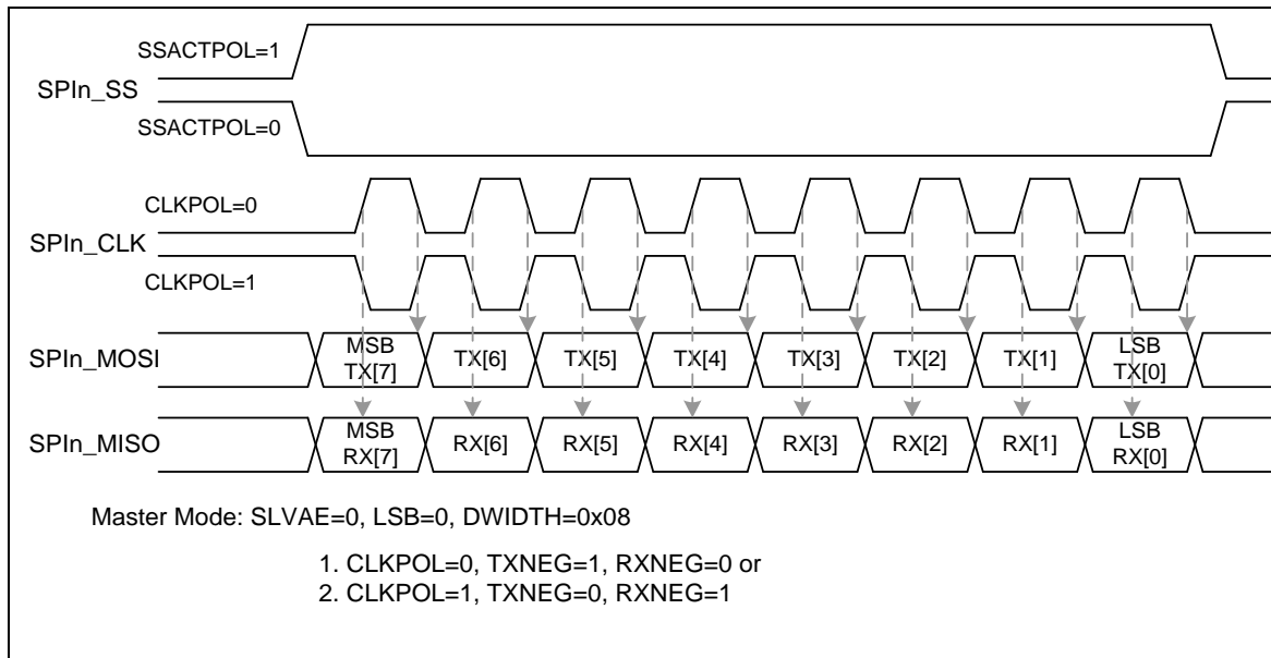
Figure 6.16-25 SPI Timing in Master Mode
