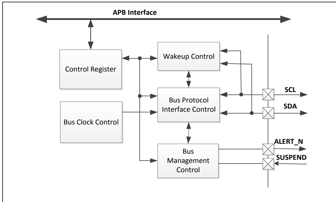
Figure 6.15-1 I²C Controller Block Diagram
