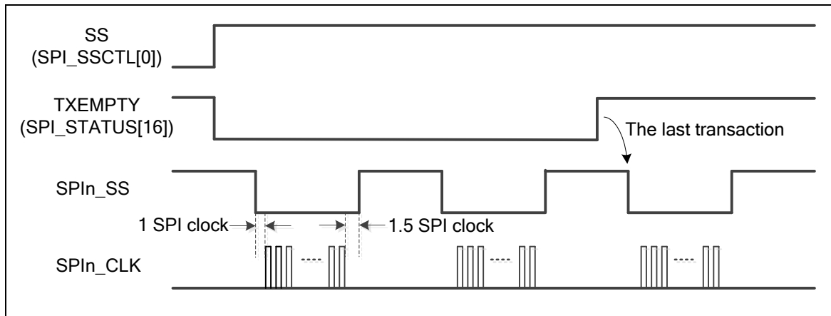
Figure 6.16-7 Automatic Slave Selection (SSACTPOL = 0, SPI_CYCLE > 0x2)
