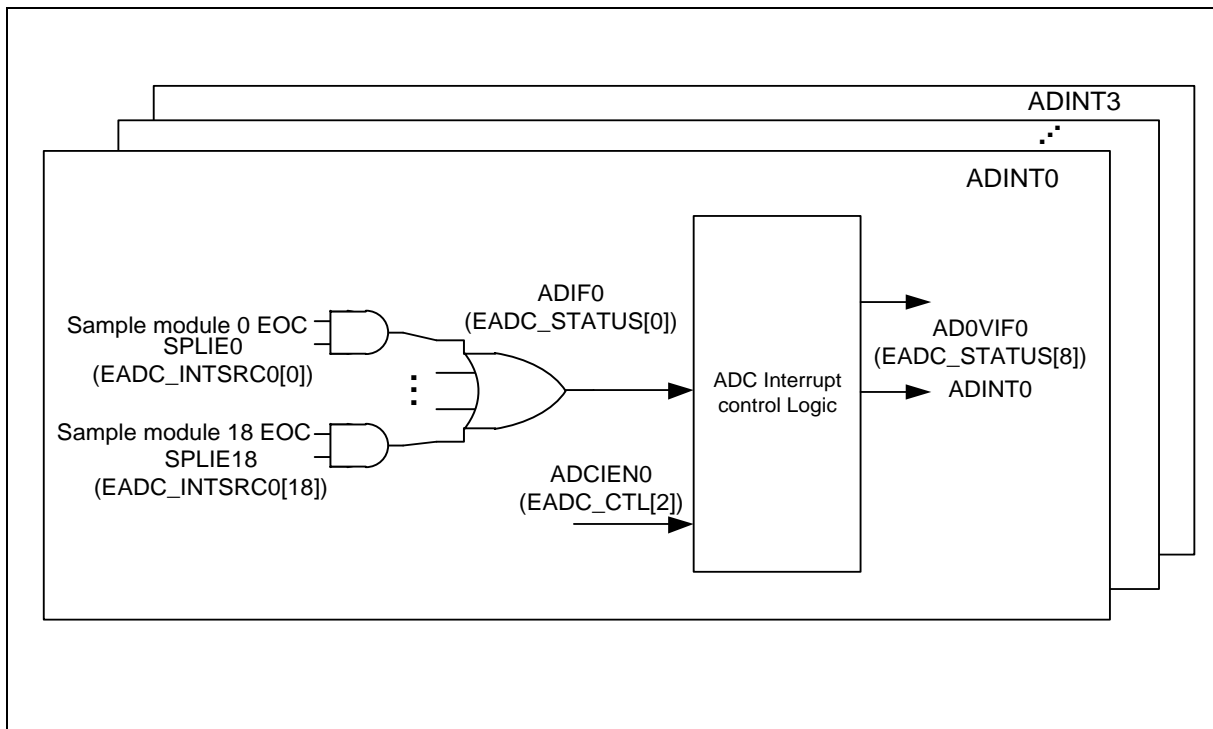
Figure 6.20-8 Specific Sample Module A/D EOC Signal for ADINT0~3 Interrupt
