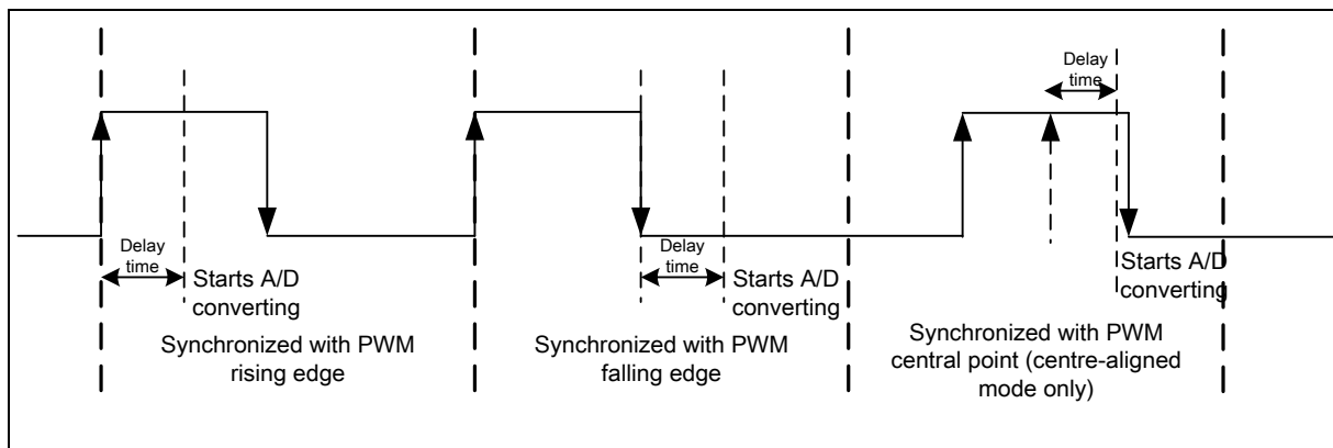
Figure 6.20-10 PWM-triggered ADC Start Conversion
