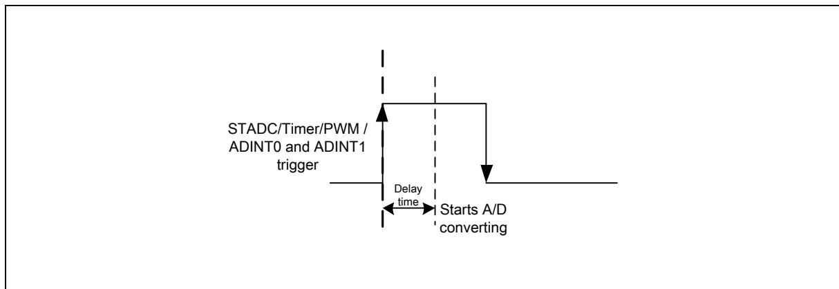
Figure 6.20-11 External triggered ADC Start Conversion
