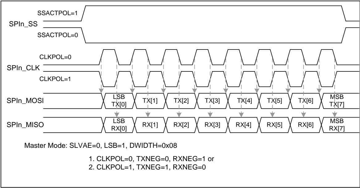
Figure 6.16-26 SPI Timing in Master Mode (Alternate Phase of SPIn_CLK)
