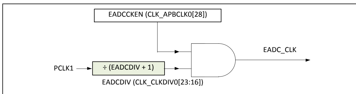
Figure 6.20-5 EADC Clock Control
