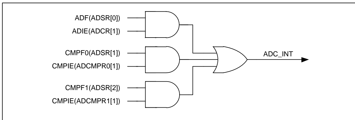
Figure 6.14-7 A/D Controller Interrupt
