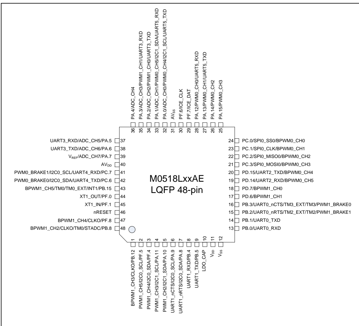
Figure 4.3-2 NuMicro® M0518LxxAE LQFP 48-pin Diagram
