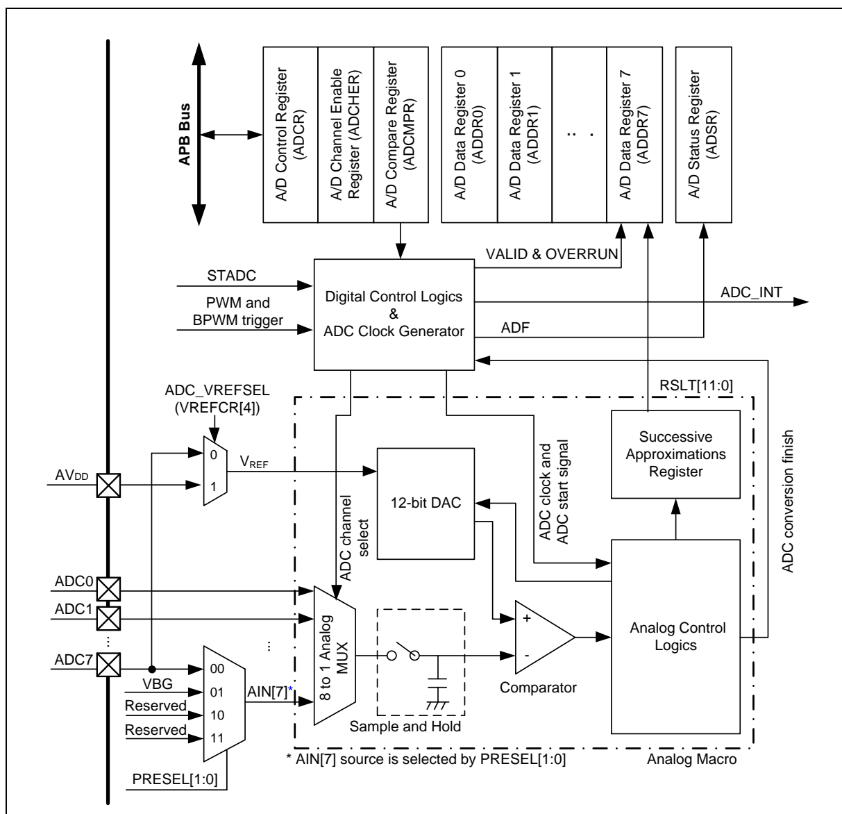
Figure 6.14-1 ADC Controller Block Diagram
