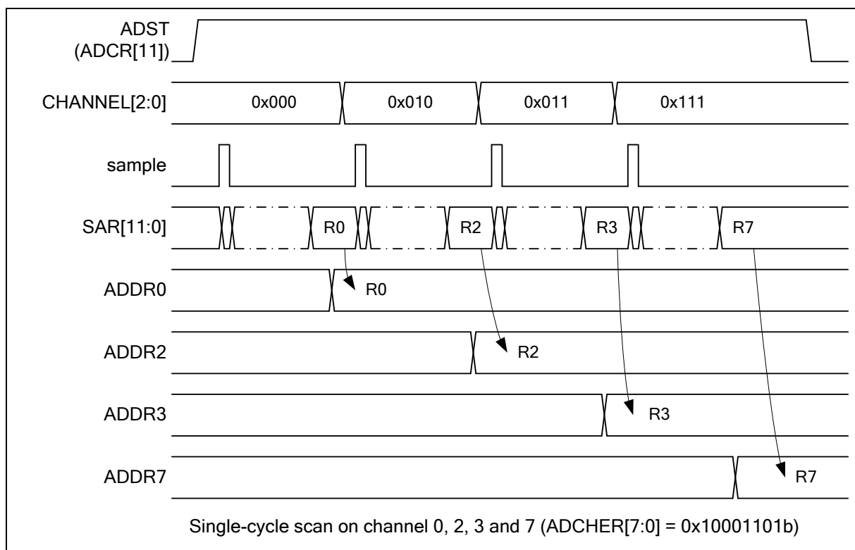
Figure 6.14-4 Single-Cycle Scan on Enabled Channels Timing Diagram
