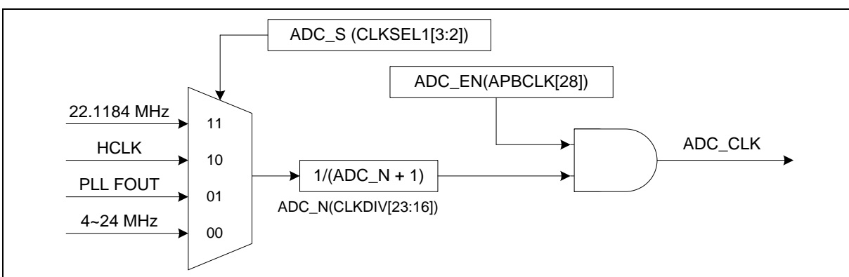
Figure 6.14-2 ADC Clock Control
