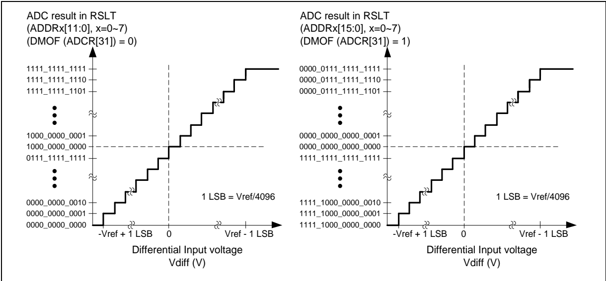
Figure 6.14-9 ADC Differential Input Conversion Voltage and Conversion Result Mapping
