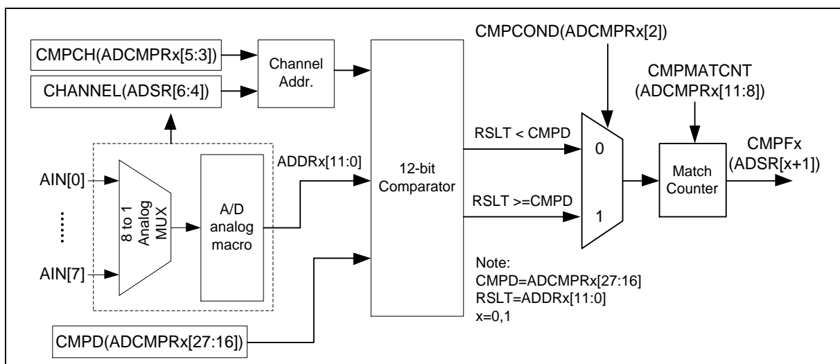
Figure 6.14-6 A/D Conversion Result Monitor Logics Diagram
