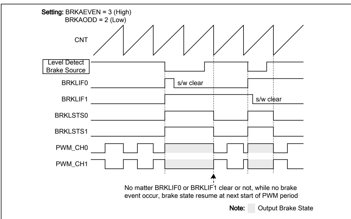
Figure 6.7-26 Level Detector Waveform for PWM_CH0 and PWM_CH1 Pair
