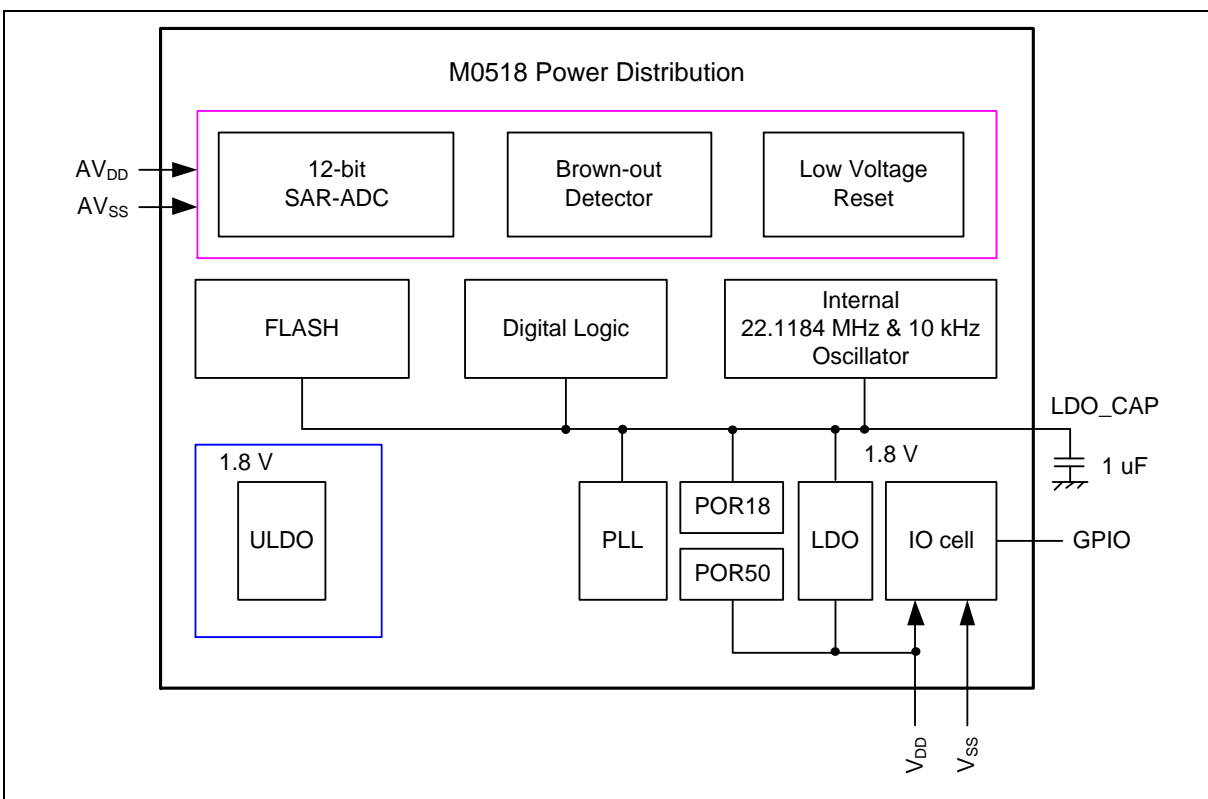
Figure 6.2-1 NuMicro® M0518 Series Power Distribution Diagram
