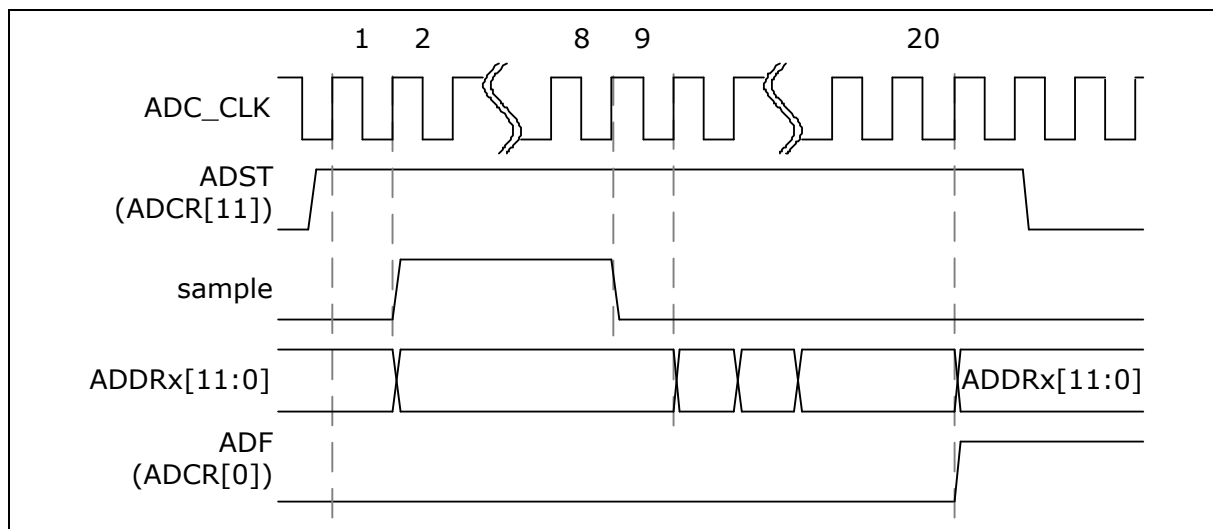
Figure 6.14-3 Single Mode Conversion Timing Diagram
