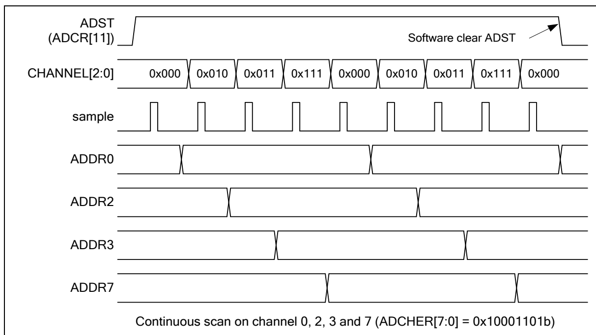
Figure 6.14-5 Continuous Scan on Enabled Channels Timing Diagram
