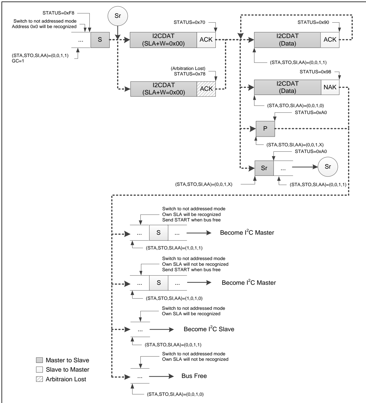
Figure 6.12-13 GC Mode
