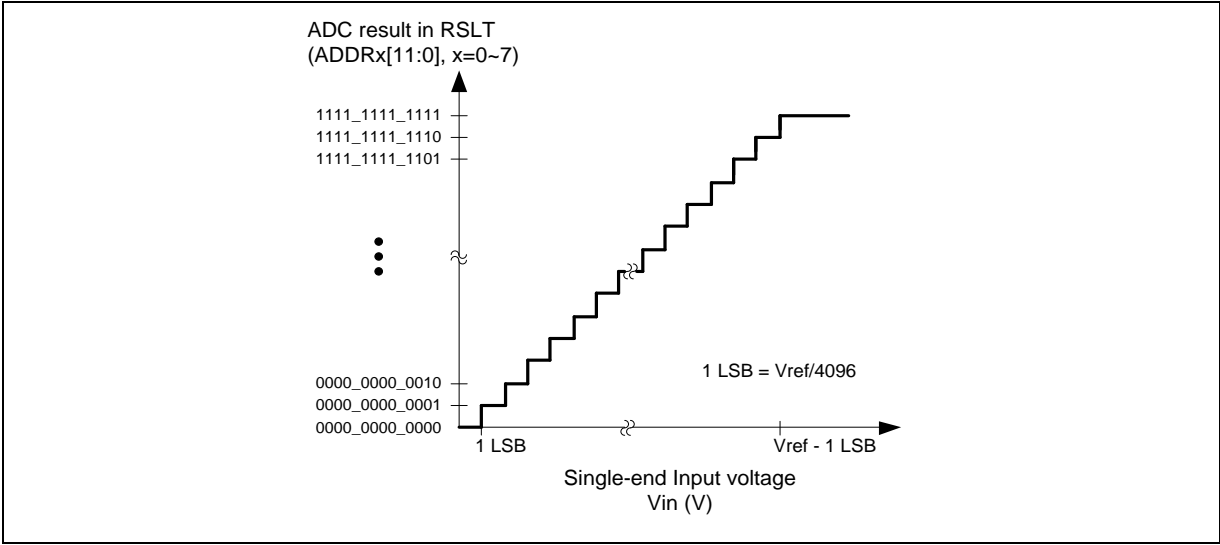
Figure 6.14-8 ADC Single-end Input Conversion Voltage and Conversion Result Mapping
