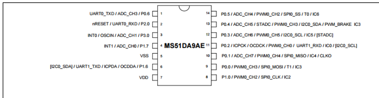
Figure 5-4 MS51 Series TSSOP-14-pin Diagram
