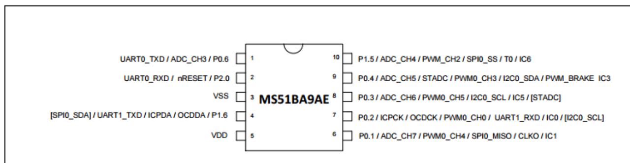
Figure 5-5 MS51 Series MSOP-14-pin Diagram
