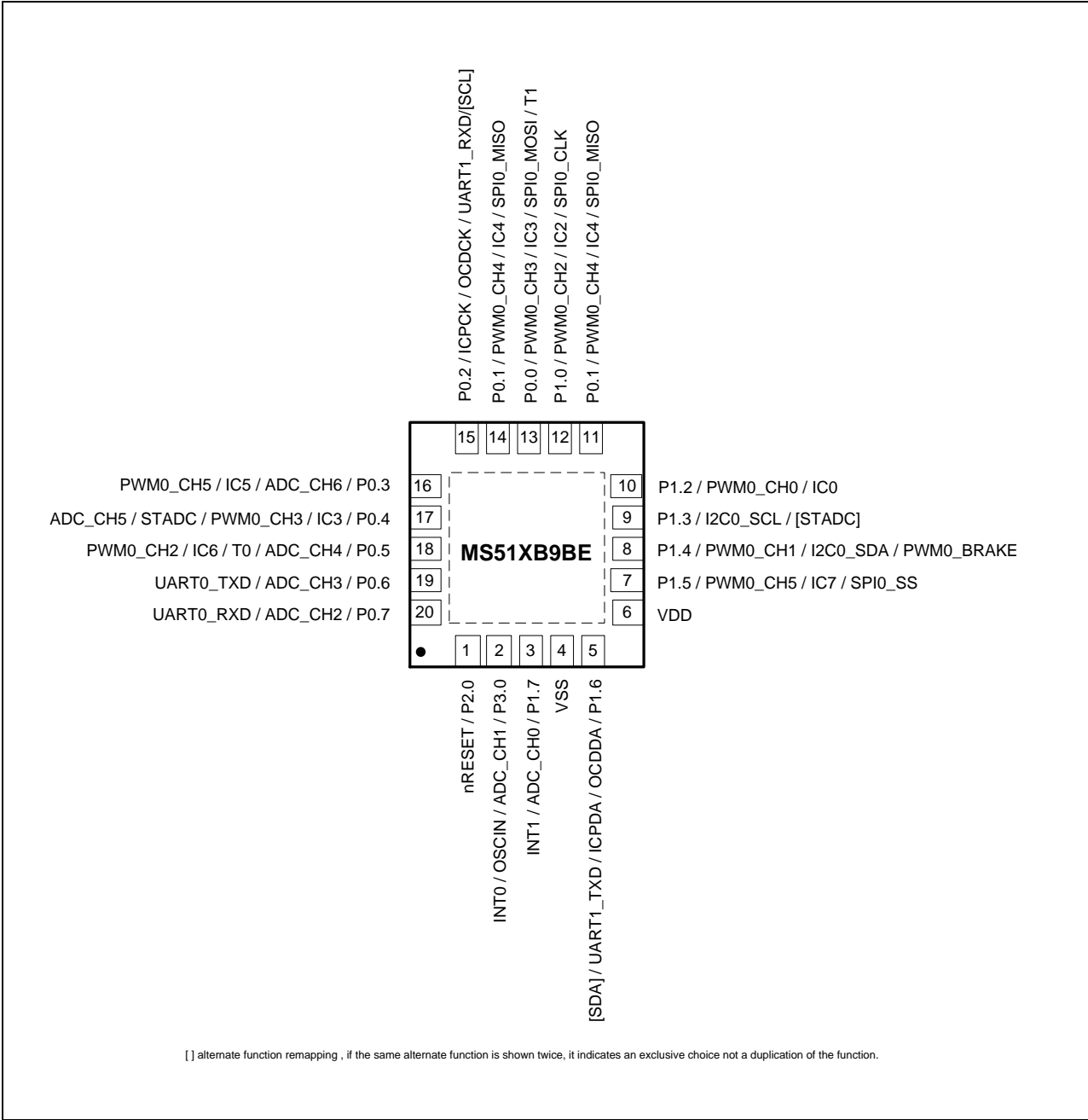
Figure 5-2 MS51 Series QFN-20-pin Diagram
