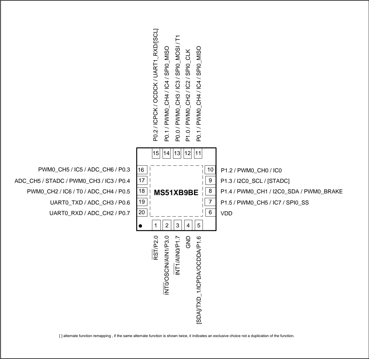
Figure 5-3 MS51 Series QFN-20-pin Diagram
