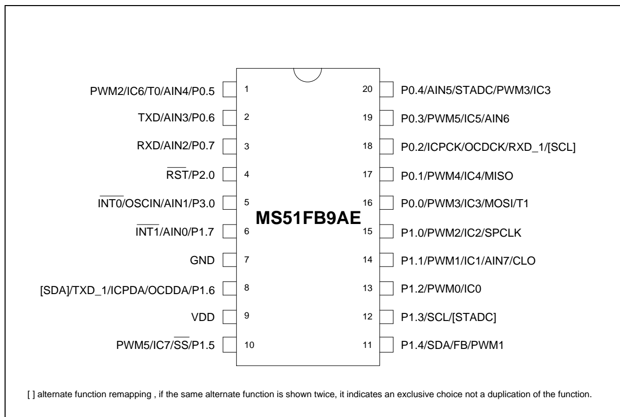
Figure 5-1 MS51 Series TSSOP-20 -pin Diagram
